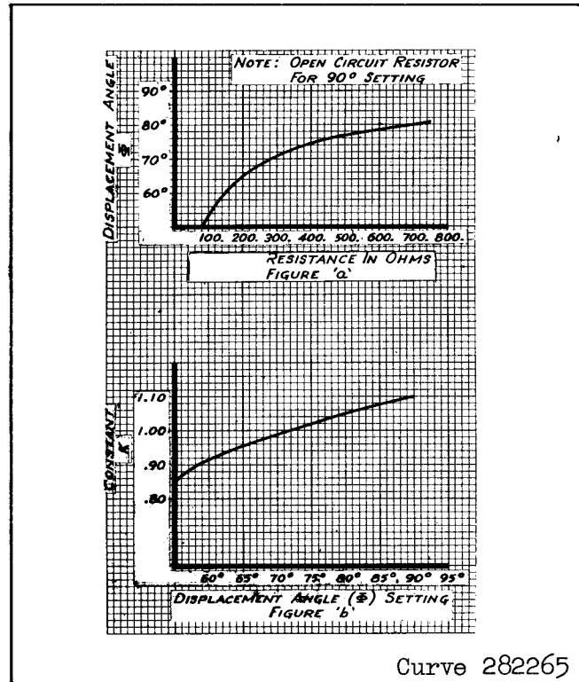
Fig. 5 Adjustment Curve for the Angular Displacement of the Operating Circle Center.
