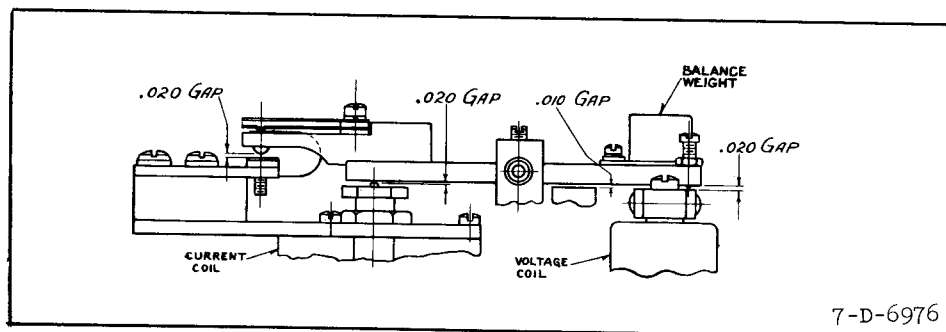
Fig. 1 Sectional View of the Impedance Units.
