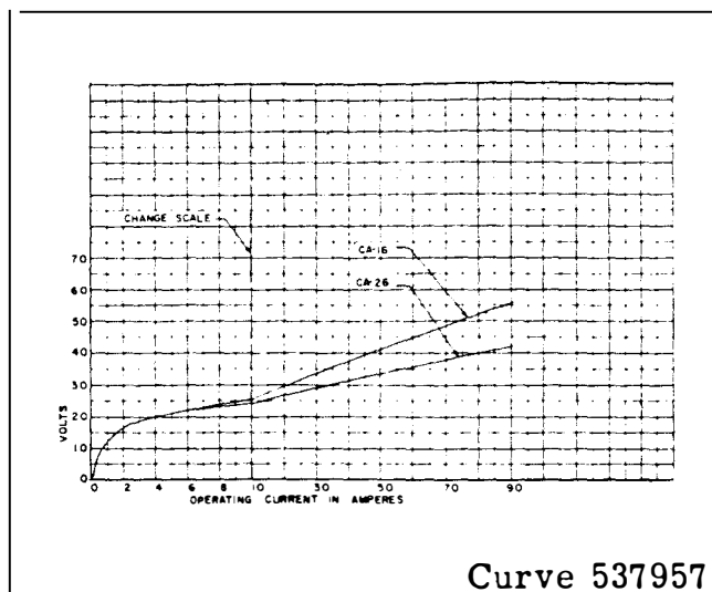
Fig. 7. Typical Burden Characteristic of the Operating Circuit of the CA-16 and CA-26 Differential Relays
