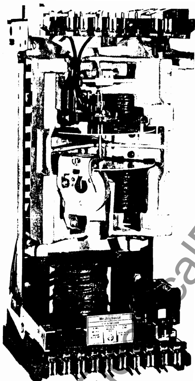
Fig. 1. Types CA-16 Relay (front view)
