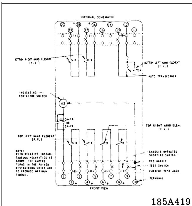
Fig. 3 Internal Schematic of the Type CA-16 Bus Relay or CA-26 Transformer Relay.
