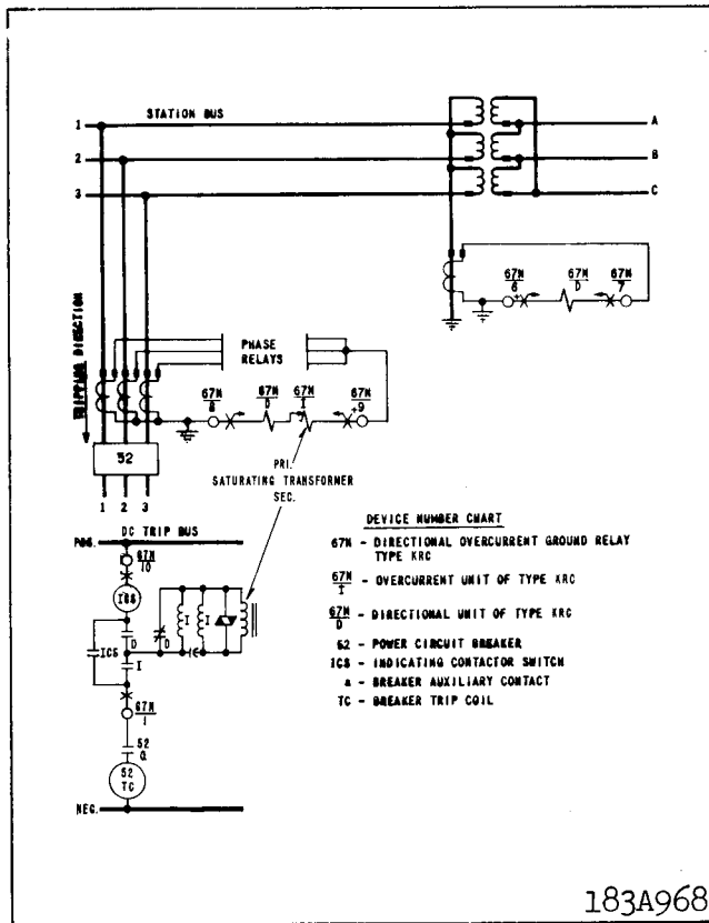
* Fig. 7. External Schematic of the Type KRC Relay.
