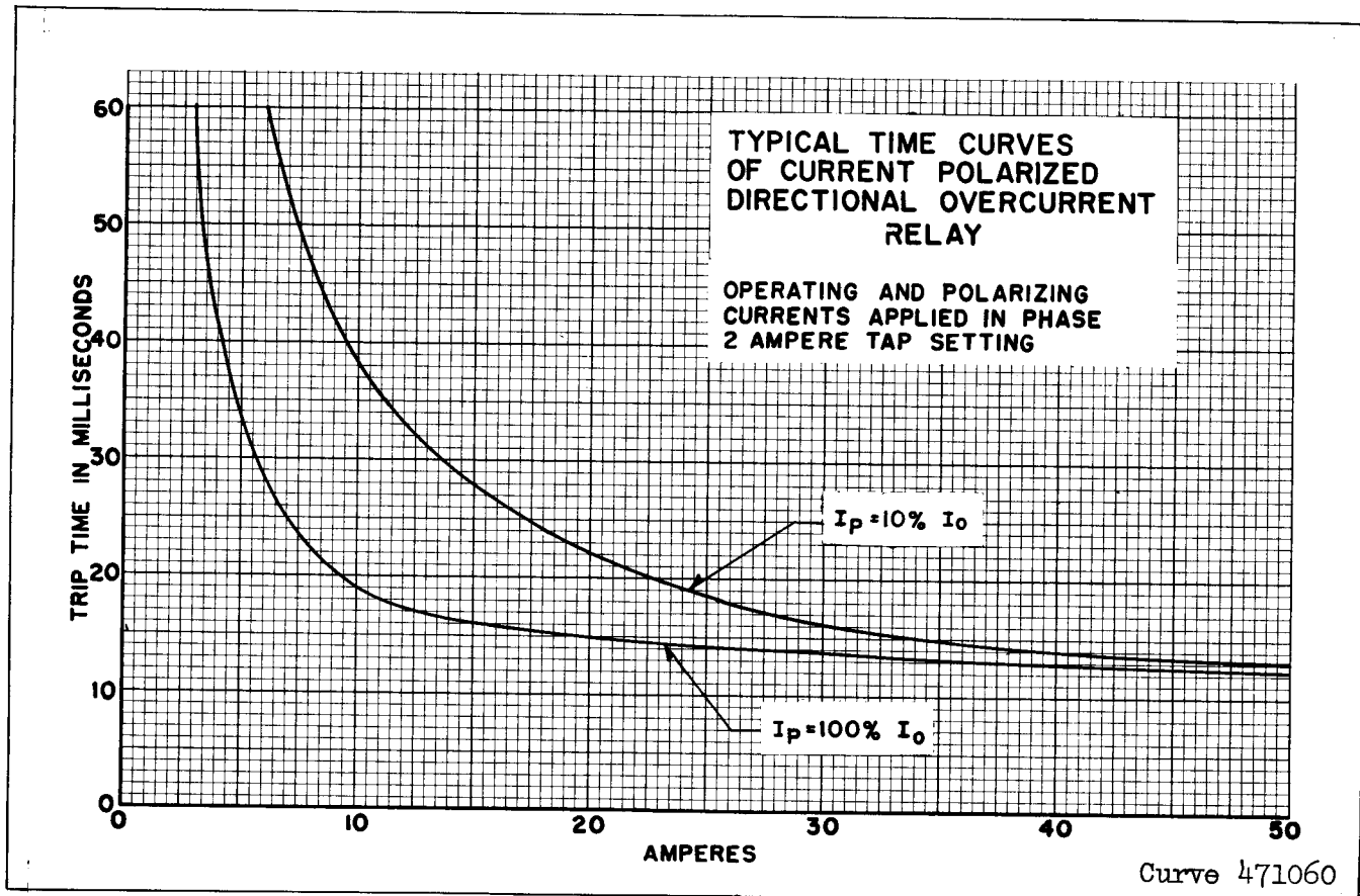
Fig. 6. Typical Operating Times for the Type KRC and KRD (When Current Polarized) Relays.
