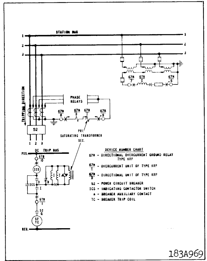
* Fig. 8. External Schematic of the Type KRP Relay.
