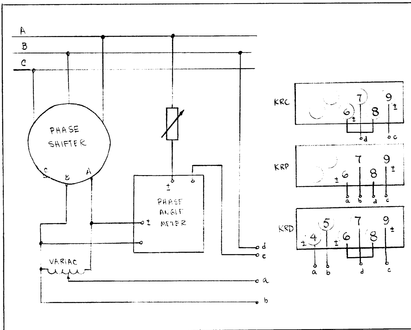
Figure 10. Test Connections
