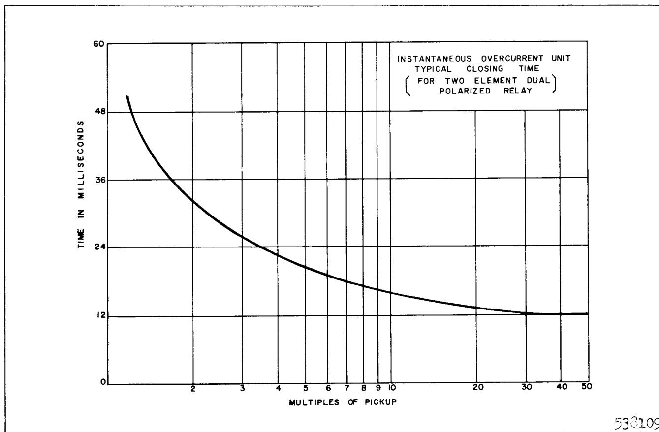
* Fig. 6. Typical Operating Times for the instantaneous Type KRC and KRD overcurrent unit (When Current Polarized) Relays.
