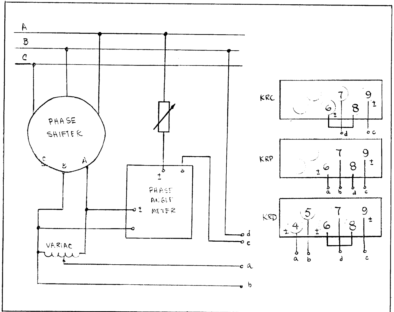
Figure 10. Test Connections
