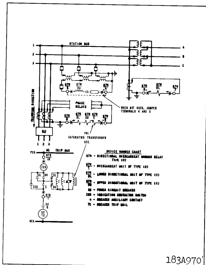
*Fig. 9. External Schematic of the Type KRD Relay.
