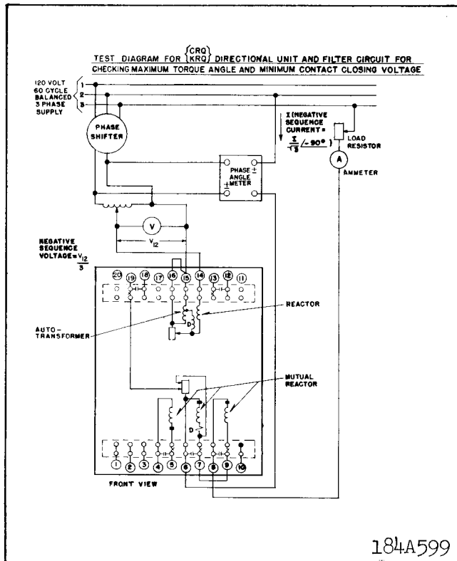
Fig. 12. Test Diagram for Checking Maximum Torque Angle and Minimum Voltage for Contact Closure of the Directional Unit.
