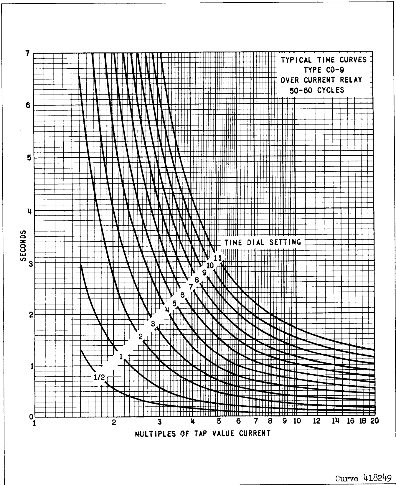
Fig. 20. Typical Time Curve of the Time-Overcurrent Unit of the Very Inverse (9) Relay.
