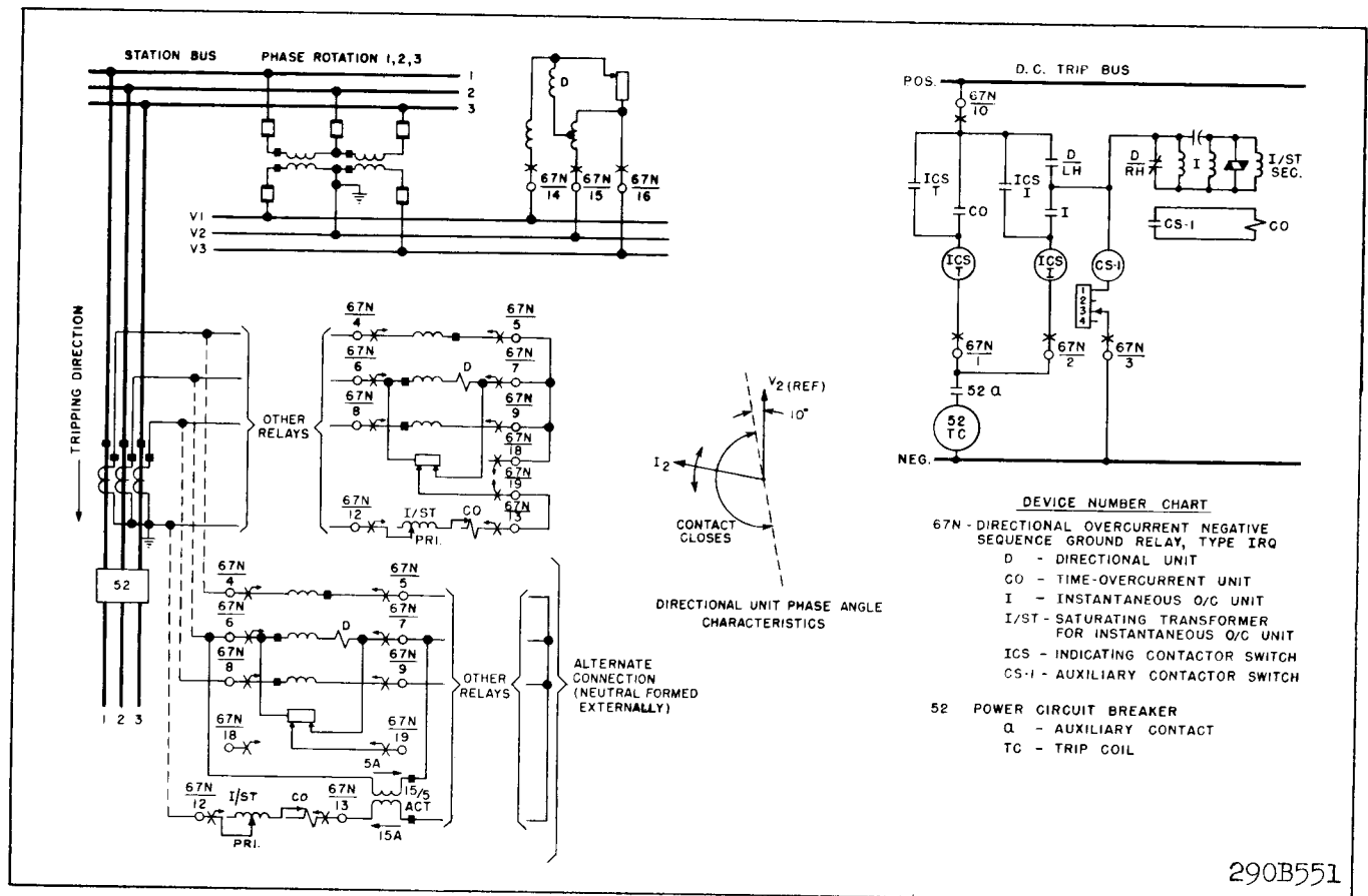
Fig. 11. External Schematic of IRQ Relay.
