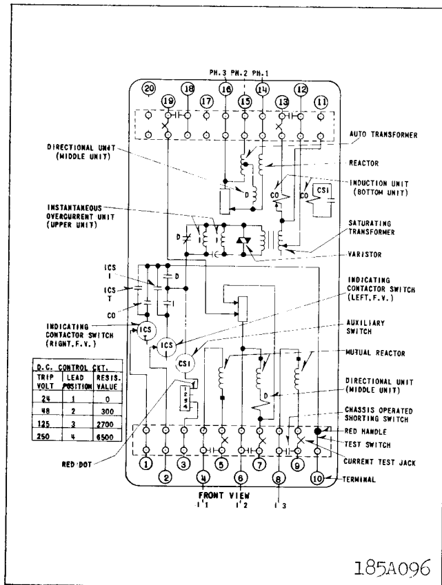
Fig. 4. Internal Schematic of the IRQ Relay.
