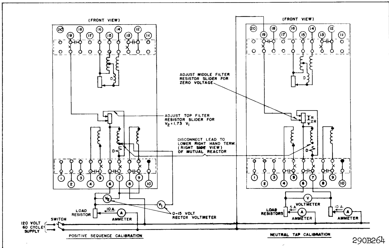
Fig. 8. Test Diagram for Calibration of the Negative Sequence Current Filter in the IRQ Relay.
