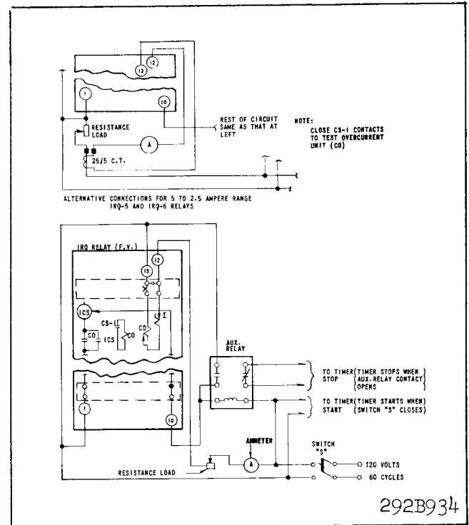
Fig. 7. Diagram of Test Connections for the Circuit Closing Time Overcurrent Unit of the IRQ Relay.
