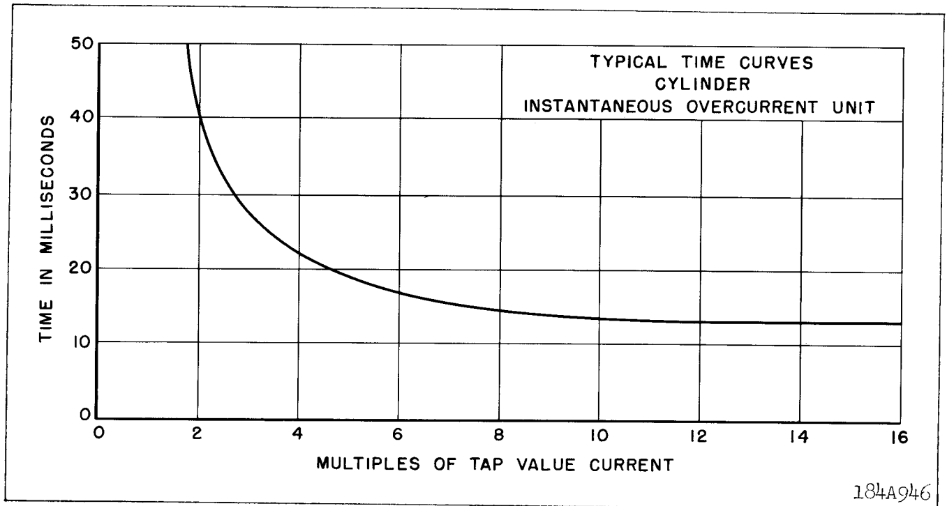
Fig. 13. Typical Time Curve of the Instantaneous Overcurrent Unit.
