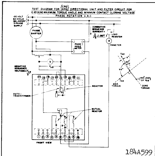
Fig. 12. Test Diagram for Checking Maximum Torque Angle and Minimum Voltage for Contact Closure of the Directional Unit.
