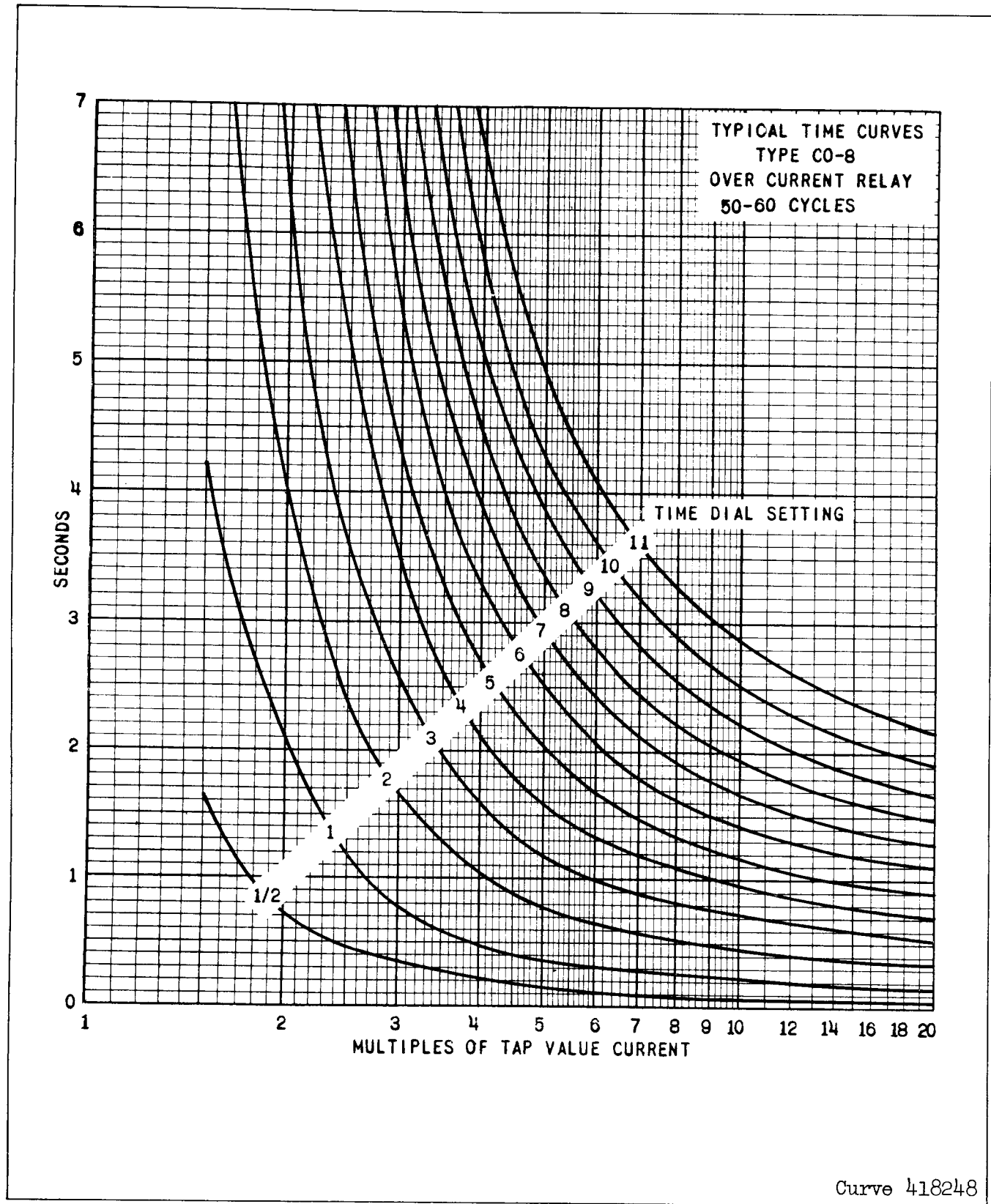
Fig. 19. Typical Time Curve of the Time-Overcurrent Unit of the Inverse (8) Relay.
