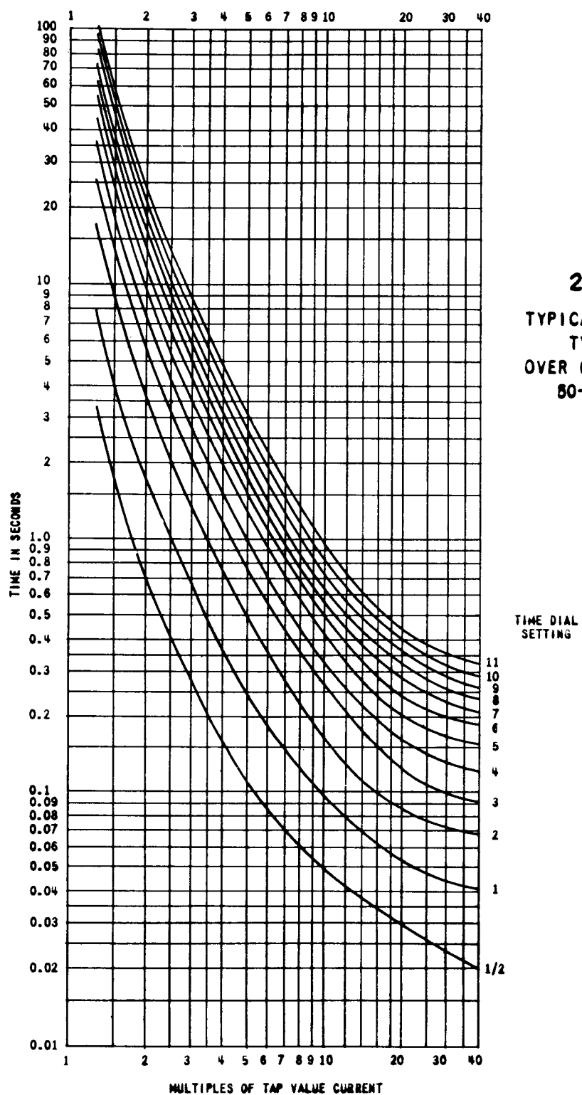
Fig. 21. Typical Time Curve of the Time-Overcurrent Unit of the Extremely Inverse (11) Relay.
