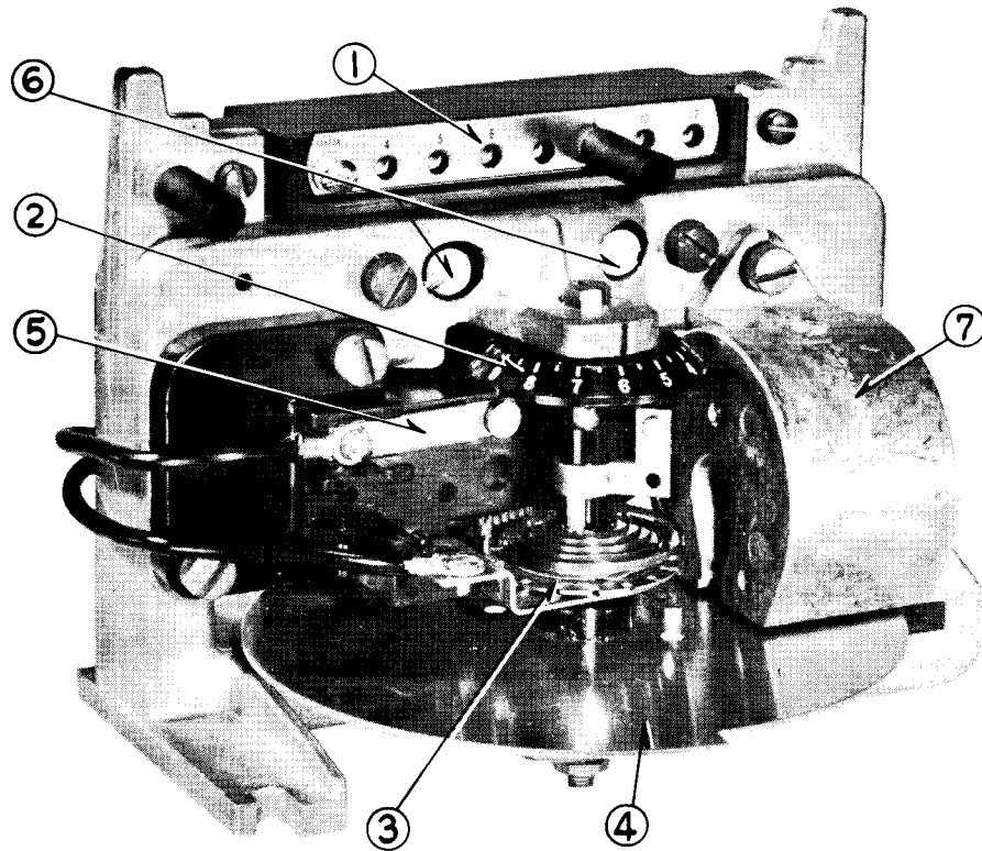
Fig. 3. Time Overcurrent Unit (Front View). 1-Tap Block, 2-Time Dial, 3-Control Spring Assembly, 4-Disc, 5-Stationary Contacts Assembly, 6-Magnetic Plugs, 7-Permanent Magnet
