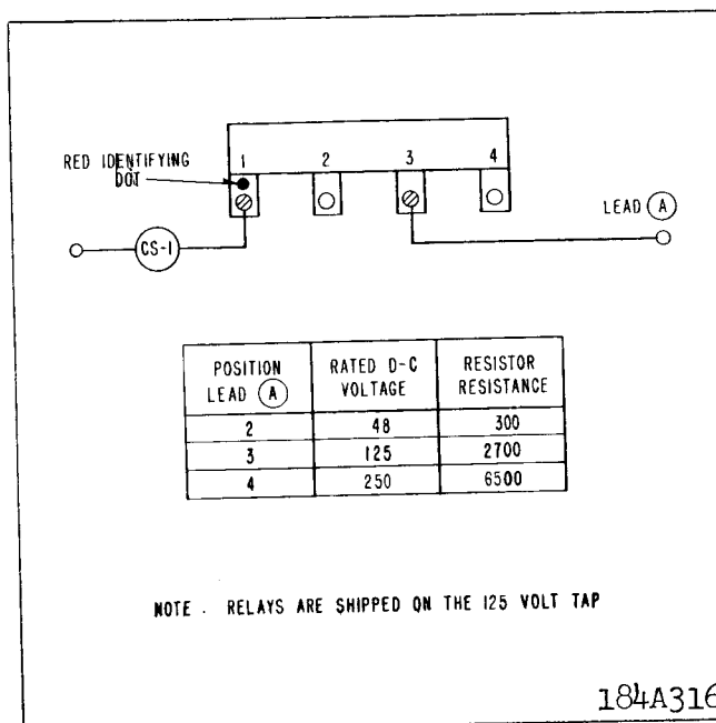
Fig. 14. Selection of Proper Voltage Tap for Auxiliary Switch (CS-1) Operation.
