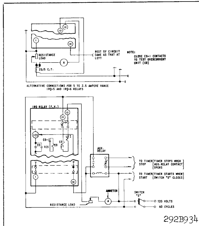
Fig. 7. Diagram of Test Connections for the Circuit Closing Time Overcurrent Unit of the IRQ Relay.
