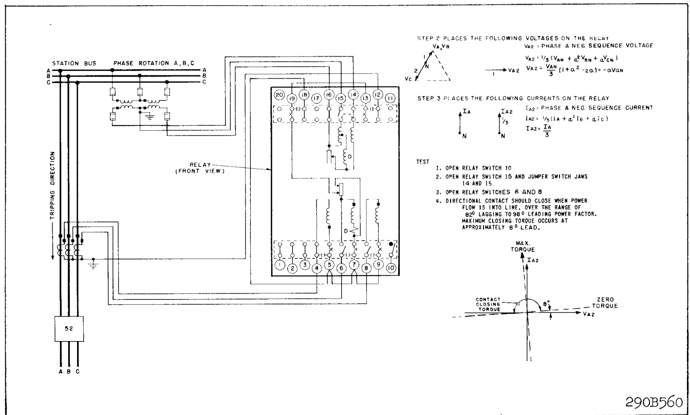
* Fig. 9. In Service Test Procedure for Verifying Proper External Connections Where CT Neutral is Formed Within the Relay.
