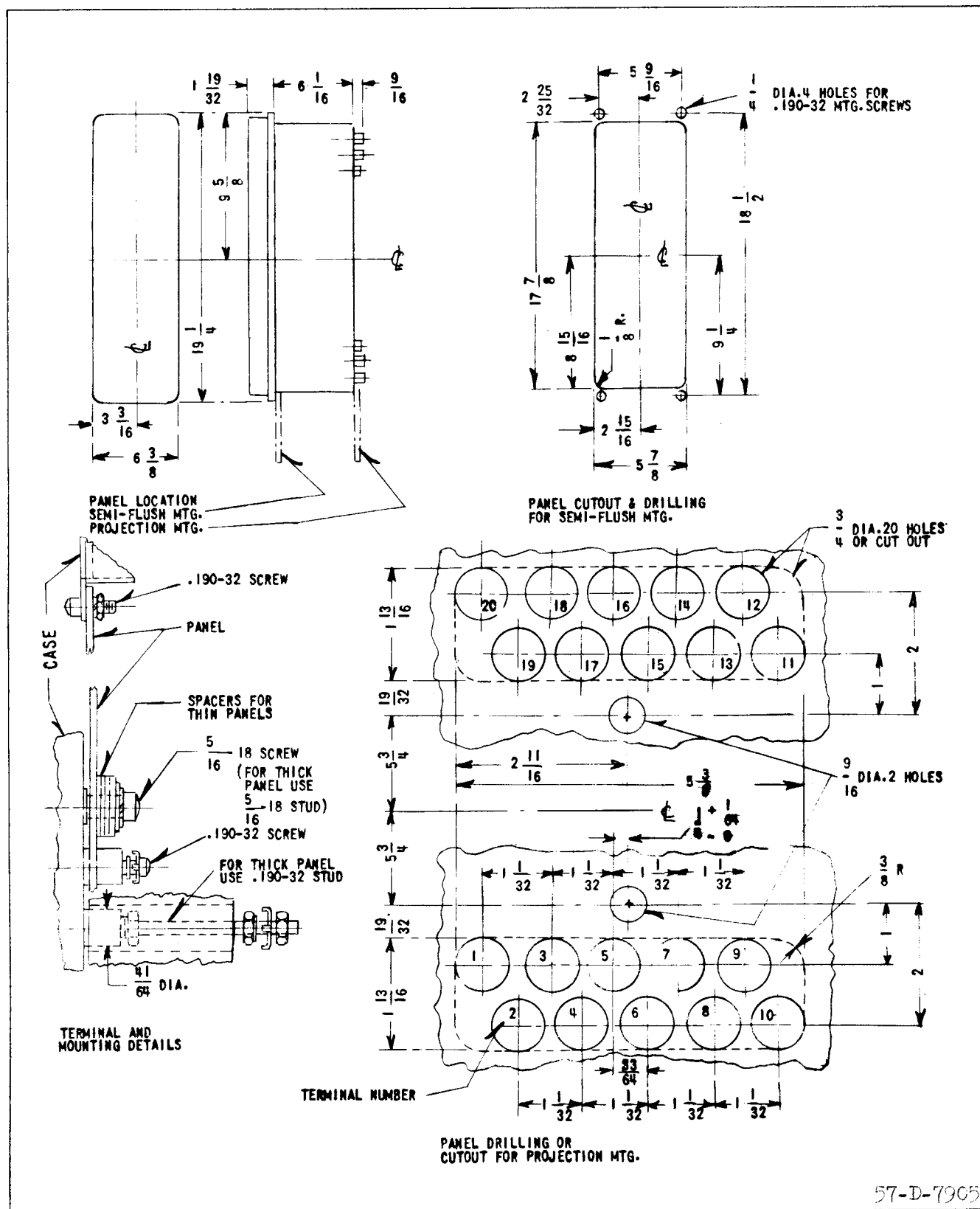
Fig. 22. Outline and Drilling Plan for the Type IRQ Relay in the FT42 Case.
