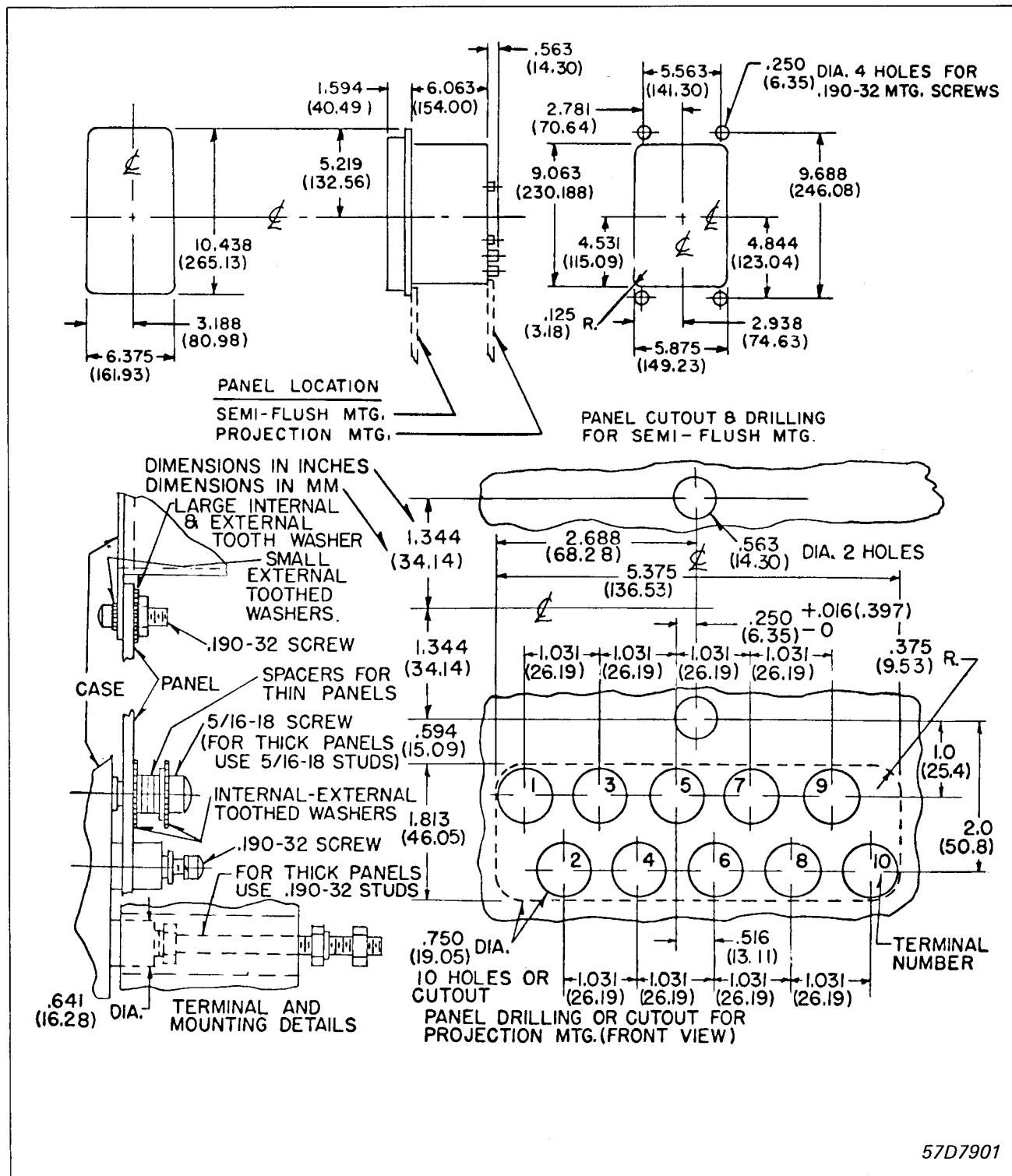
Fig. 6. Outline and Drilling for the Type CO-4 Relay in Type FT-21 Case.
