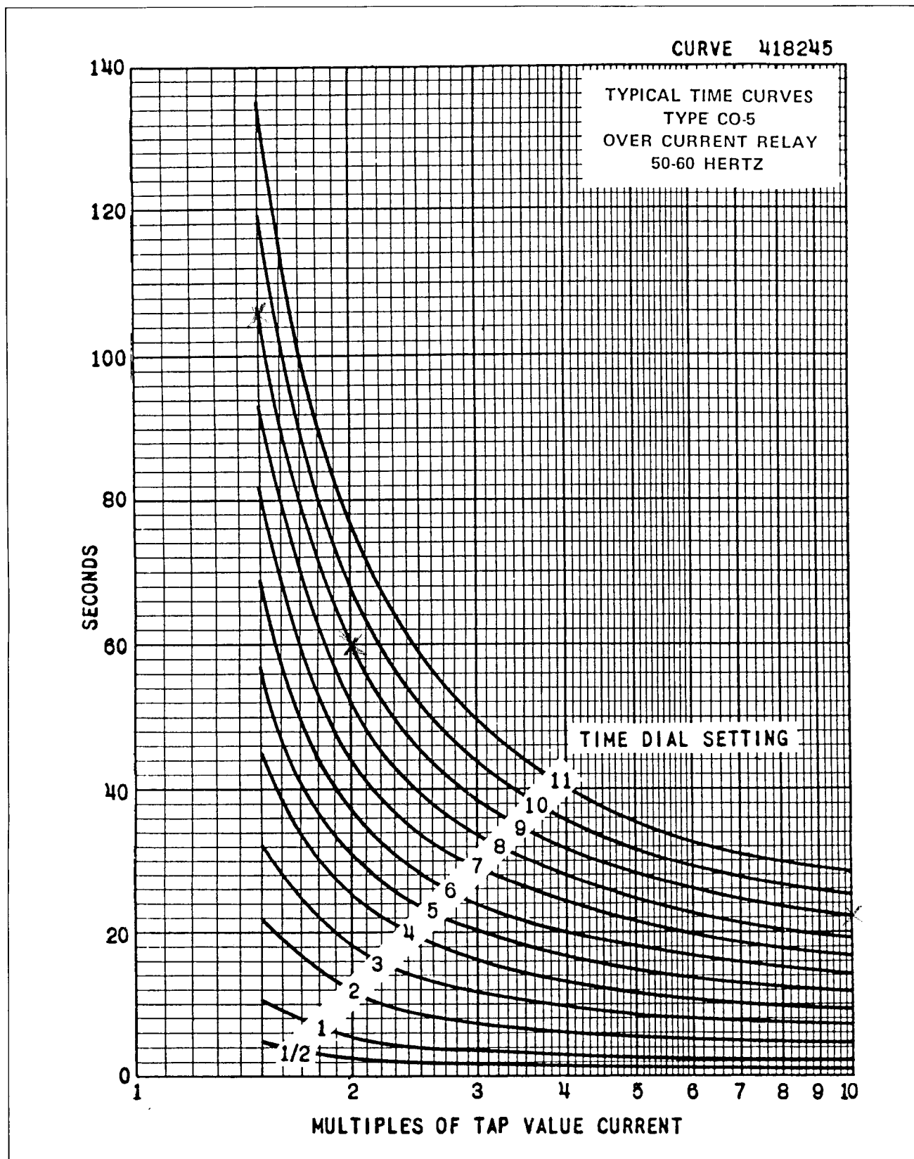
Fig. 2. Typical Time Curves for the Overcurrent Unit.
