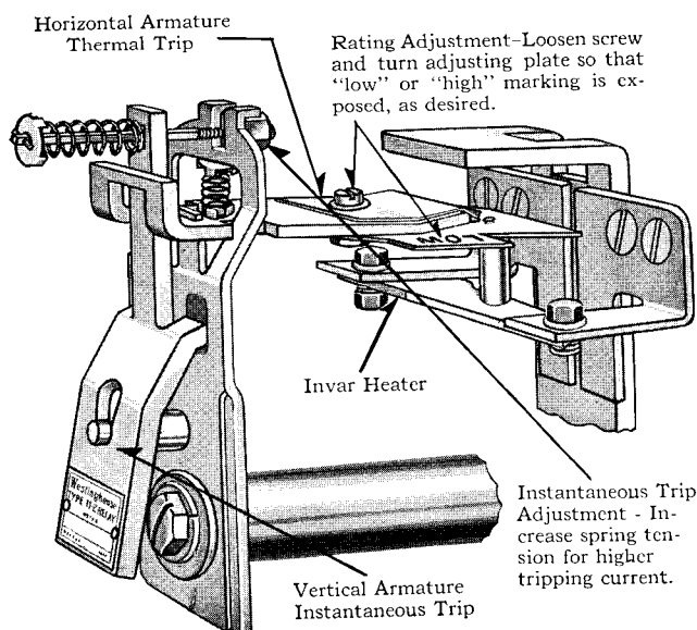
FIG. 2—INSTANTANEOUS TRIP ADJUSTMENT
