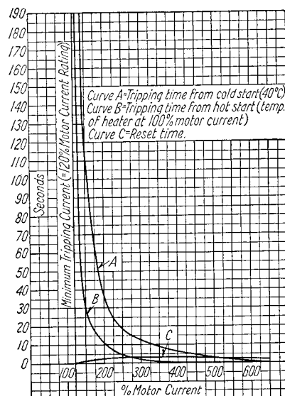
FIG. 1—RATING CHARACTERISTICS
