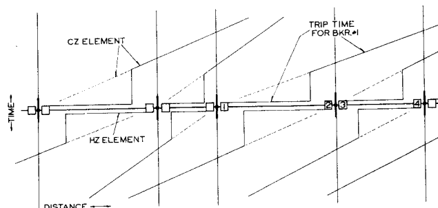
Figure 1 Typical Time-Distance Characteristic of the Type HCZ Relay.
