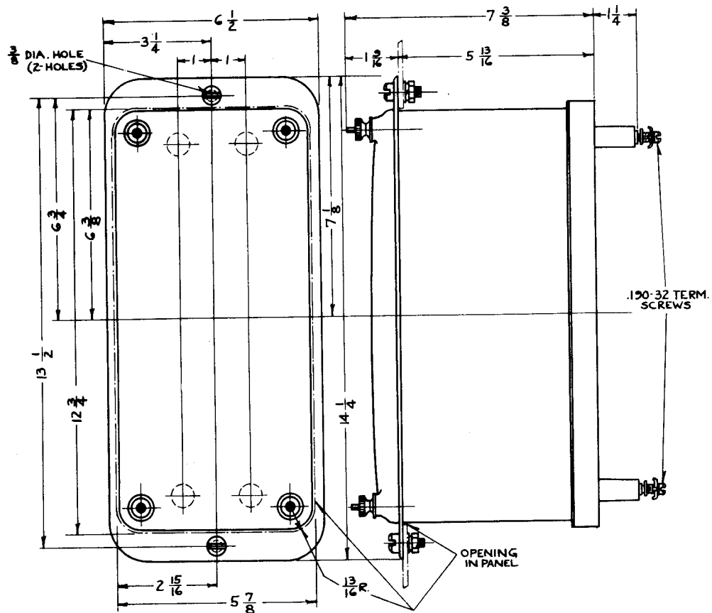
Figure 20 Outline and Drilling Plan for the Standard Flush Type Case.
