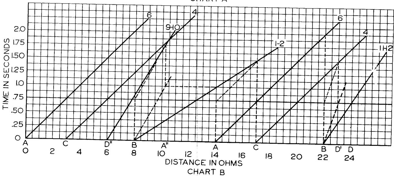
Figure 9 Construction of Time-Distance Chart for the System Shown.
