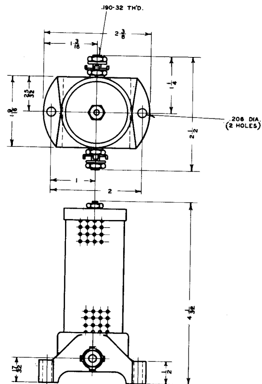
Figure 18 Outline and Drilling Plan for the External Control Circuit Resistor for the 250 volt d-c. Relays.
