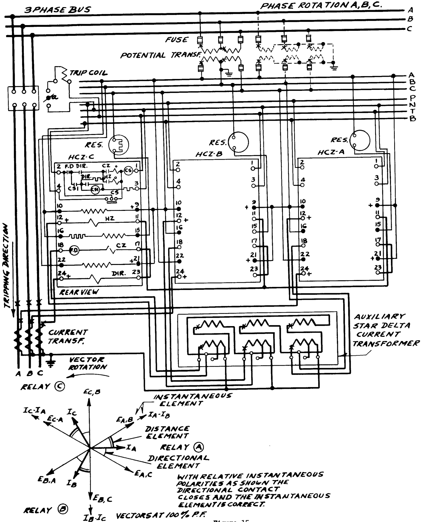
Figure 15 External Connections Using Star Current for the Directional and Distance Elements and Delta Current for the Instantaneous Element.
