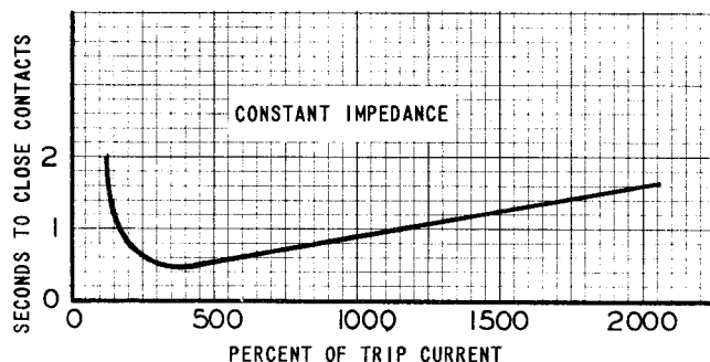
Figure 12 Typical Time-Ampere Curve of the Distance (CZ) Element for a Constant Given Distance.
