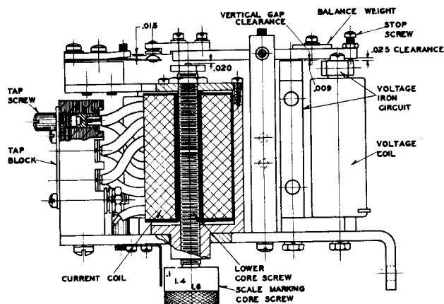
Figure 3 Sectional View of the Instantaneous (HZ) Element.
