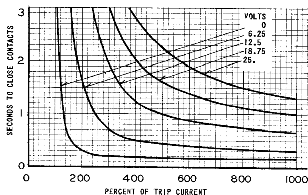
Figure 11 Typical Time-Ampere Curves of the Distance (CZ) Element (Enlarged)
