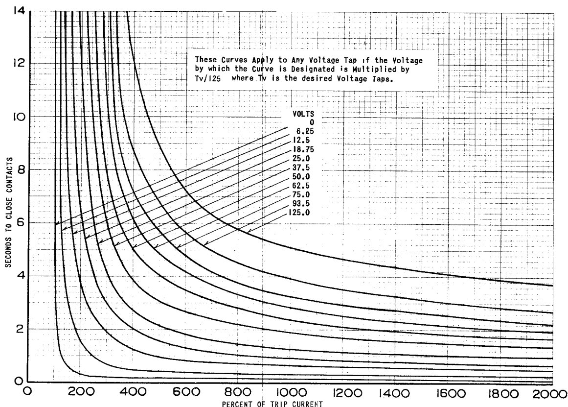
Figure 10 Typical Time-Ampere Curves of the Distance (CZ) Element
