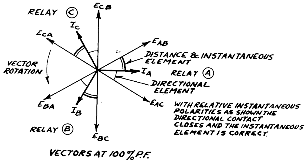
Figure 16 External Connections Using Star Current for All Elements
