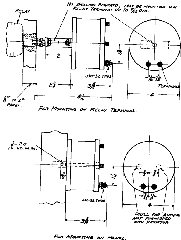
Figure 17 Outline and Drilling Plan for the Tapped a-c. Voltage Resistor for the Distance (CZ) Element.
