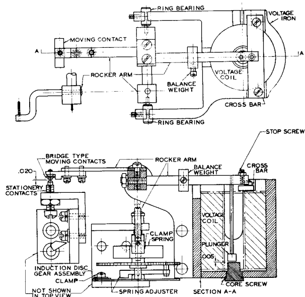
Figure 4 Sectional View of the Distance (CZ) Element
