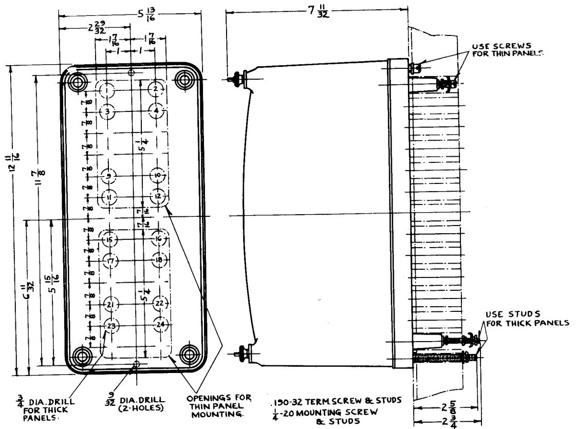
Figure 19 Outline and Drilling Plan for the Standard Projection Type Case
