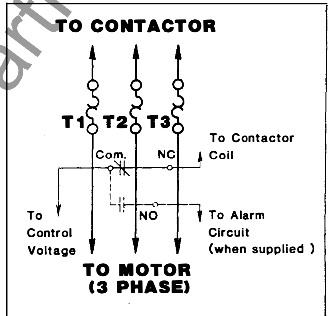
Fig. 6 Connection Diagram
