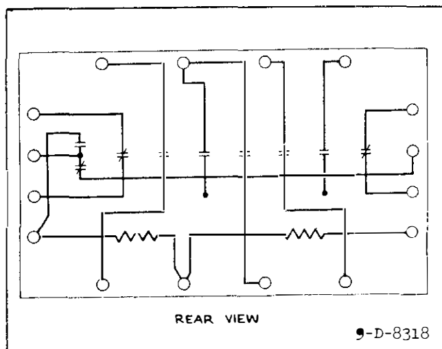
Fig. 1—Internal Schematic of S#1274697 Type SG Relay in the Projection Case.
