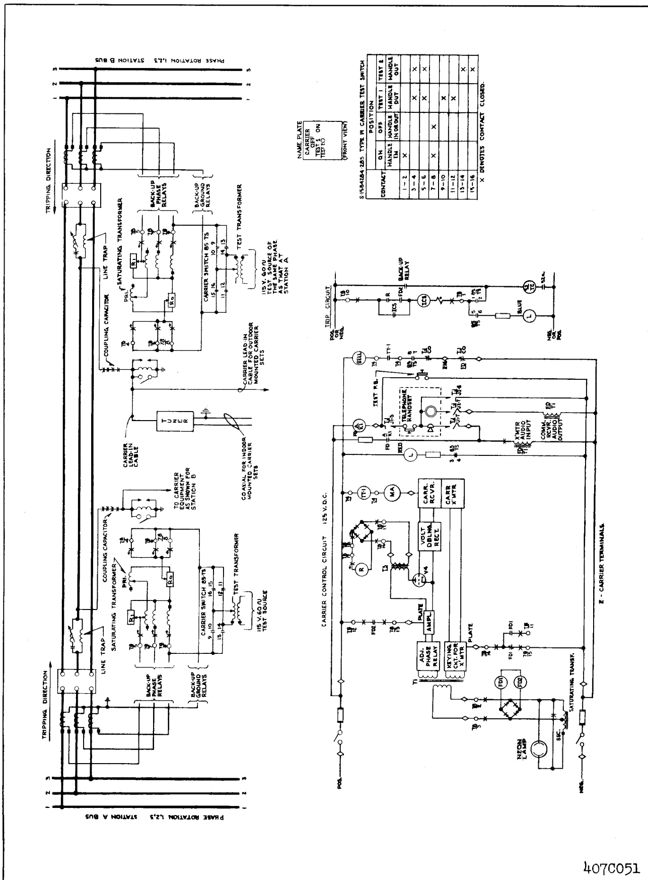
Fig. 3. External Schematic of the HKB Relay and Test Facilities, with TT-1 Alarm Relay.
