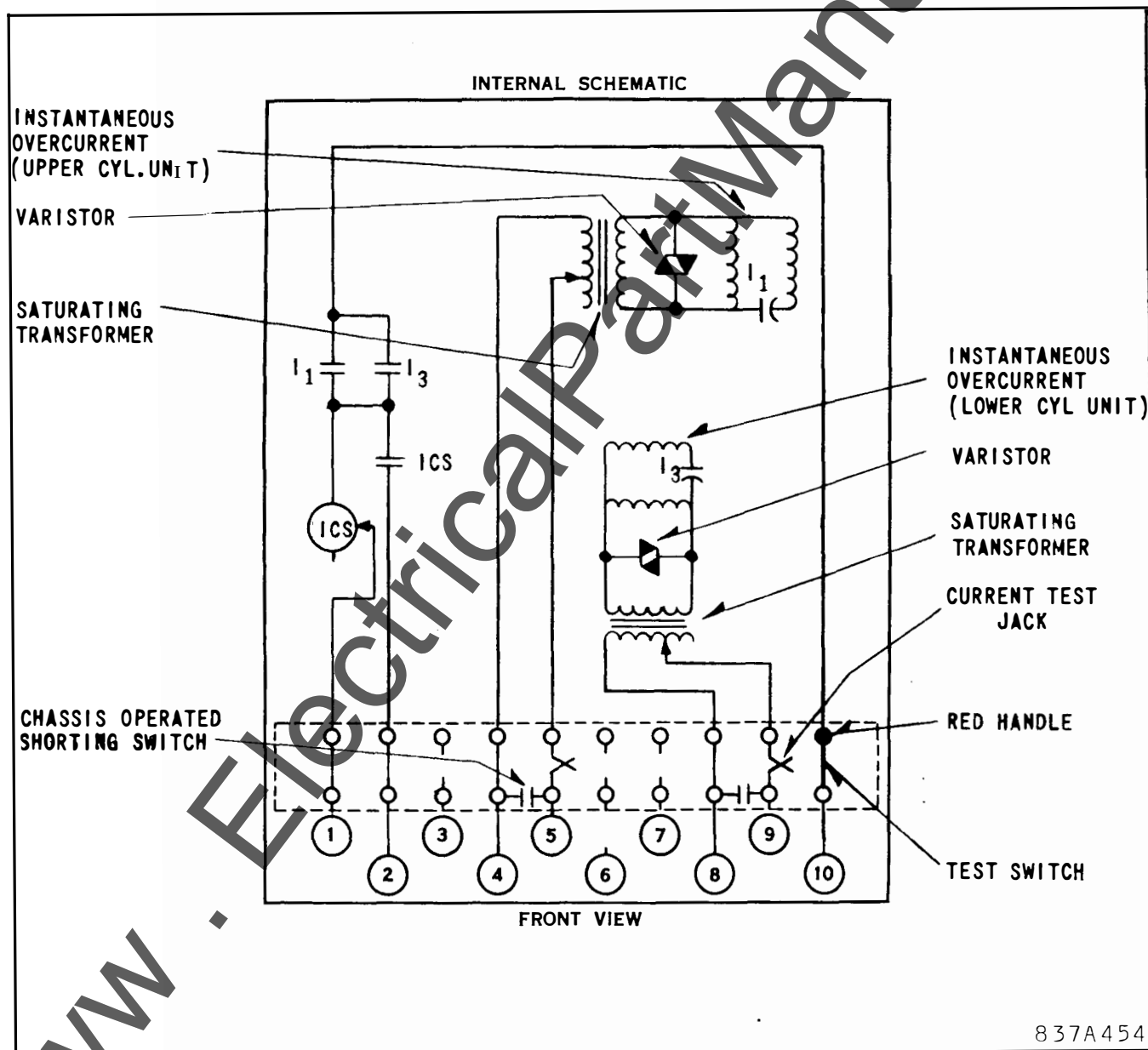
Fig. 1 Internal Schematic
