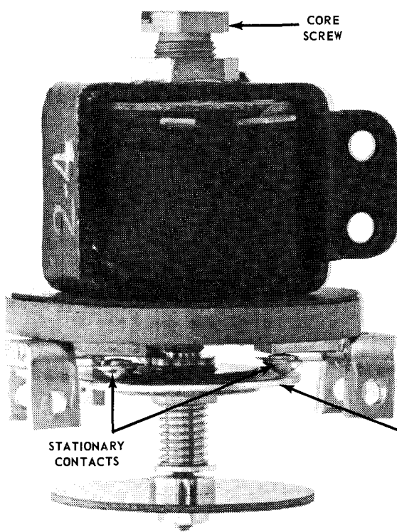
★ Fig. 1. High Drop-Out Instantaneous Trip Unit (ITH).
