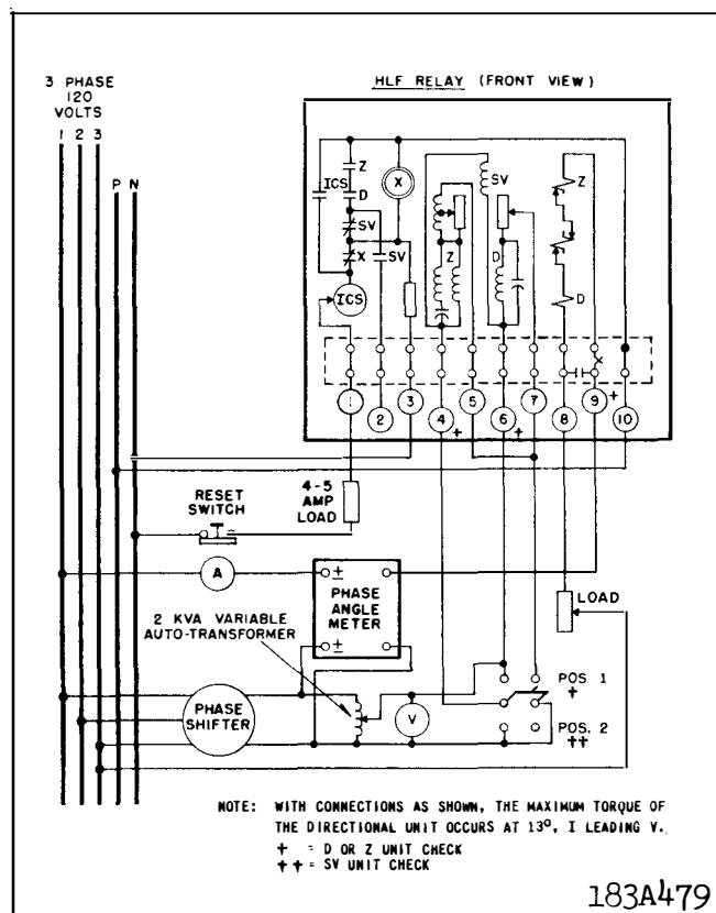
* Fig. 8. Diagram of Test Connections for HLF Relay.
