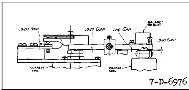
Fig. 1. Sectional View of Impedance Unit Beam.
