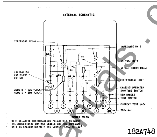
Fig. 2. Internal Schematic of the Type HLF Relay in the FT31 Case.
