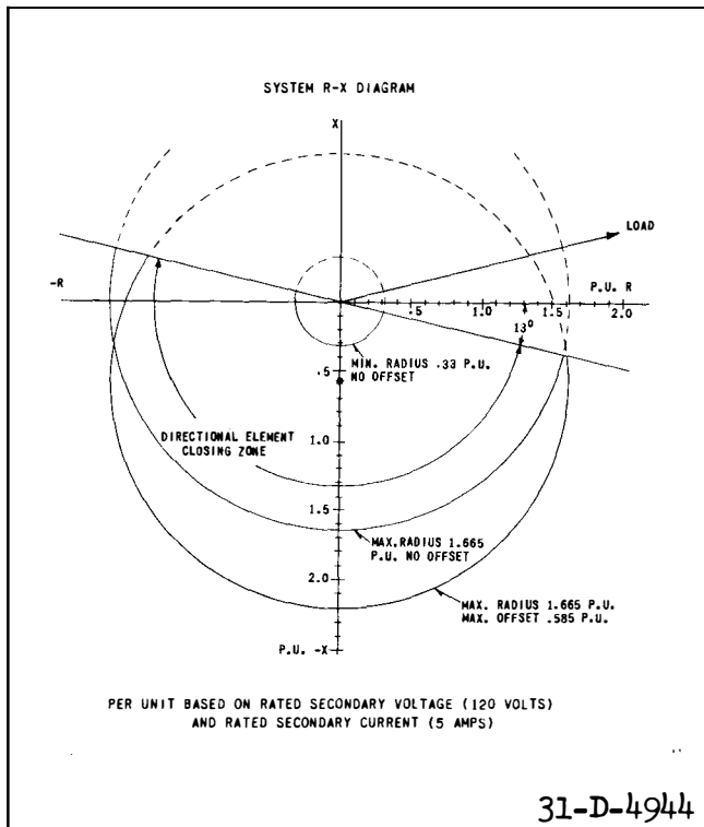
Fig. 4. Impedance and Directional Unit Characteristics Plotted on System R-X diagram - Per Unit Impedance .
