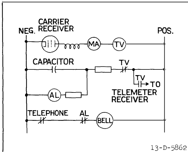
Fig. 4—Time Delay Circuit for the Carrier Alarm when using the Carrier Channel for Telemetering or Supervisory.
