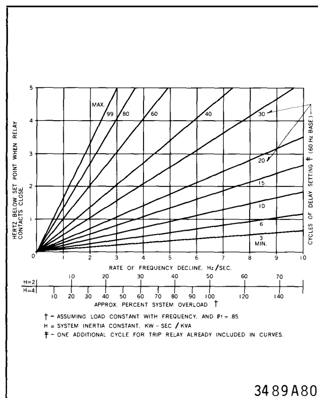
Fig. 13 SDF-1 Relay Tripping Delay Under Declining Frequency Conditions
