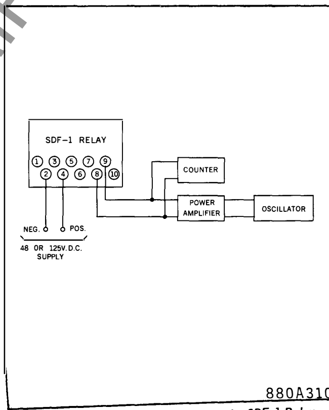
Fig. 10 Diagram of Test Connections for SDF-1 Relay
