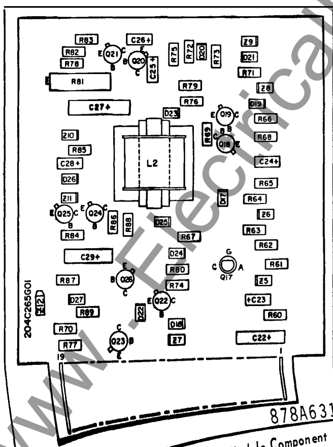
Fig. 7 Twelve Bit Binary Counter Printed Circuit Module Component Location
