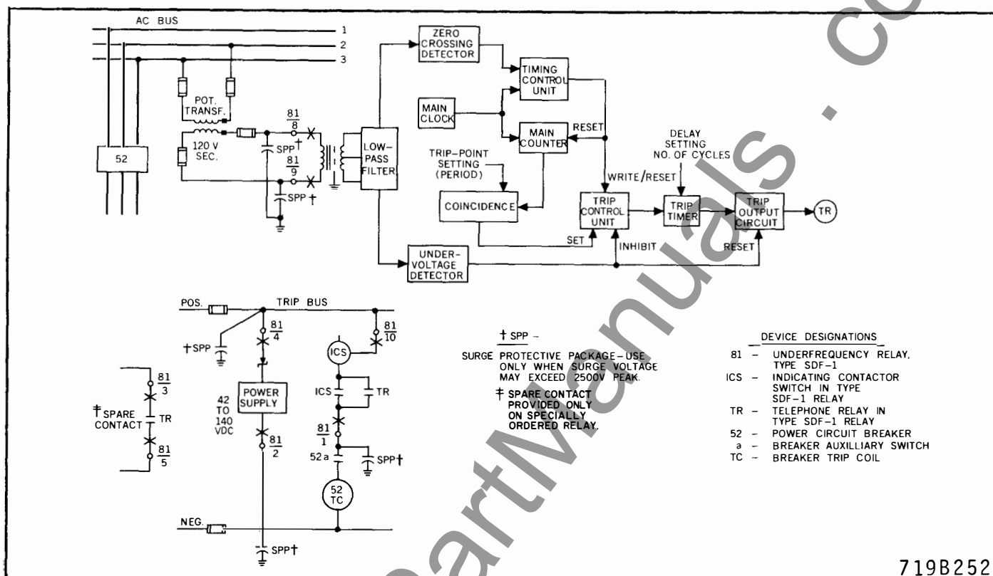
Fig. 4 External Schematic and Logic Diagram
