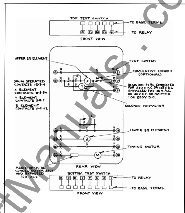
Fig. 4—Internal Schematic Connections of Type RC Reclosing Relay With Z Element. In the Type FT Flexitest Case.
