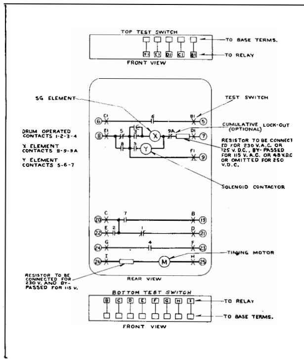
Fig. 3—Internal Schematic Connections of Type RC Reclosing Relay Without Z Element. In the Type FT Flexitest Relay Case.
