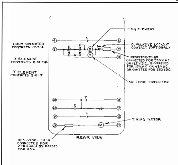
Fig. 1—Internal Schematic Connections of Type RC Reclosing Relay Without Z Element. In Standard Relay Case.
