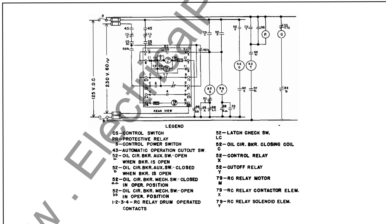
* Fig. 6-Typical External Connections of the Type RC Reclosing Relay Without Z Element, in Either Standard or Flexitest Case. Used in a D.C. Breaker Control Circuit.
