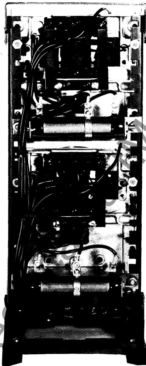
Fig. 1b. Non-Tapped Type CM Relay without case (Rear View)
