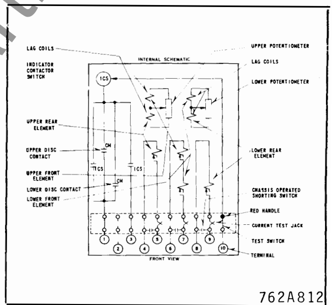
Fig. 3b. Internal Schematic of the tapped Type CM Relay in the Type FT31 Case
