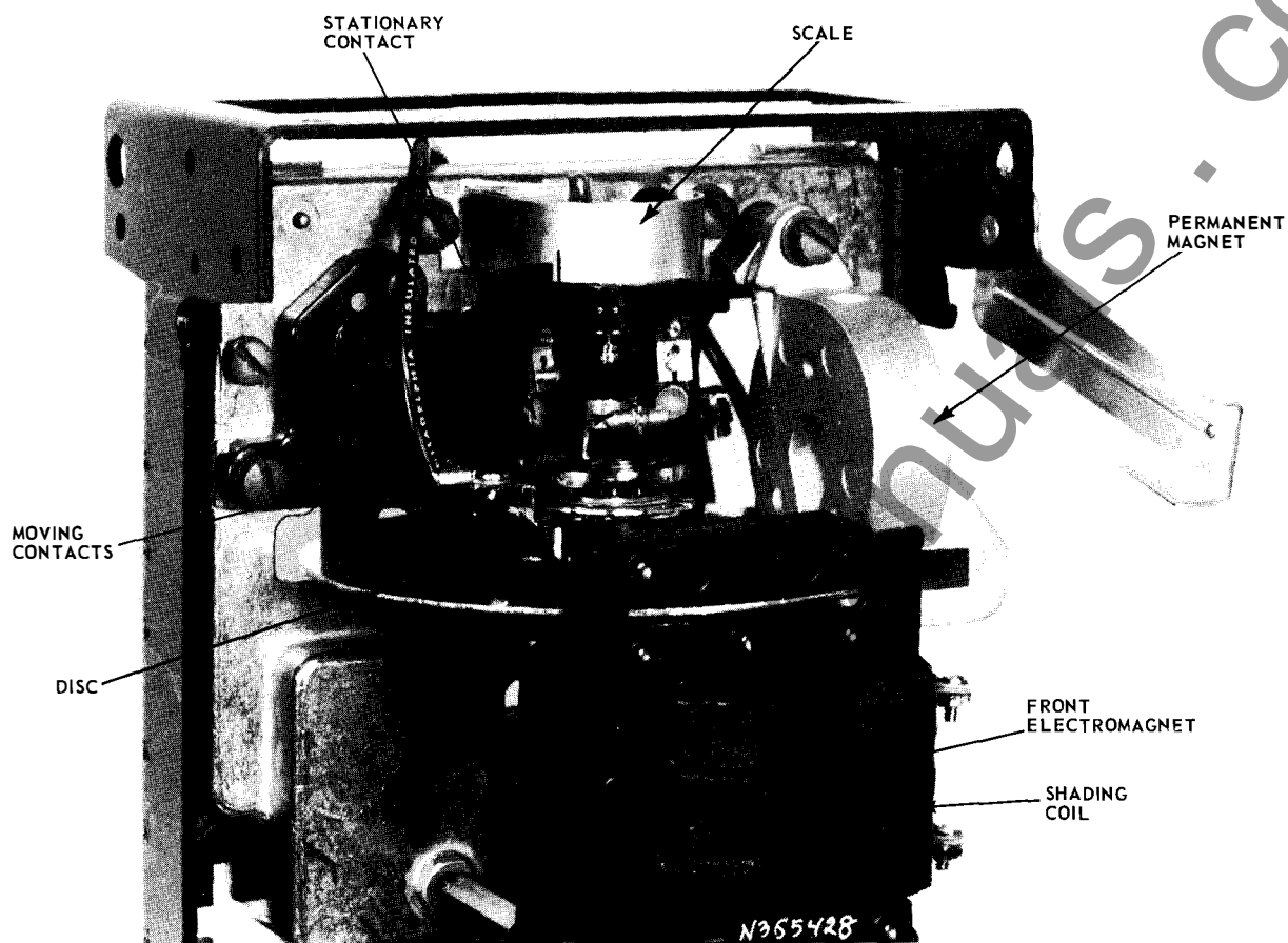
Fig. 8. Element Assembly Drawing for non-tapped CM Relay (Front View)
