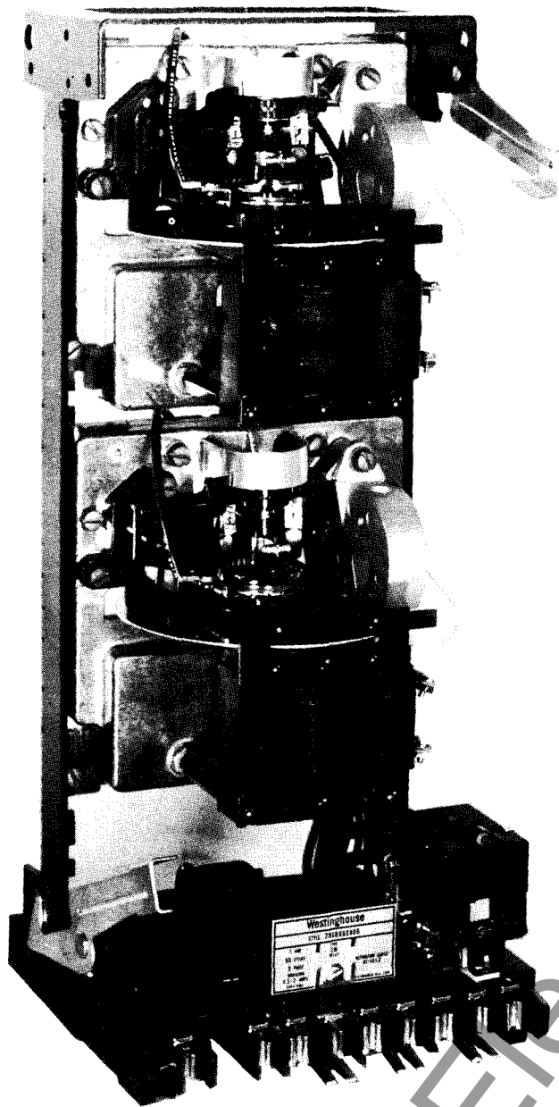
Fig. 1a. Non-Tapped Type CM Relay without case (Front View)
