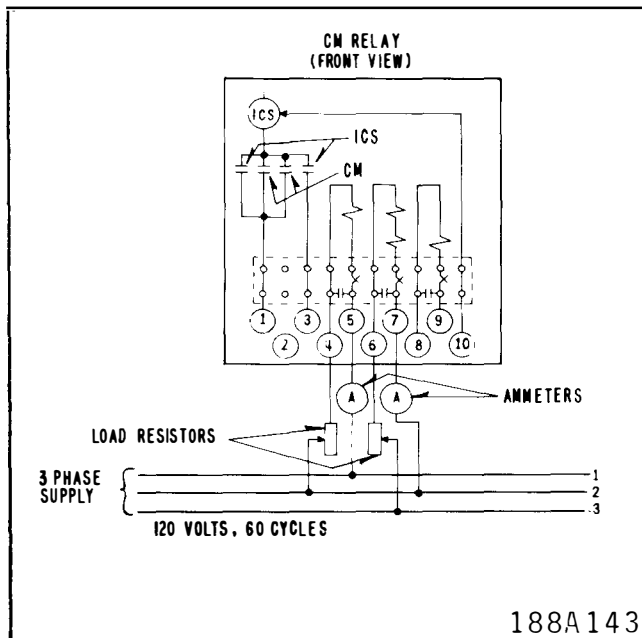
Fig. 6. Diagram of test connection for the non-tapped Type CM Relay in the FT31 Case. For tapped CM place tap screw in 1 amp. tap setting.
