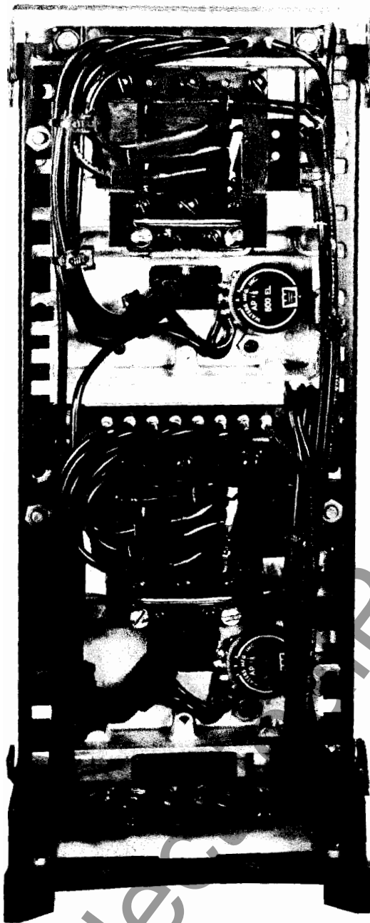
Fig. 2b. Type CM Tapped Relay (Rear View)
