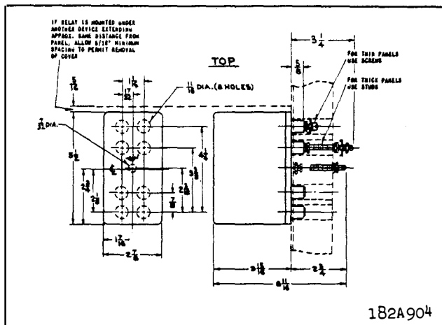
*Fig. 6 Outline and Drilling Plan for the Closed Type SG Auxiliary Relay with 5/8 inch terminal studs. For Reference Only.
