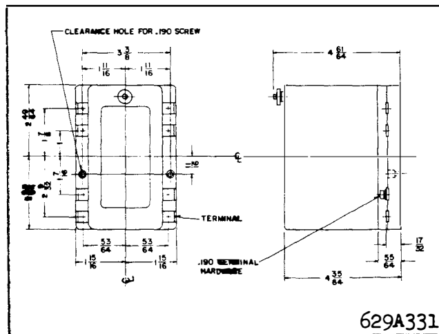
*Fig. 11 Outline and Drilling Plan for the Type SG Relay in Front Connected with dust cover.
