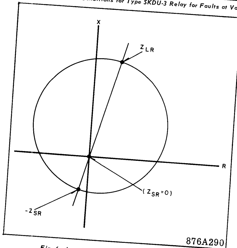
Fig. 6. Impedance Circle for Type SKDU-3 Relay.
