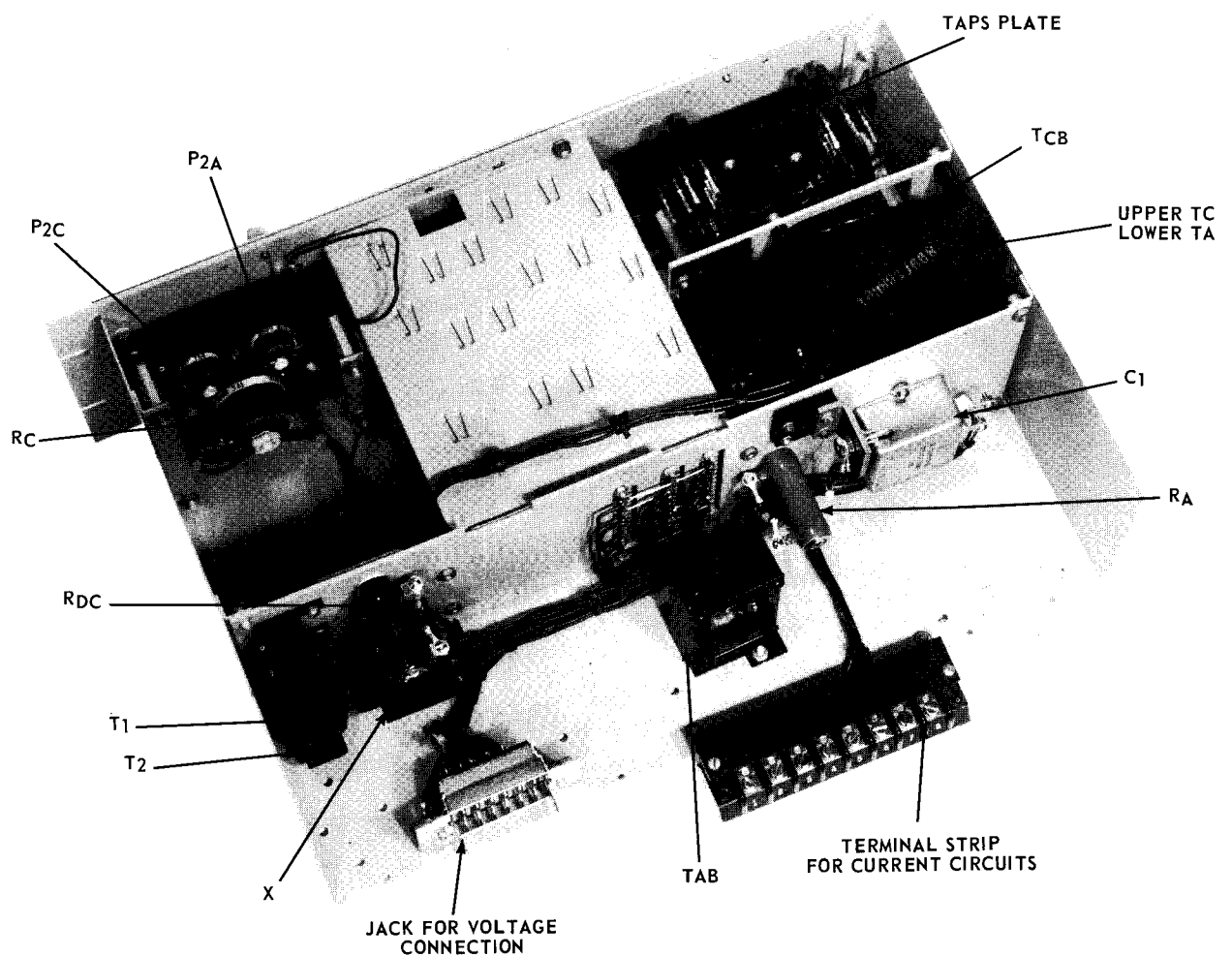
* Fig. 1. Type SKDU-3 Relay Without Case.
