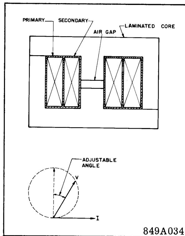
Fig. 2. Compensator Construction.
