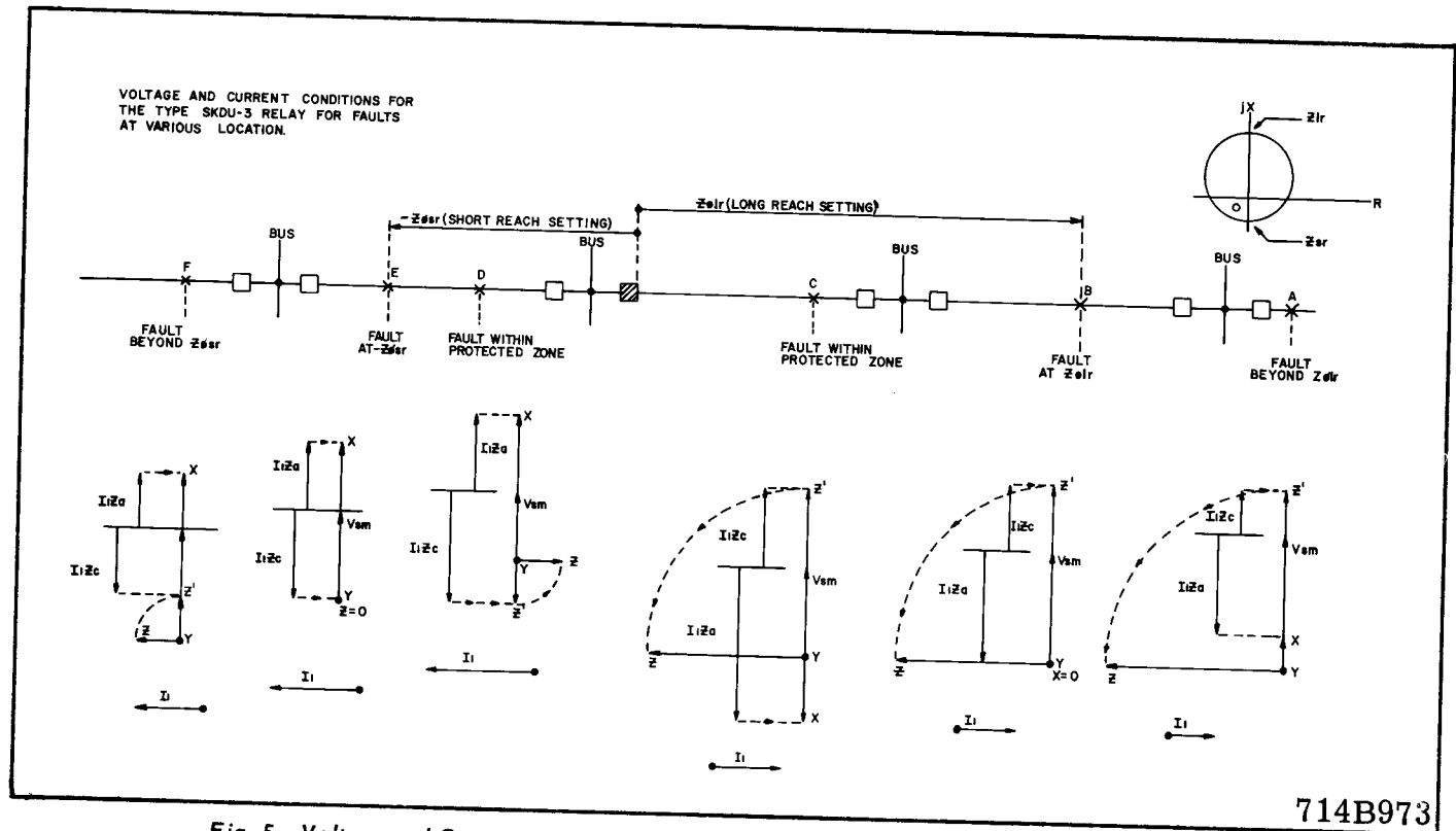
Fig. 5. Voltage and Current Conditions for Type SKDU-3 Relay for Faults at Various Locations.
