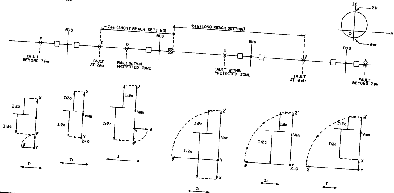
Fig. 5. Voltage and Current Conditions for Type SKDU-3 Relay for Faults at Various Locations.
