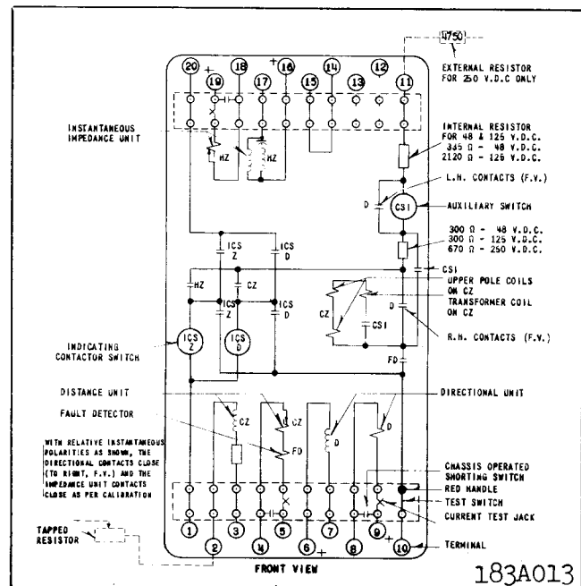
* Fig. 2. Internal Schematic of the Type HCZ Relay in the FT32 Case.
