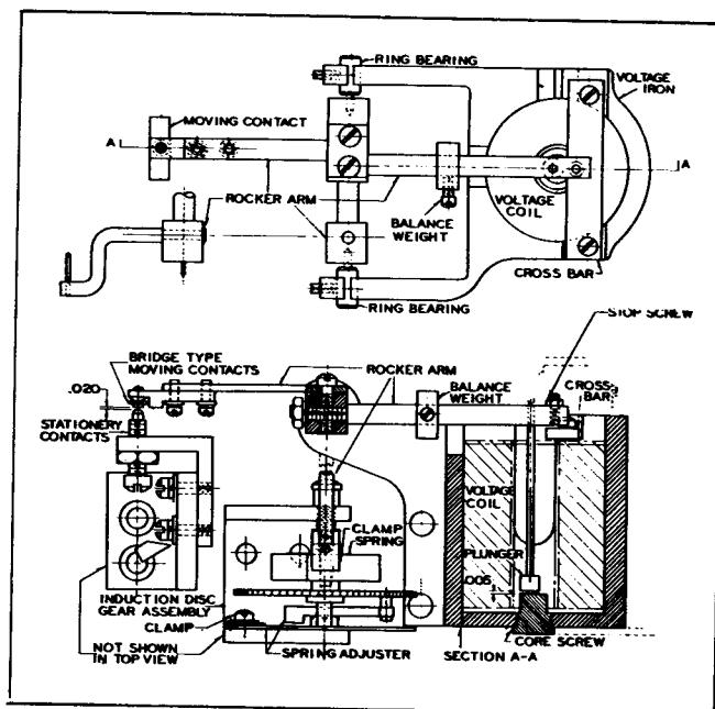
Fig. 4. Sectional View of the Time-Distance Unit (CZ).
