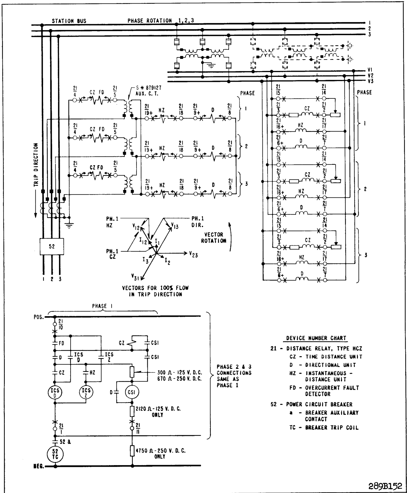
Fig. 12. External Schematic of the HCZ Relay in the FT32 Case.
