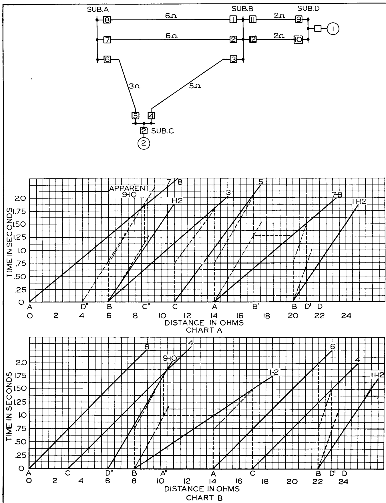
Fig. 9. Construction of a Time-Distance Chart for the Time-Distance Unit (CZ).
