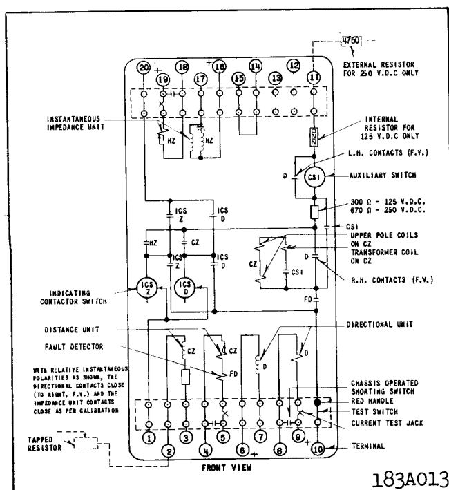
Fig. 2. Internal Schematic of the Type HCZ Relay in the FT32 Case.
