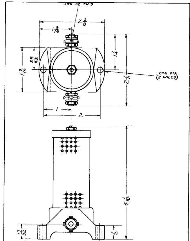
Fig. 15. Outline and Drilling Plan for Control Circuit Resistor - Used on 250 volt dc only. For Reference Only.
