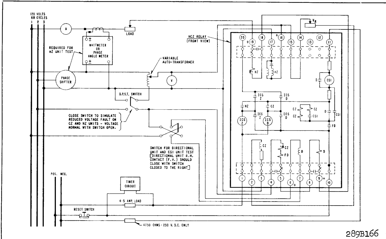
* Fig. 13. Diagram of Test Connections.
