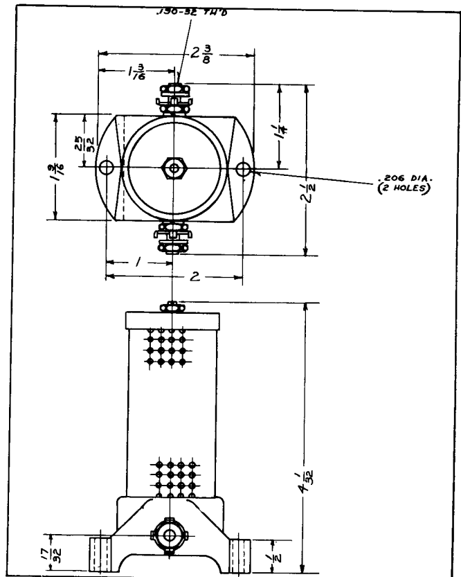
Fig. 15. Outline and Drilling Plan for Control Circuit Resistor - Used on 250 volt dc only. For Reference Only.
