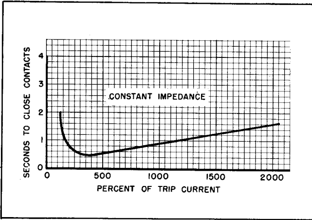
Fig. 11. Typical Time-Curve of the Time-Distance Unit (CZ) for Constant Impedance.
