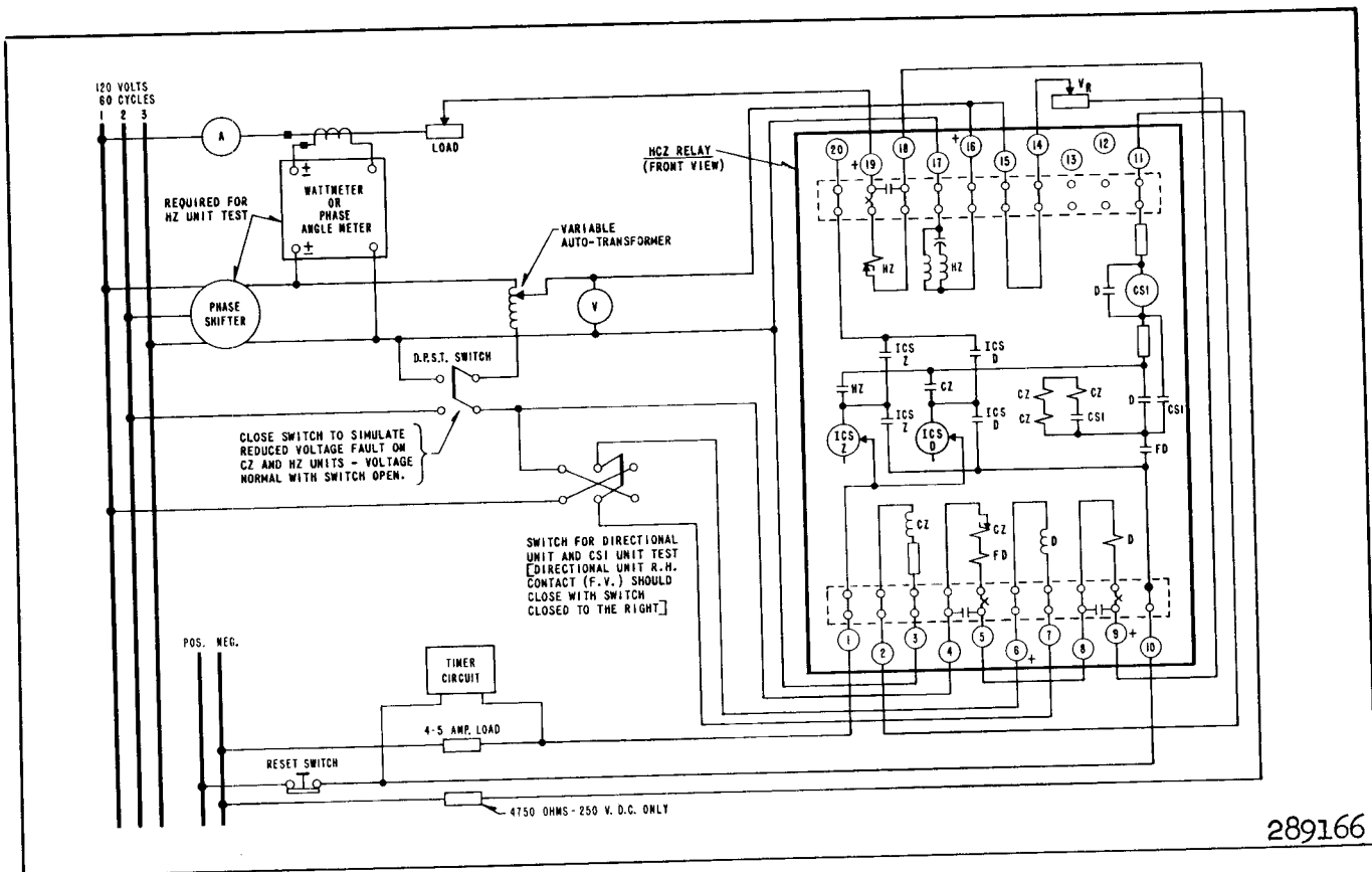
Fig. 13. Diagram of Test Connections.
