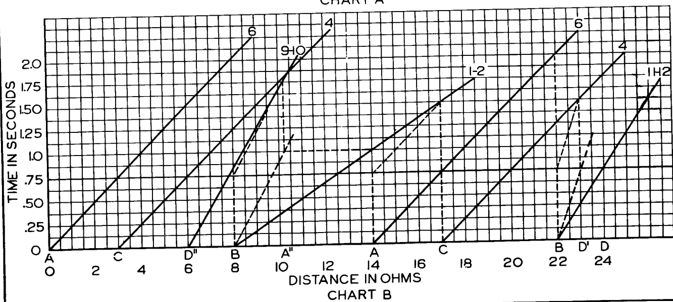
Fig. 9. Construction of a Time-Distance Chart for the Time-Distance Unit (CZ).
