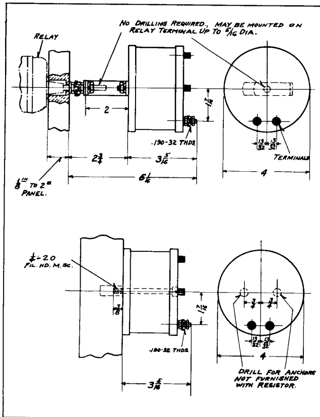
Fig. 14. Outline Drilling Plan for Resistor, VR, Used With Time-Distance Unit Potential Coil. For Reference Only.
