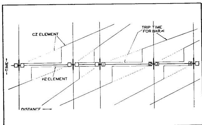
Fig. 1. Typical Time-Distance Characteristic of the Type HCZ Relay.
