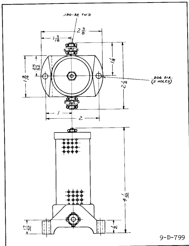
Fig. 15 —Outline And Drilling Plan For The External Control Circuit Resistor For The 250 Volt d-c Relays. For Reference Only.
