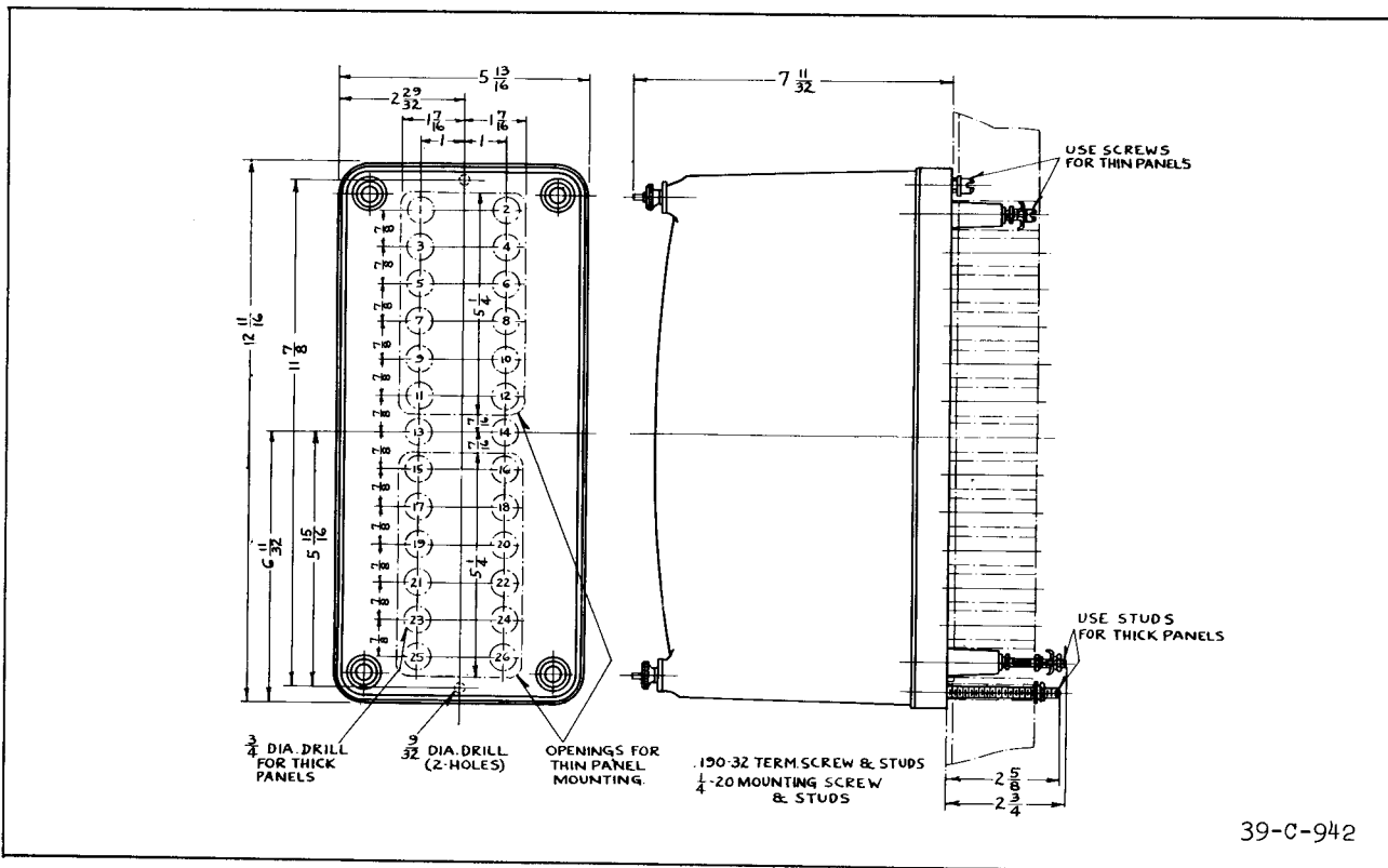
Fig. 16—Outline And Drilling Plan For The Standard Projection Type Case. See The Internal Schematics For Terminals Supplied. For Reference Only.
