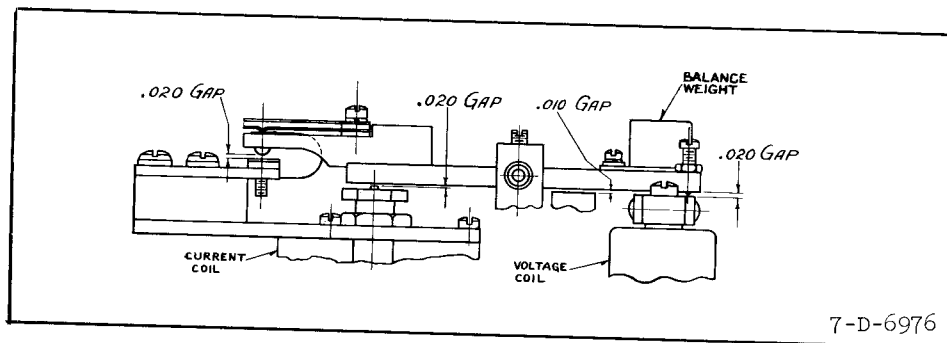
Fig. 1—Sectional View of the Impedance Elements.
