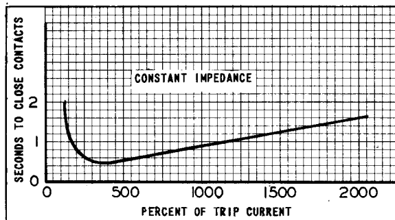
Fig. 13 — Typical Time-Ampere Curve of the Distance (CZ) Element for a Constant Given Distance.
