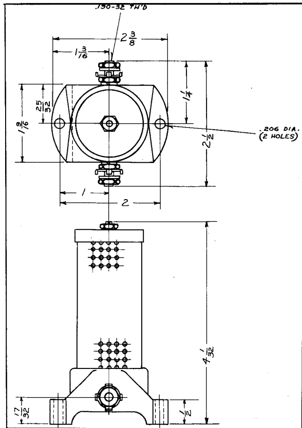
Fig. 24 — Outline and Drilling Plan for the External Control Circuit Resistor for the 250 Volt D-C Relays. For Reference Only.
