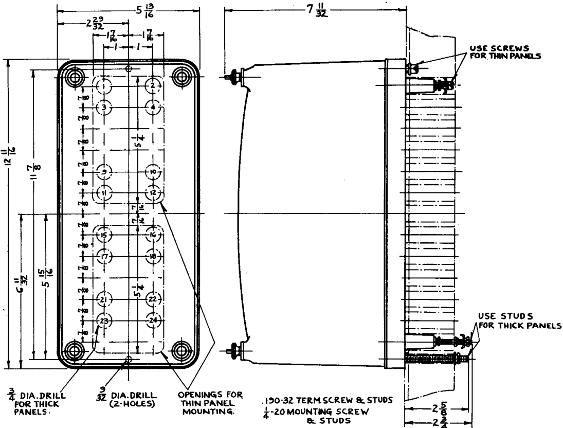
Figure 19 Outline and Drilling Plan for the Standard Projection Type Case
