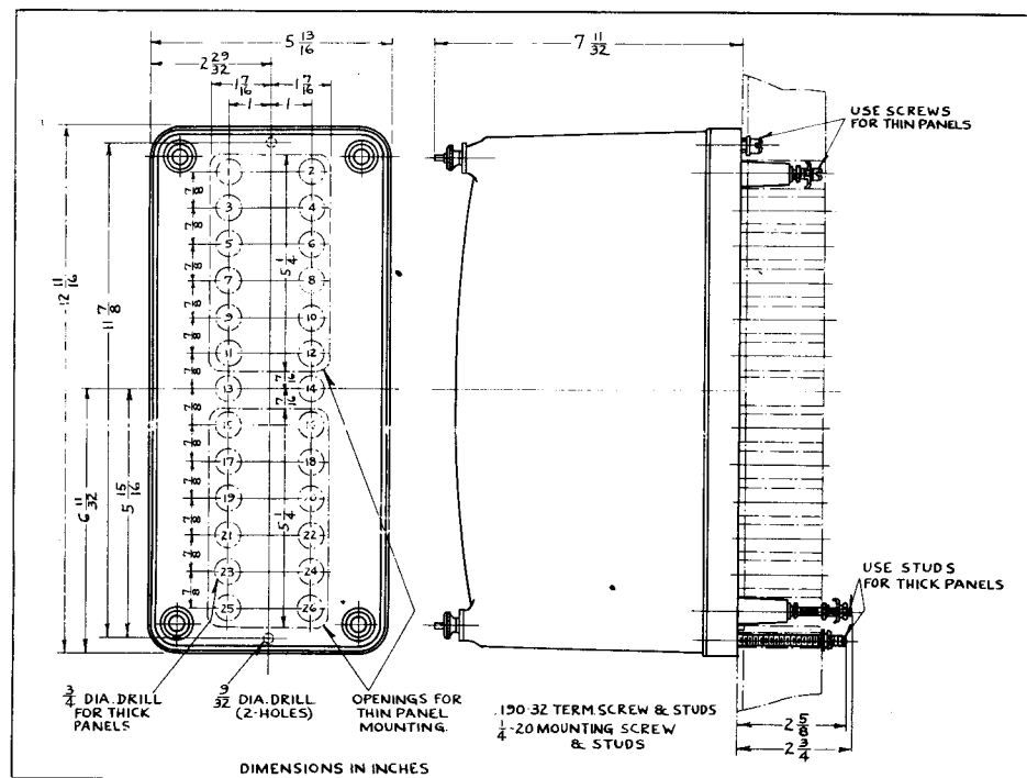
Fig. 20 — Outline and Drilling Plan for the Standard Projection Type Case. See the Internal Schematics For Terminals Supplied. For Reference Only.
