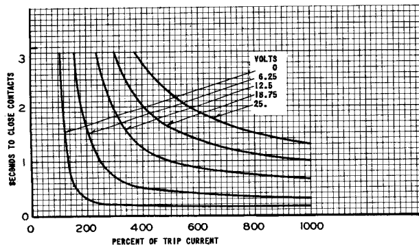
Figure 11 Typical Time-Ampere Curves of the Distance (CZ) Element (Enlarged)
