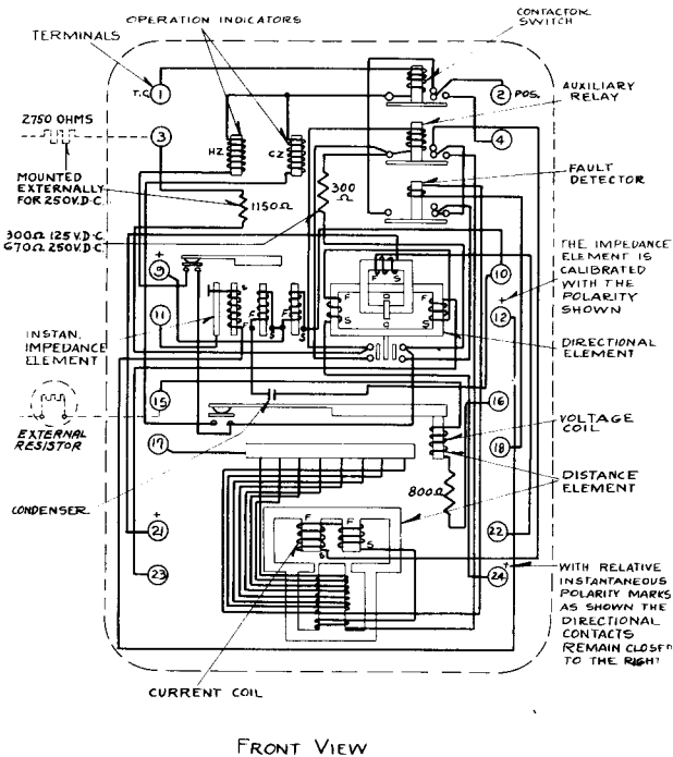
Figure 2 Internal Connections of the Type HCZ Relay
