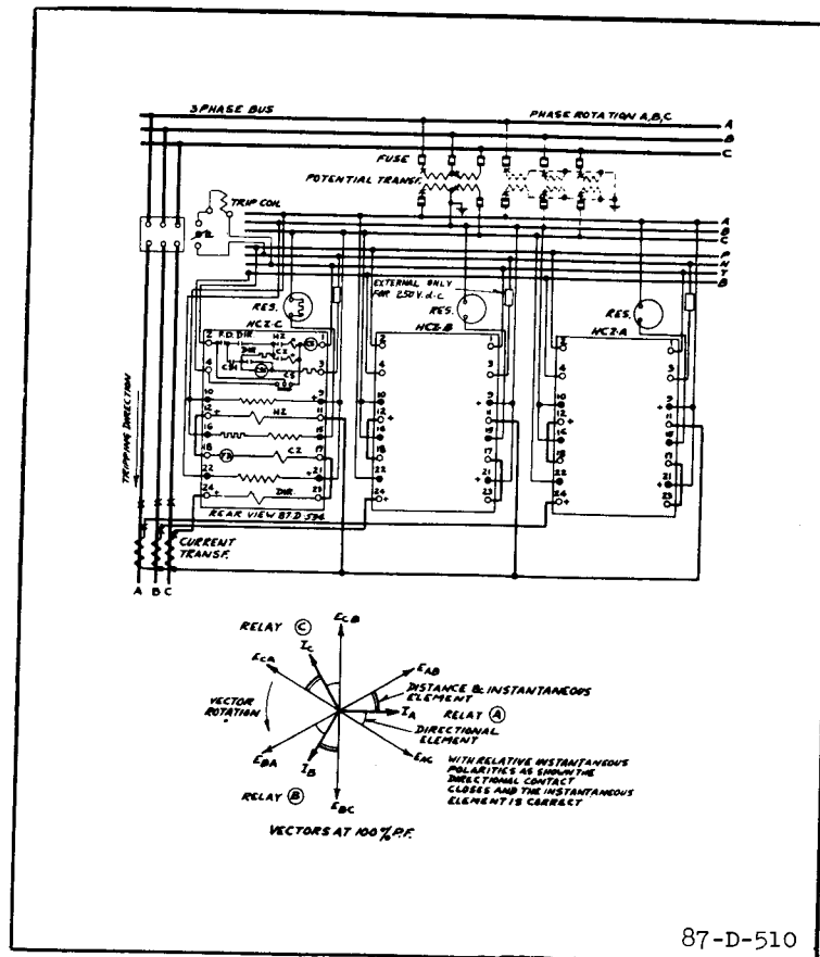
Fig. 17 — External Connections of the Type HCZ Relay in the Standard Case Using Star Current for All Elements.
