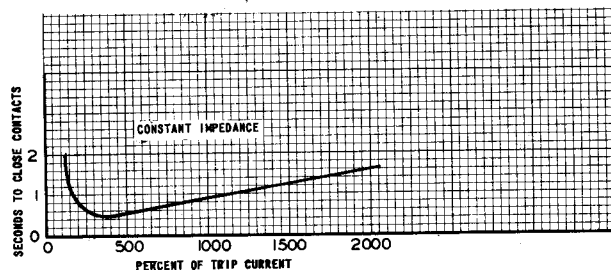
Figure 12 Typical Time-Ampere Curve of the Distance (CZ) Element for a Constant Given Distance.
