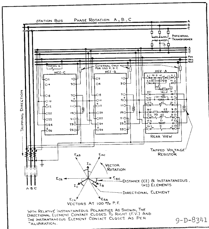
Fig. 19 — External Connections of the Type HCZ Relay in the Type FT Case Using Star Current for All Elements.
