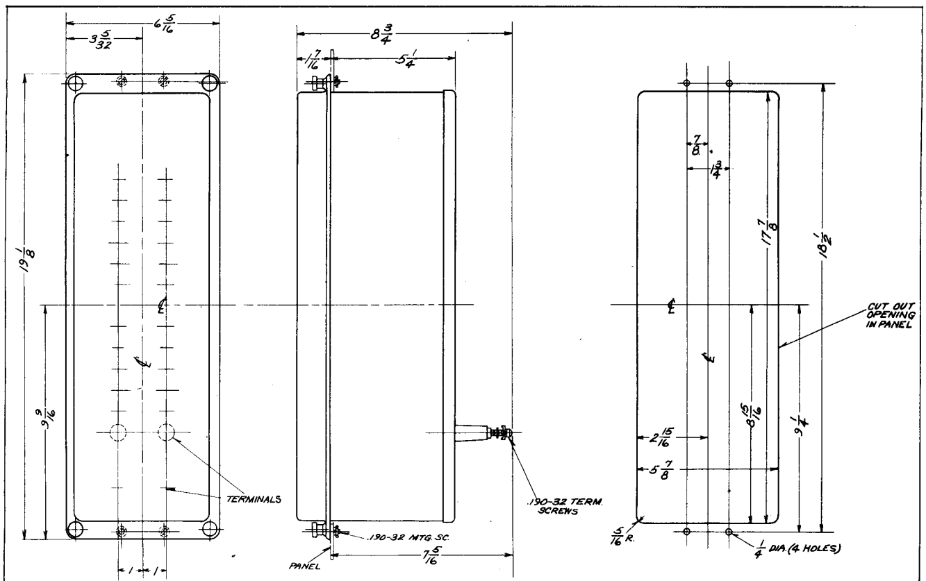
Fig. 21 — Outline and Drilling Plan for the Flush Type FT Flexitest Case. For Reference Only.
