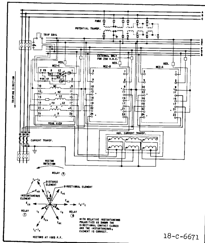
* Fig. 16 — External Connections of the Type HCZ Relay in the Standard Case Using Star Current for the Directional and Distance Elements and Delta Current for the Instantaneous Element.
