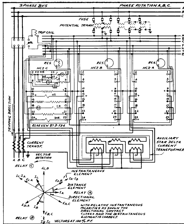
Fig. 16 — External Connections of the Type HCZ Relay in the Standard Case Using Star Current for the Directional and Distance Elements and Delta Current for the Instantaneous Element.
