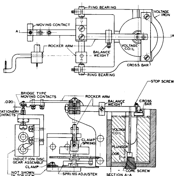
Figure 4 Sectional View of the Distance (CZ) Element
