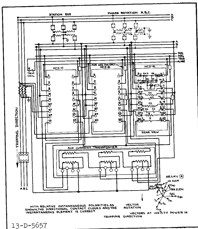
* Fig. 18 — External Connections of the Type HCZ Relay in the Type FT Case Using Star Current for the Directional and Distance Elements and Delta Current for the Instantaneous Element.
