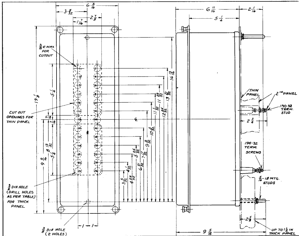
Fig. 22 — Outline and Drilling Plan for the Projection Type FT Flexitest Case. See the Internal Schematics for Terminals Supplied. For Reference Only.
