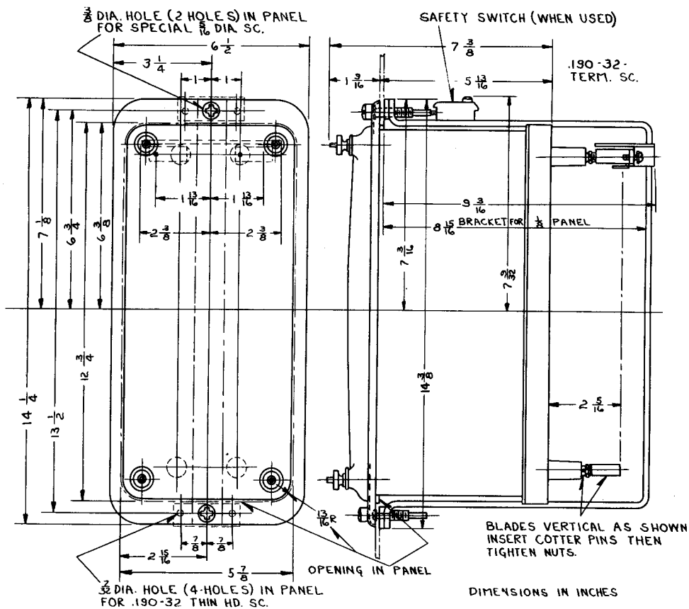
Figure 20 Outline and Drilling Plan for the Standard Flush Detachable Type Case. (1/8" panel mounting.)
