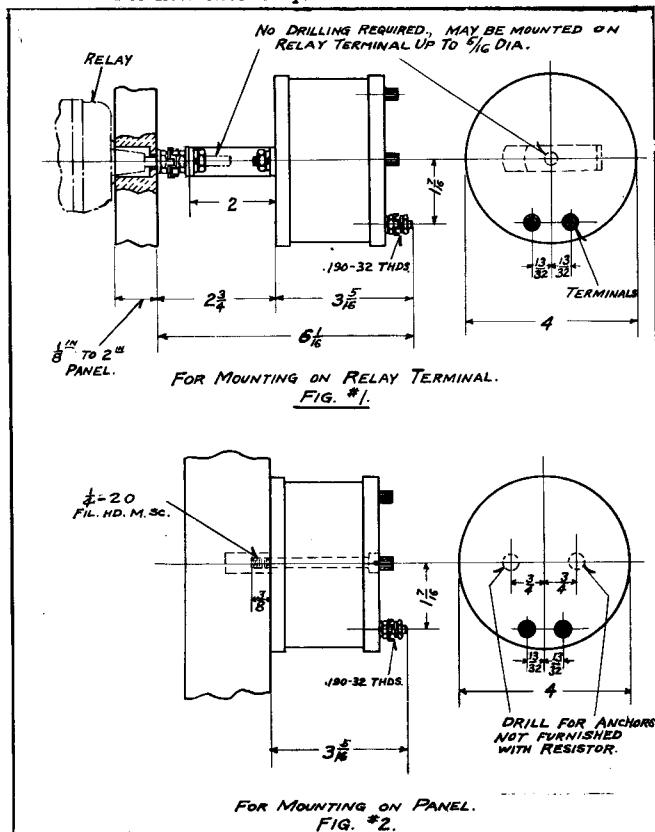
Fig. 23 — Outline and Drilling Plan for the Tapped A-C Voltage Resistor for the Distance (CZ) Element. For Reference Only.
