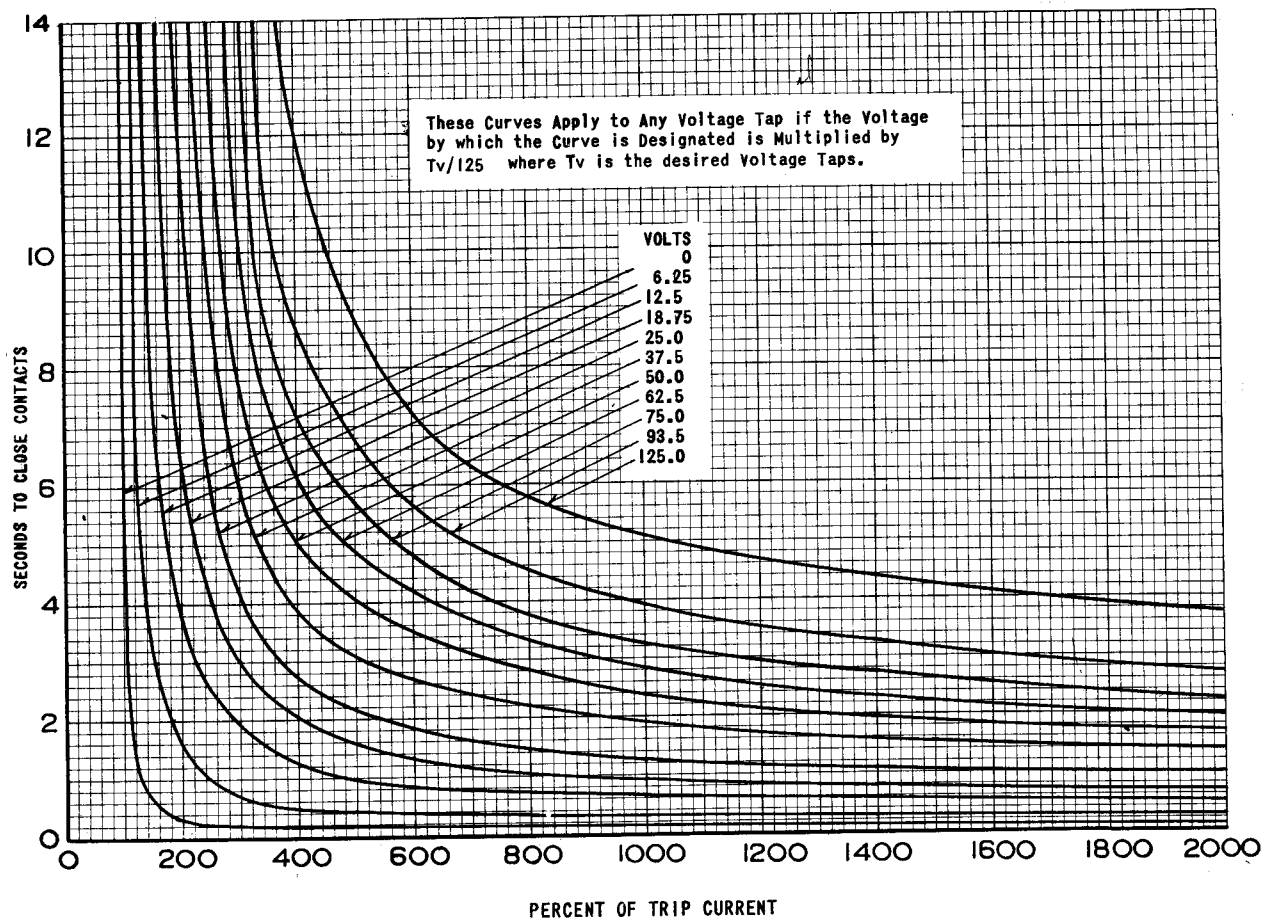
Figure 10 Typical Time-Ampere Curves of the Distance (CZ) Element
