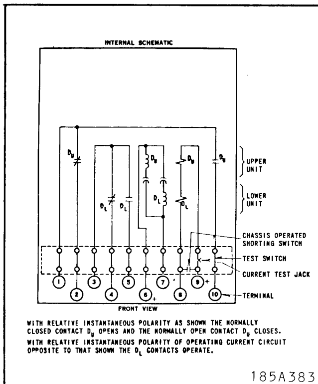
Fig. 1 Internal Schematic.
