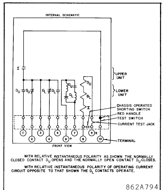
Fig. 2 Internal Schematic (with IT Unit) (.02 to 1 amp range)
