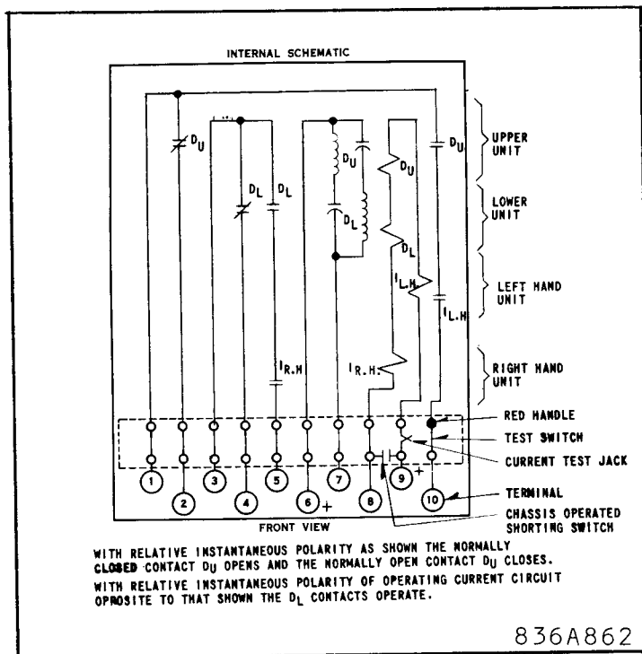
Fig. 2a Internal Schematic (with IT Units) (.5 to 2 amp range)
