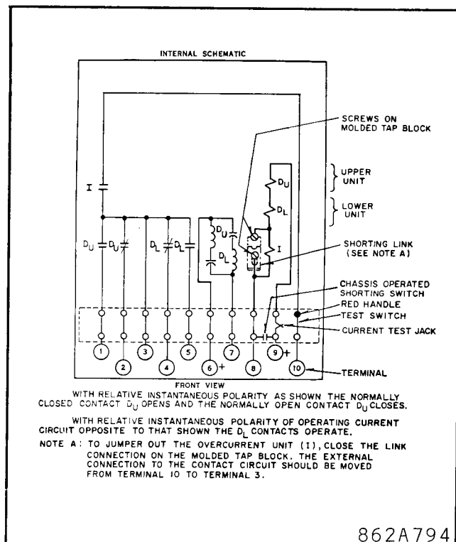
* Fig. 2 Internal Schematic (with IT Unit) (.02 to 1 amp range). Relays with suffix letter "A" on nameplate style have shorting link feature.
