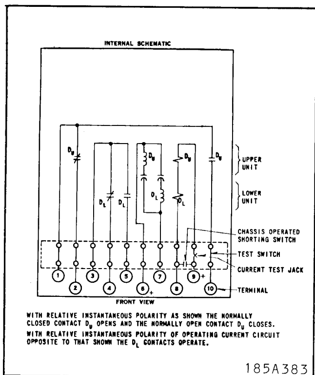
* Fig. 1 Internal Schematic. (Without IT Unit)
