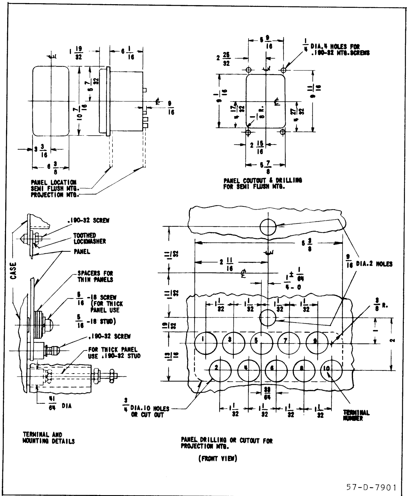
Fig. 4. Outline and Drilling (FT-21 Case)
