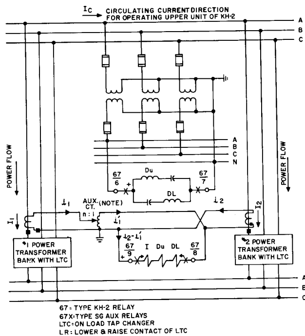
Fig. 3 External Schematic
