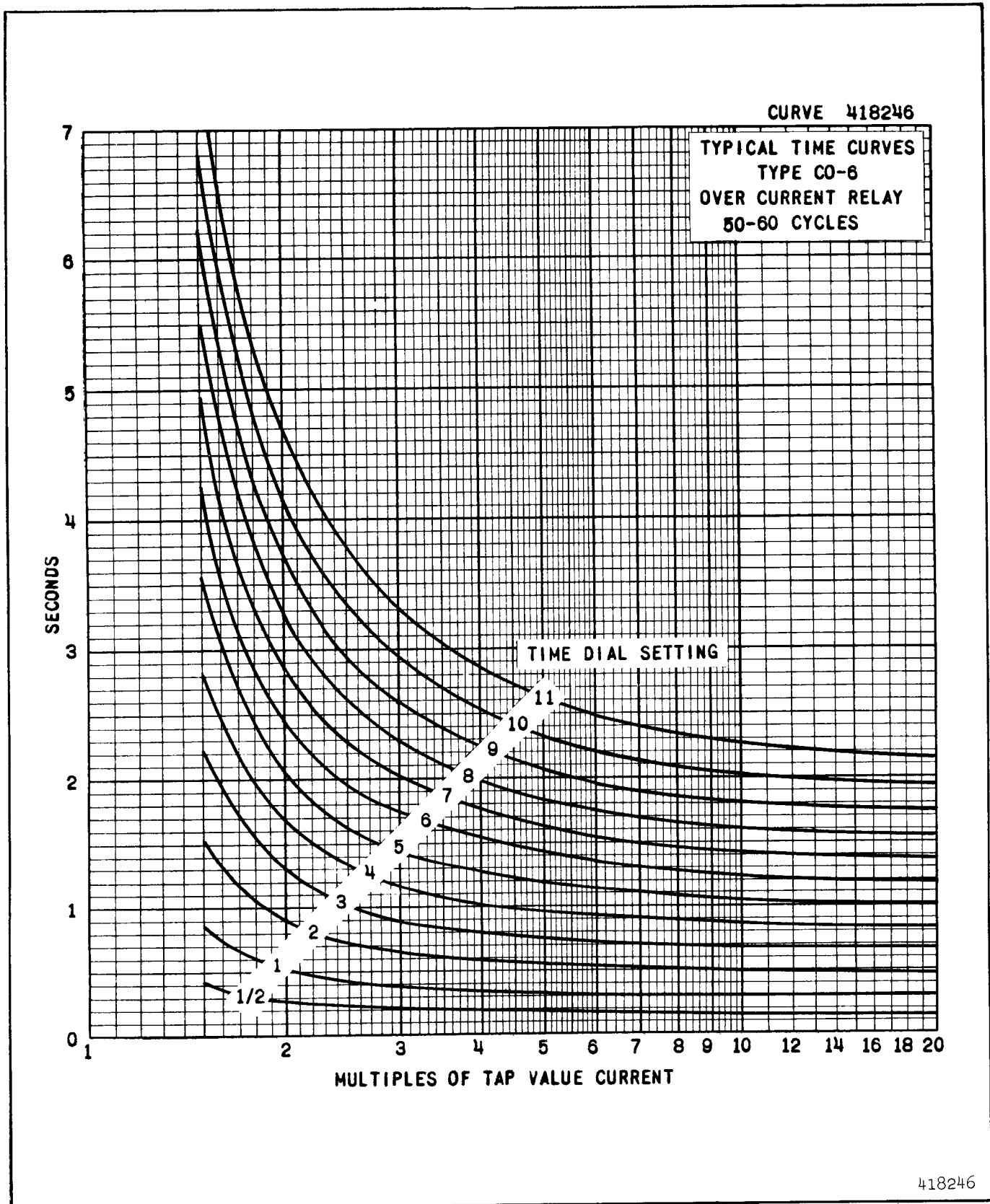
Fig. 4. Typical 50 and 60 Cycle Time Curves of COV-6 Overcurrent Unit.
