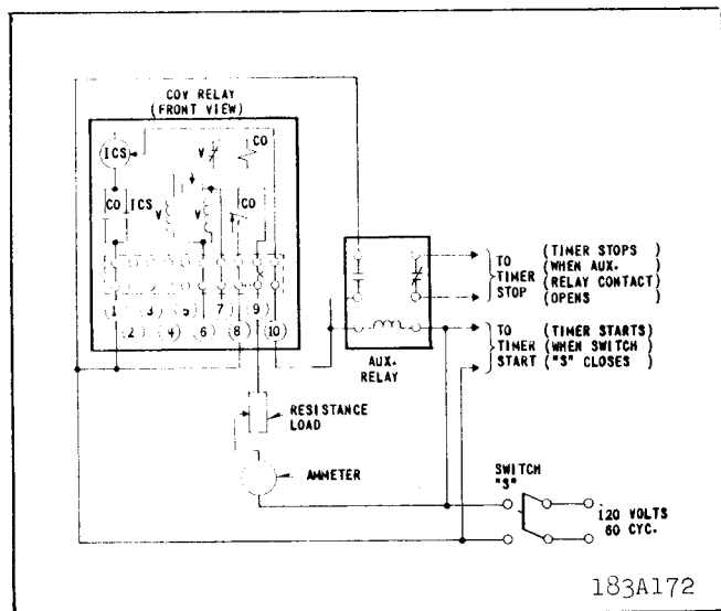
Fig. 8. Diagram of Test Connections of the Overcurrent Unit.
