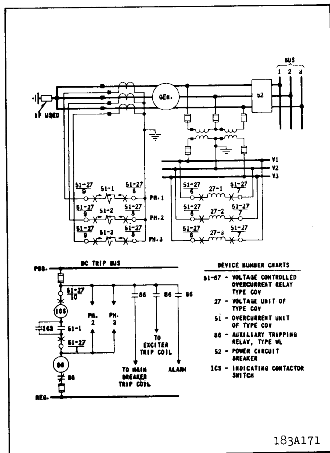
Fig. 9. External Schematic of the Type COV Relay on a Generator.
