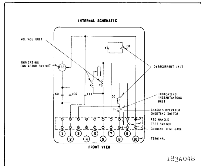
* Fig. 2. Internal Schematic of the Type COV Relay with Indicating Instantaneous Trip Unit in the Type FT21 Case.
