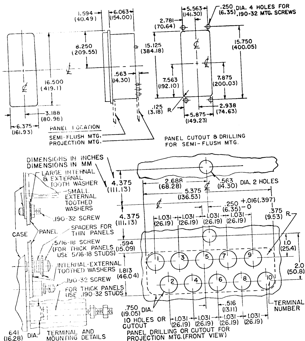
Fig. 17. Outline and Drilling Plan for the CKO Relay in the Type FT31 Case.
