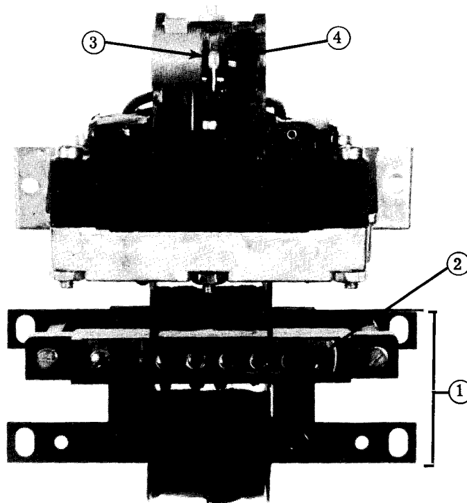
Fig. 4. Instantaneous Overcurrent Unit. 1 - Saturating Transformer. 2 - Tap Block. 3 - Stationary Contact. 4 - Moving Contact.
