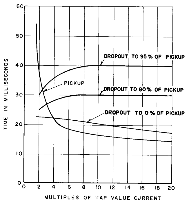
Fig. 14. Maximum Pickup and Dropout Time Curves for Instantaneous Overcurrent Unit.
