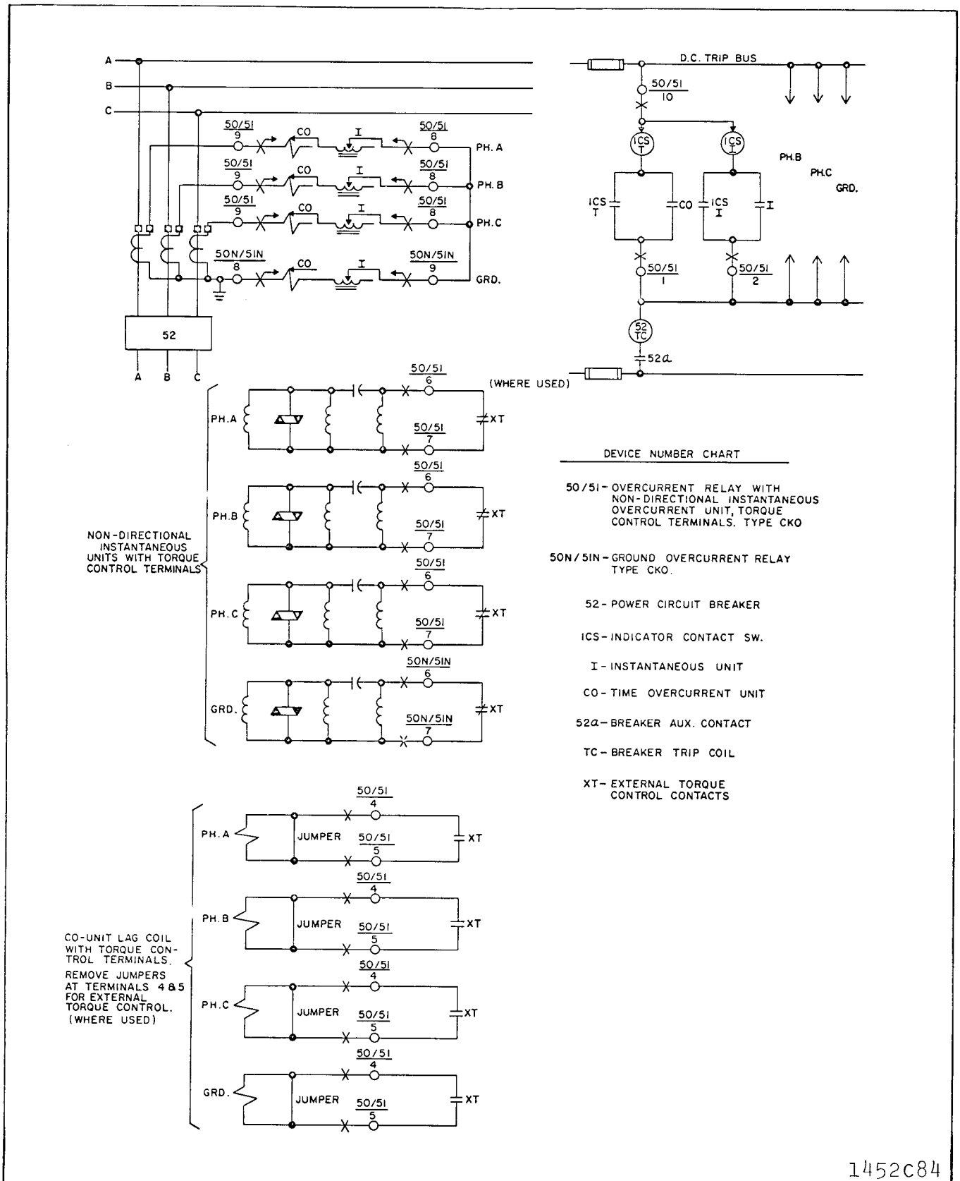
Fig. 16. External Schematic of the CKO Relay.
