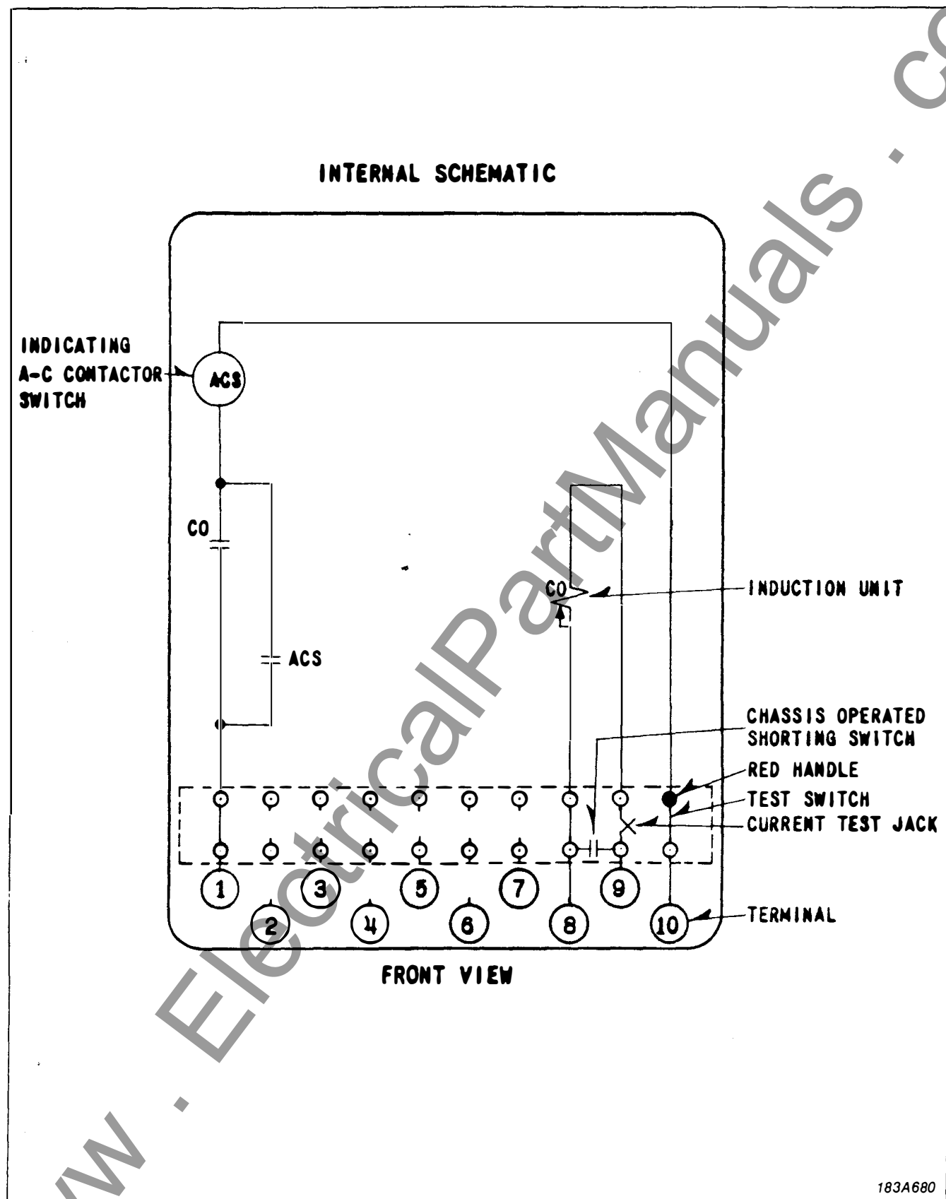
Fig. 7. Internal Schematic of the Single Trip Relay with an ACS Unit
