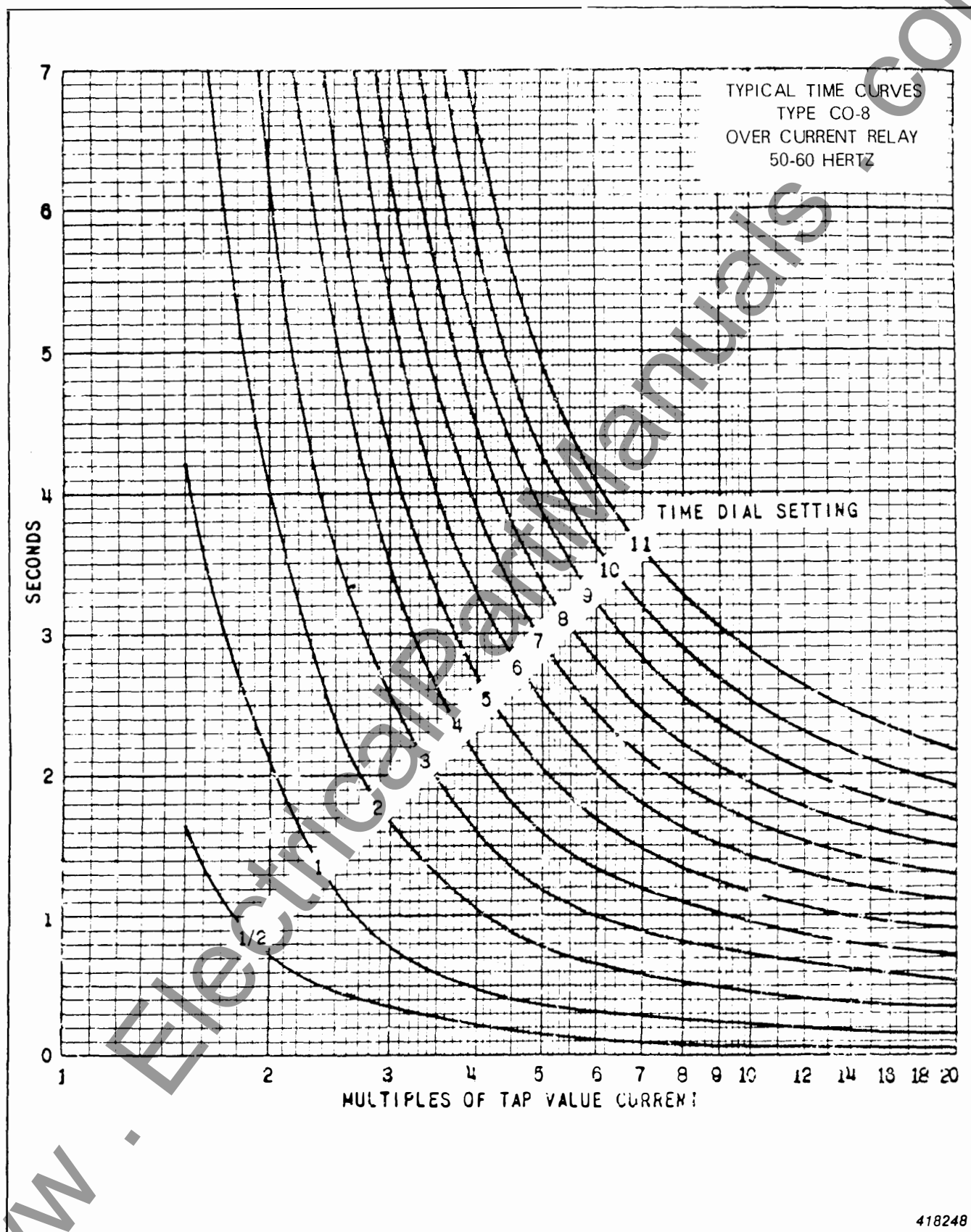
Fig. 14. Typical Time Curve of the Type CO-8 Relay
