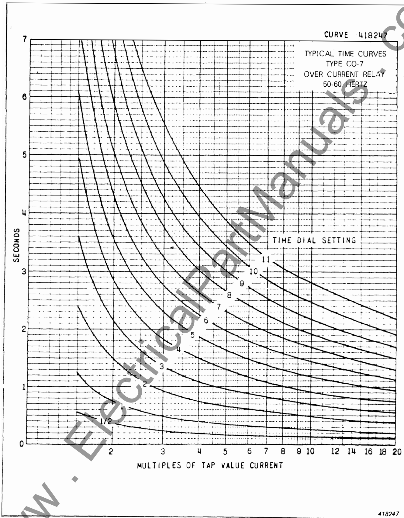
Fig. 13. Typical Time Curve of the Type CO-7 Relay
