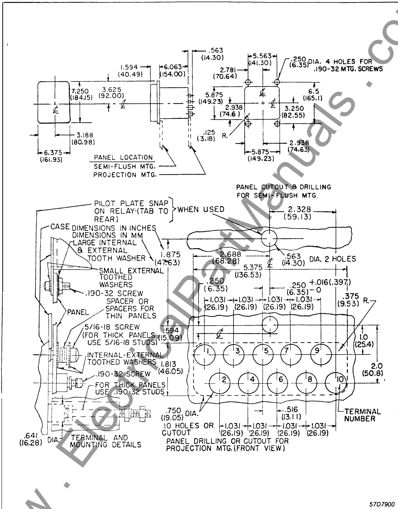
Fig. 22. Outline and Drilling Plan for the Type CO Relay.
