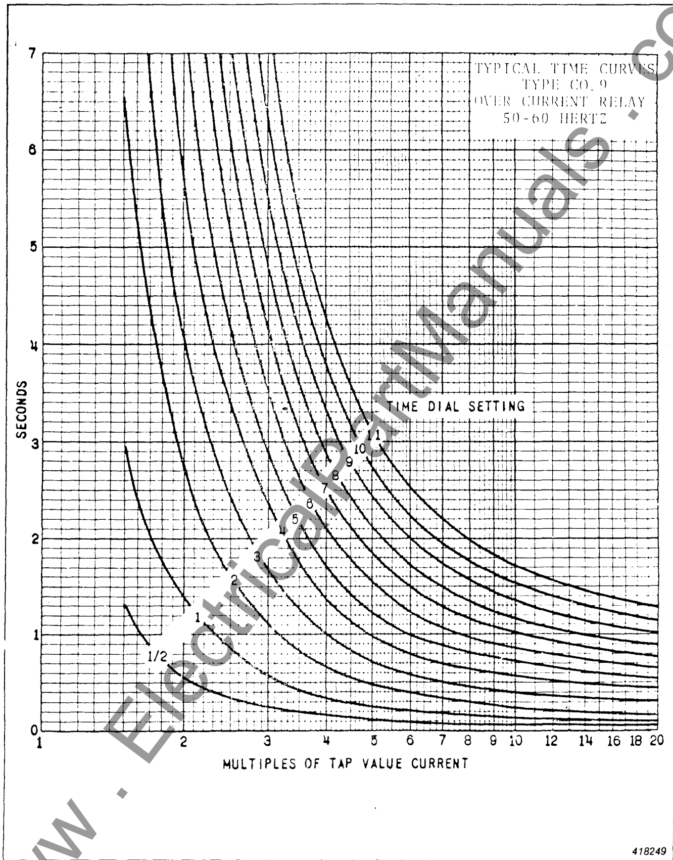
Fig. 15. Typical Time Curve of the Type CO-9 Relay
