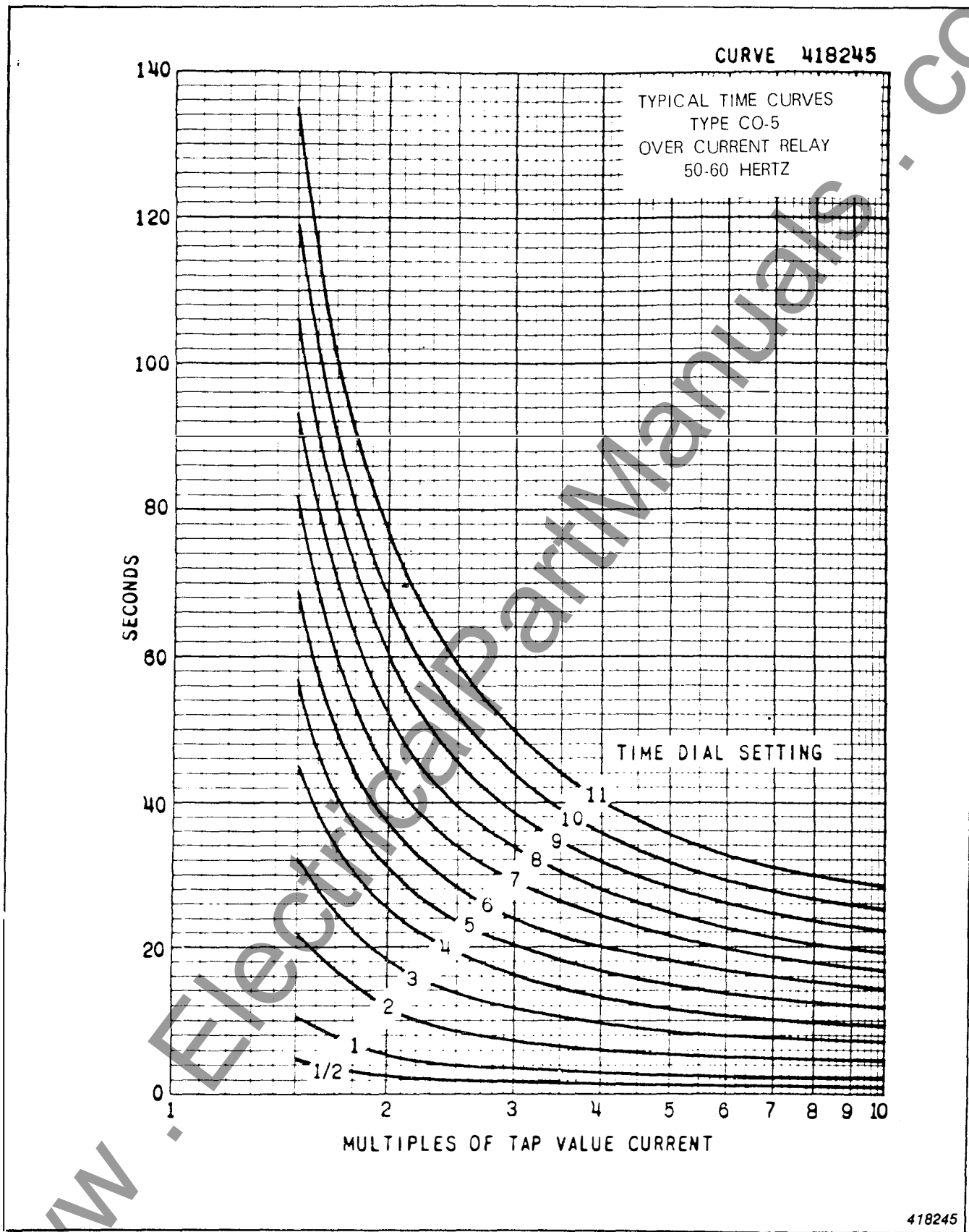
Fig. 11. Typical Time Curve of the Type CO-5 Relay
