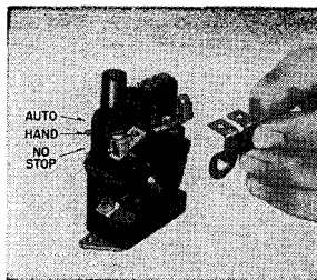
FIG. 1. Thermal Overload Relay, Showing Heater and Installation Method
