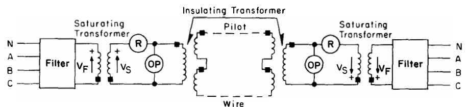
Fig. 2: Simplified External Schematic.
