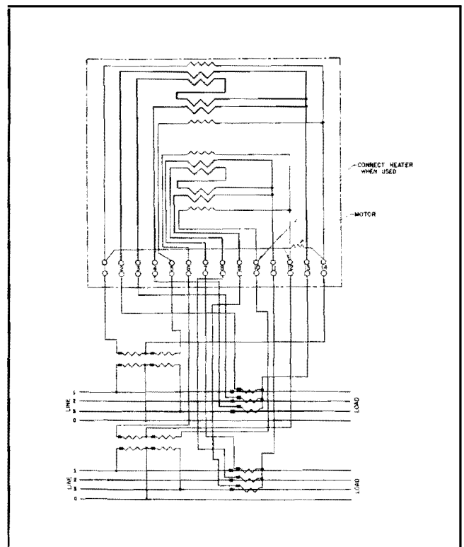
Fig. 36 - Type R-38, Totalizing, Two 3-Phase, 4-Wire "Y" Circuits
