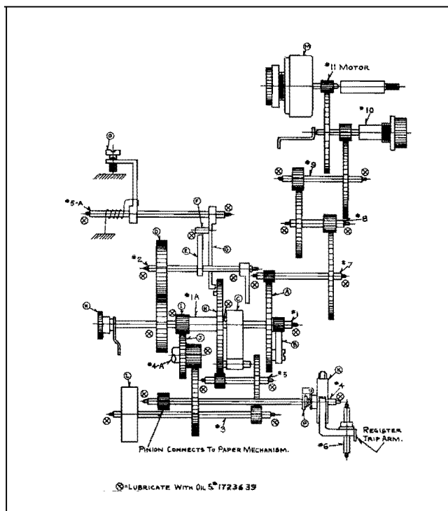
Fig. 37 - Schematic Diagram of Clock Mechanism
