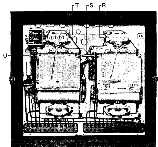
Fig. 40 — Type R-23 Duplex Recording Demand Meter
