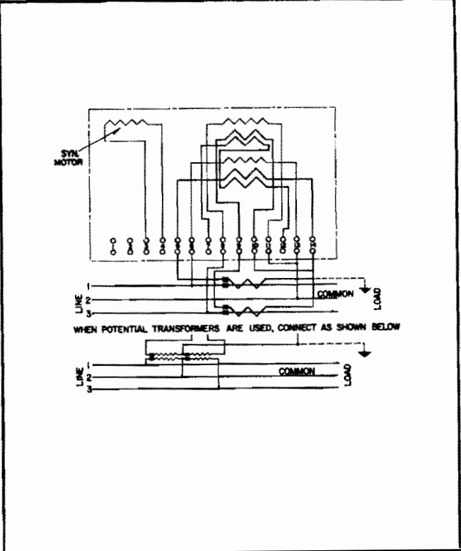
Fig. 25 - Type R-8, 3-Phase, 3-Wire
