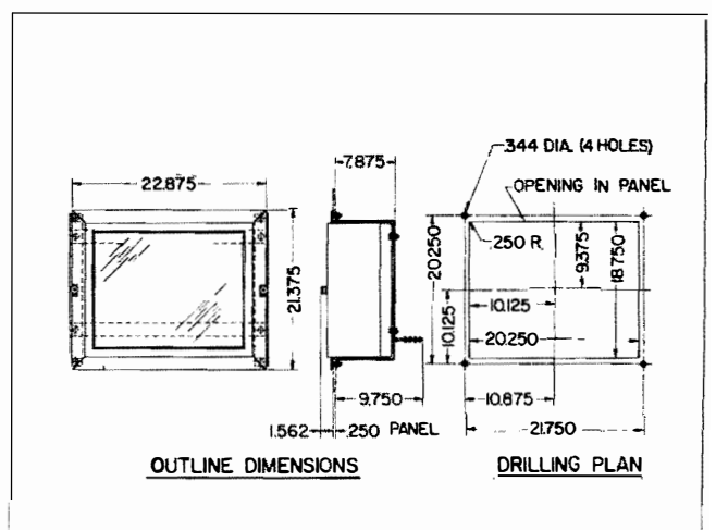
Fig. 13 - Type R-23 Meters, Flush Type
