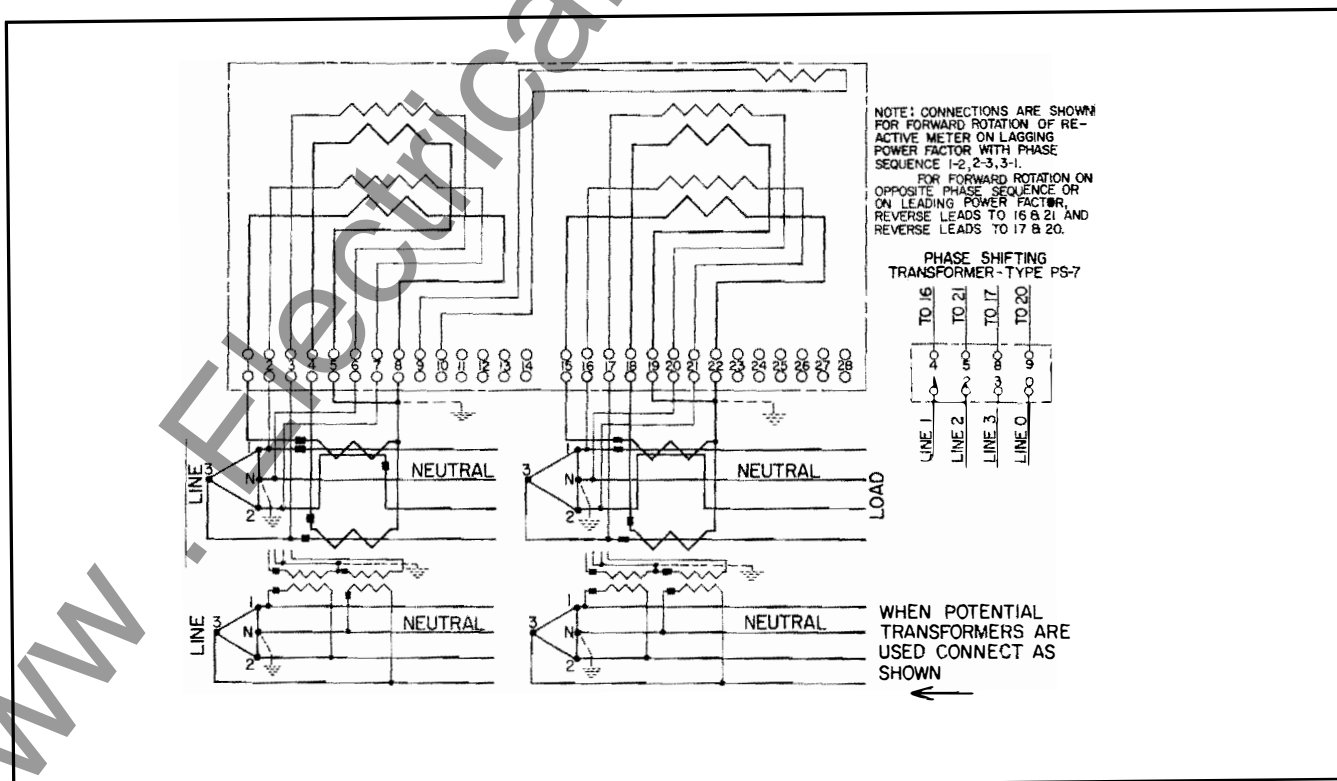
Fig. 28 - Type R-22, Duplex, 3-Phase, 4-Wire Delta
