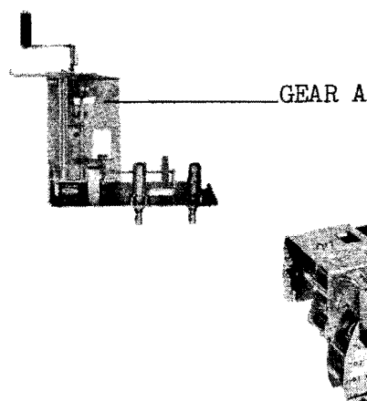
Fig. 9 Gear Checker for Mark Ia Register Style No. 111C217G01
