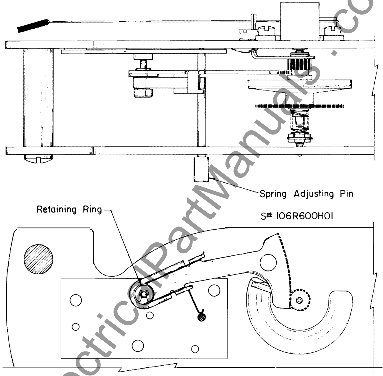
Fig. 7 Sector Adjustment
