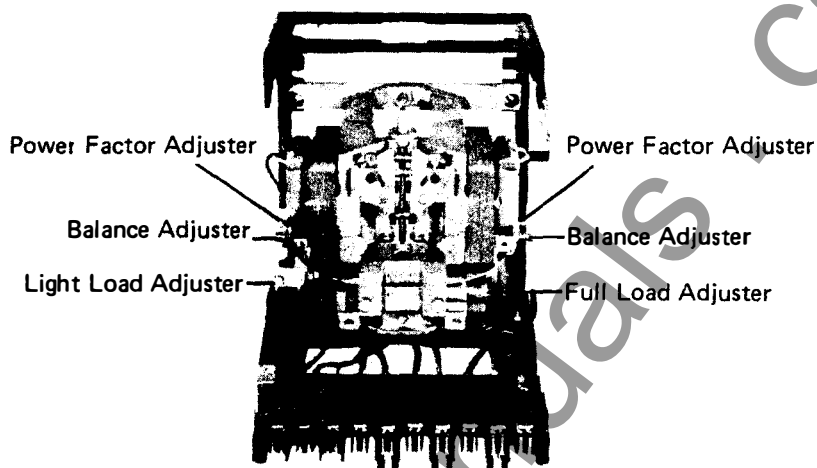
D4B-7F Chassis
