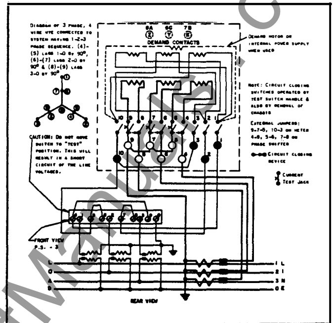
Fig. 10 - Type D4B-3F, 3-Phase, 4-Wire Wye with Phase-Shifting Transformer
