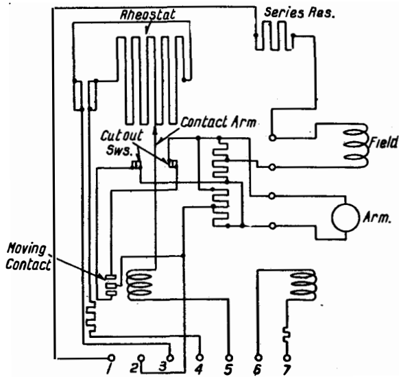
Figure 11 Transmitting D-C. Ammeter or Voltmeter Internal Connections.
