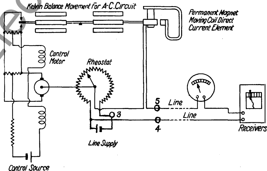
Figure 1 Connection Diagram of One Transmitter to Receivers Connected in Series.
