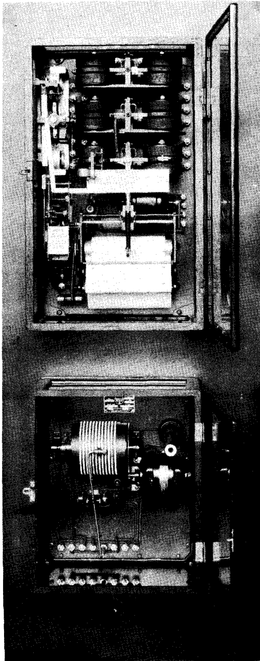
Figure 3 Totalizing Wattmeter and Transmitter.
