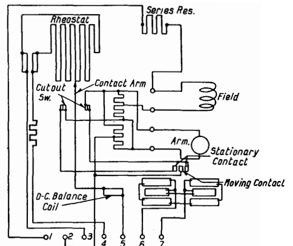
Figure 10 Transmitting A-C. Ammeter--Internal Connections
