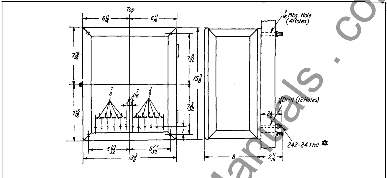
Fig. 13—Outline and Drilling Plan.
