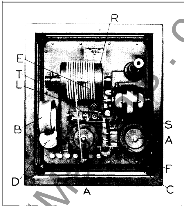
Fig. 2—Transmuting Voltmeter.
