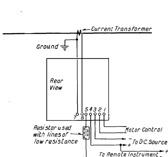
Figure 4 Transmitting A-C Ammeter Diagram.
