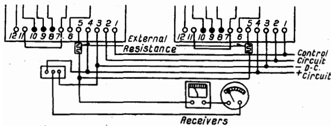
Figure 7 Showing Center-Tap External Resistor Used For Wattmeters Calibrated for Center Zero. In Other respects this Diagram is the Same as Figure 6.
