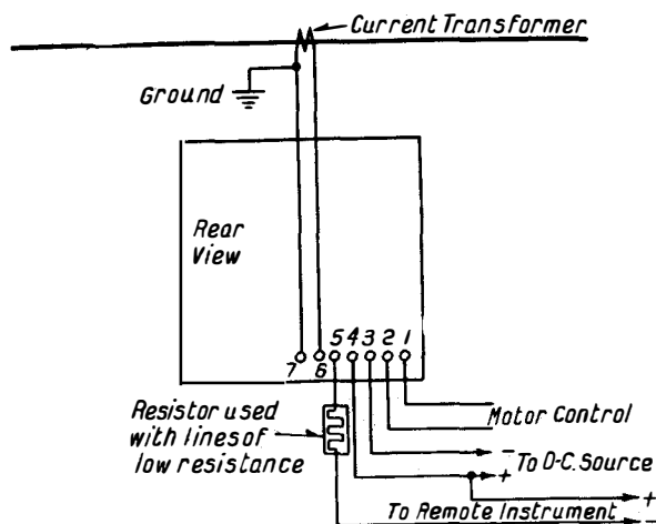
Figure 4 Transmitting A-C Ammeter Diagram.
