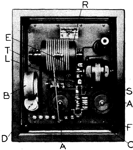
Figure 2 Transmitting Voltmeter.
