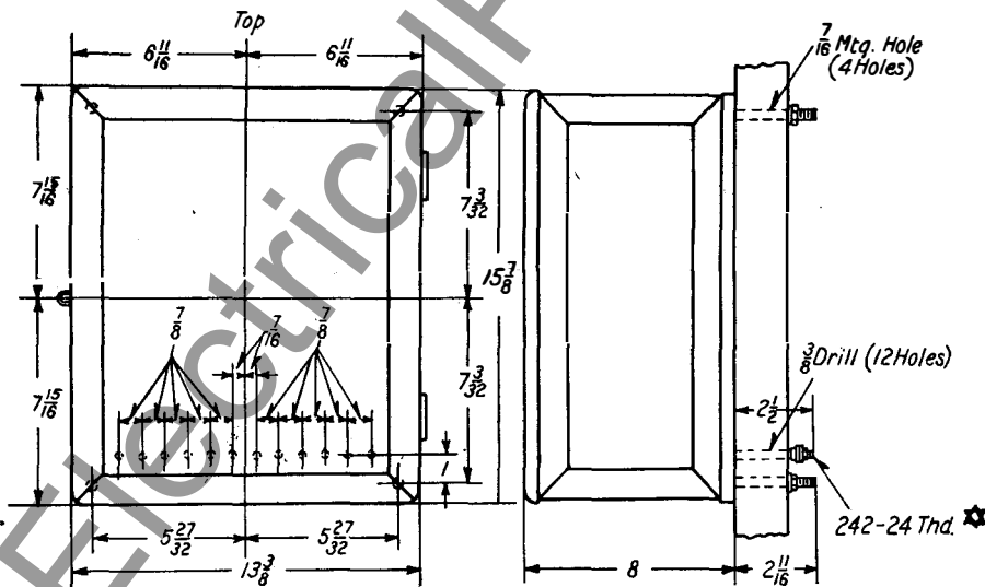
Figure 13. Outline and Drilling Plans.
