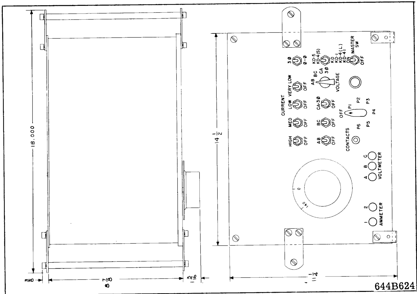
Fig. 3 Outline Drawing
