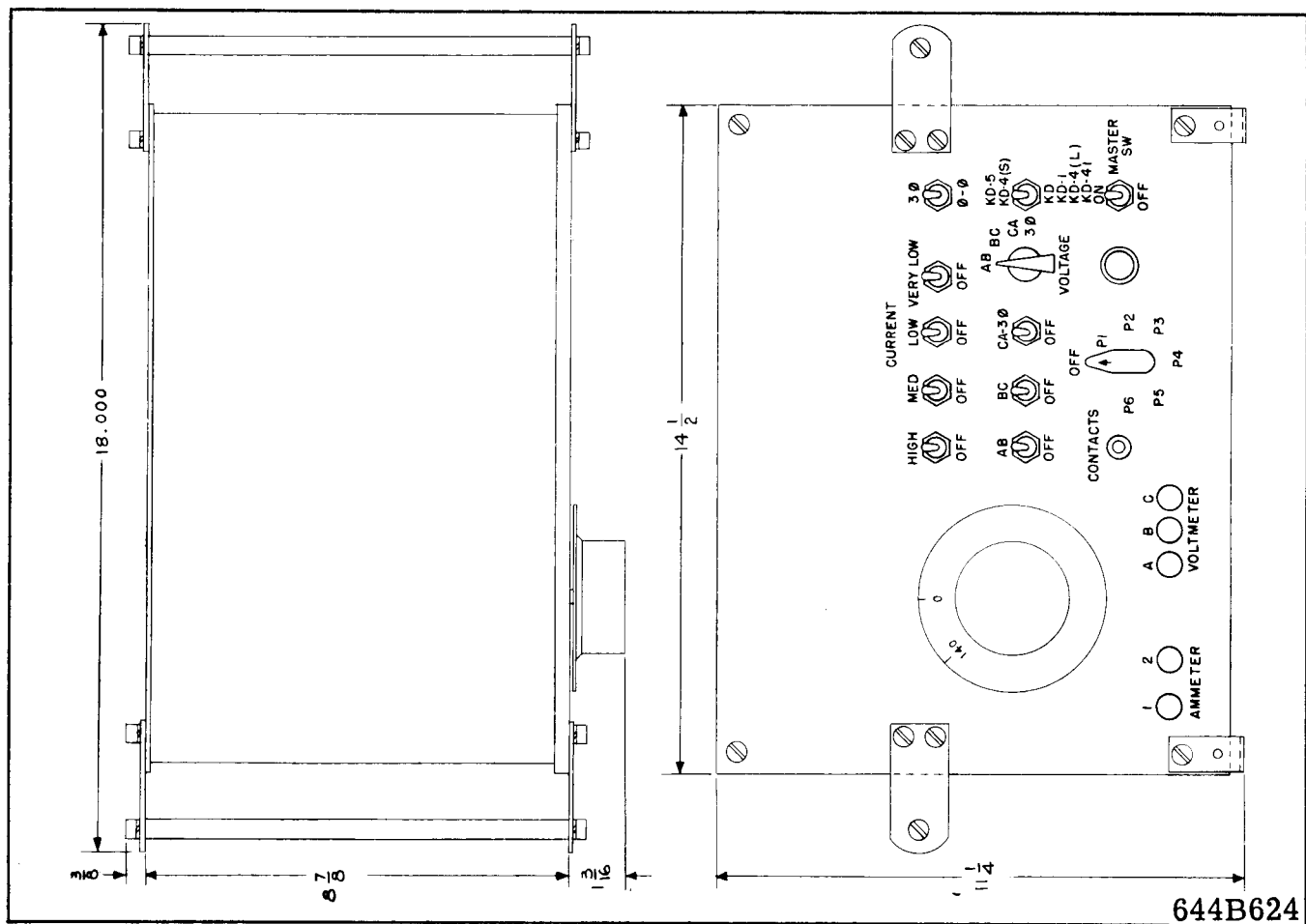
Fig. 3 Outline Drawing
