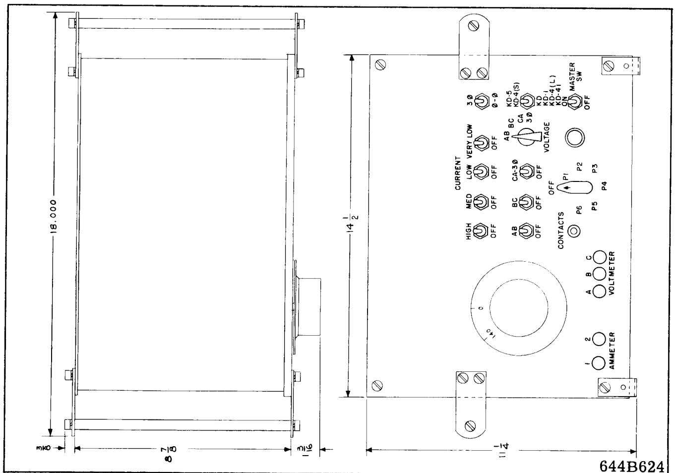
Fig. 3 Outline Drawing
