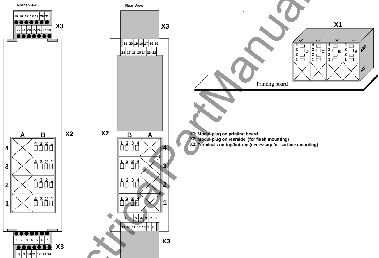
Terminal disposition at housing
