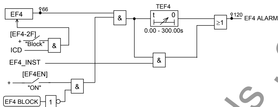
Figure 2.2.9 Earth fault Protection EF4
