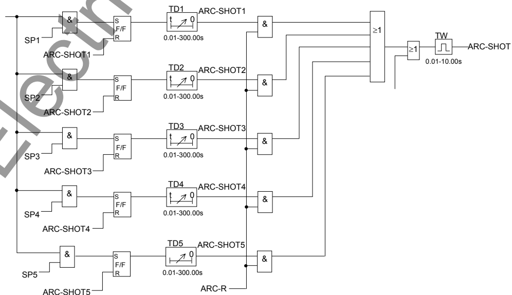
Figure 2.13.3 Autoreclosing requirement
