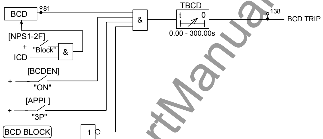
Figure 2.7.3 Broken Conductor Protection Scheme Logic
