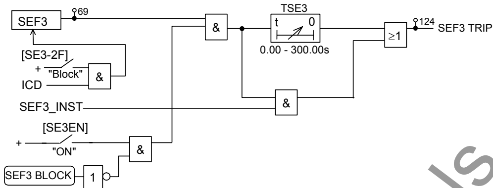
Figure 2.3.4 Definite Time SEF Protection SEF3
