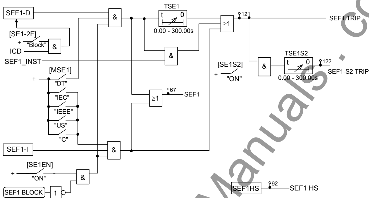
Figure 2.3.2 Inverse Time or Definite Time SEF Protection SEF1
