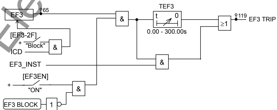
Figure 2.2.8 Earth fault Protection EF3
