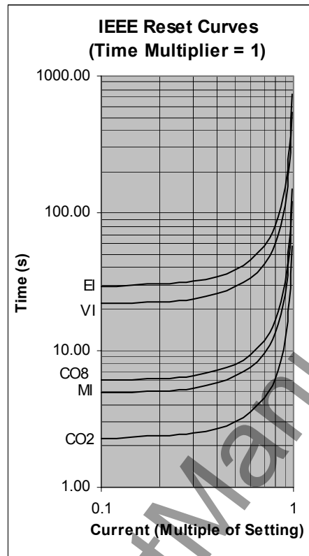
Figure 2.1.3 Dependent Time Reset Characteristics
