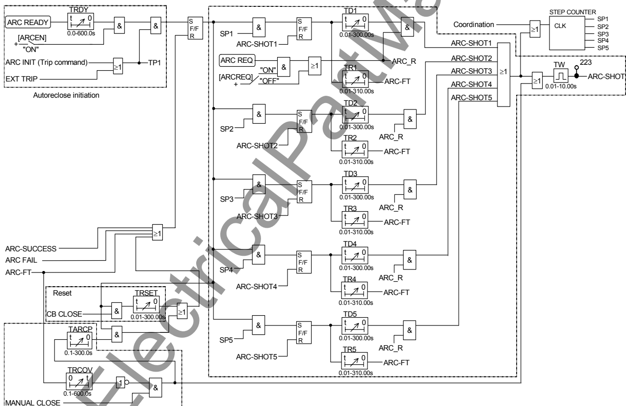
Figure 2.13.1 Autoreclose Scheme Logic
