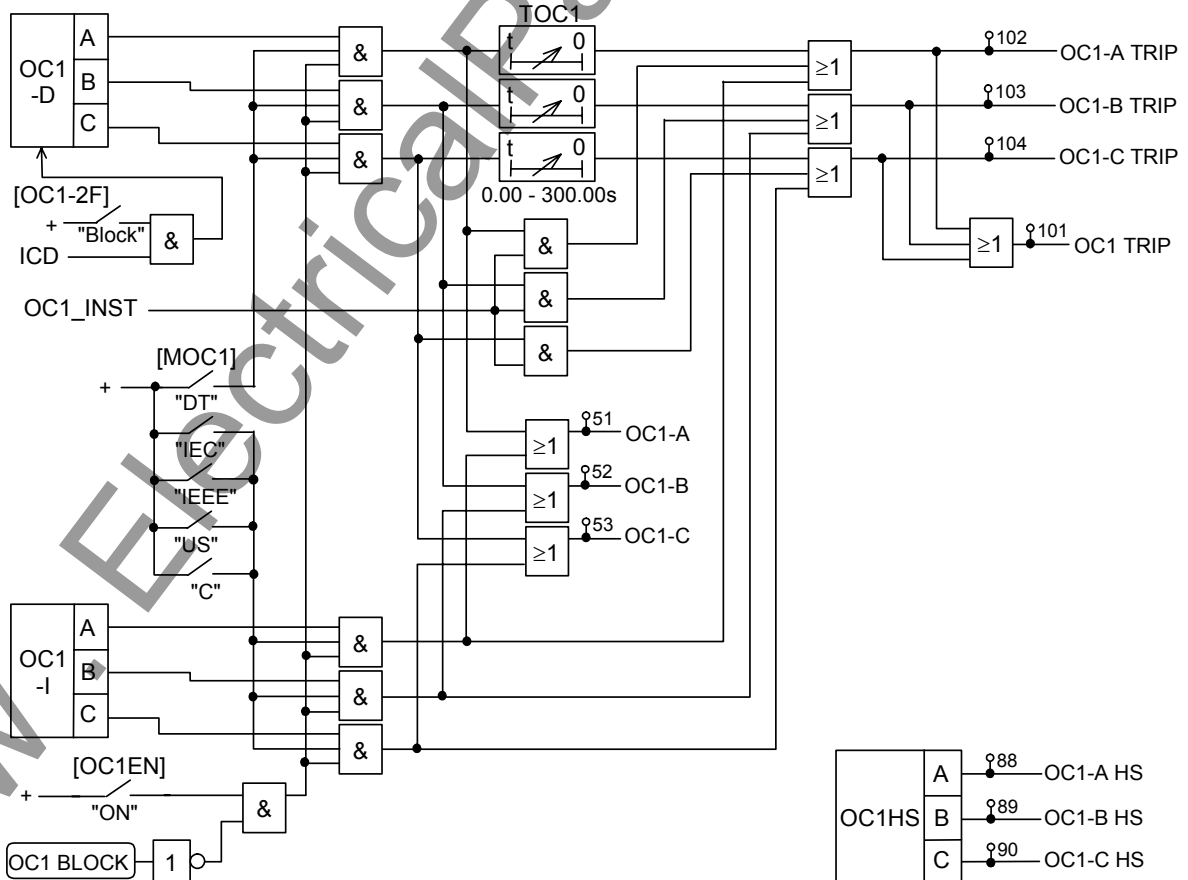
Figure 2.1.5 Phase Fault Overcurrent Protection OC1
