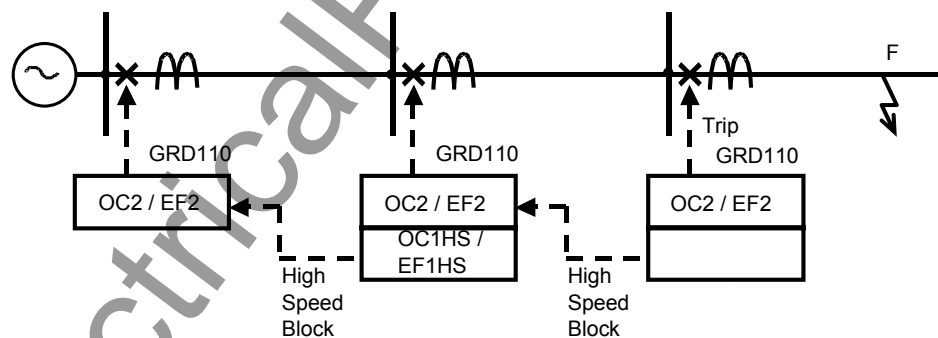
Figure 2.11.1 Blocked Overcurrent Protection
