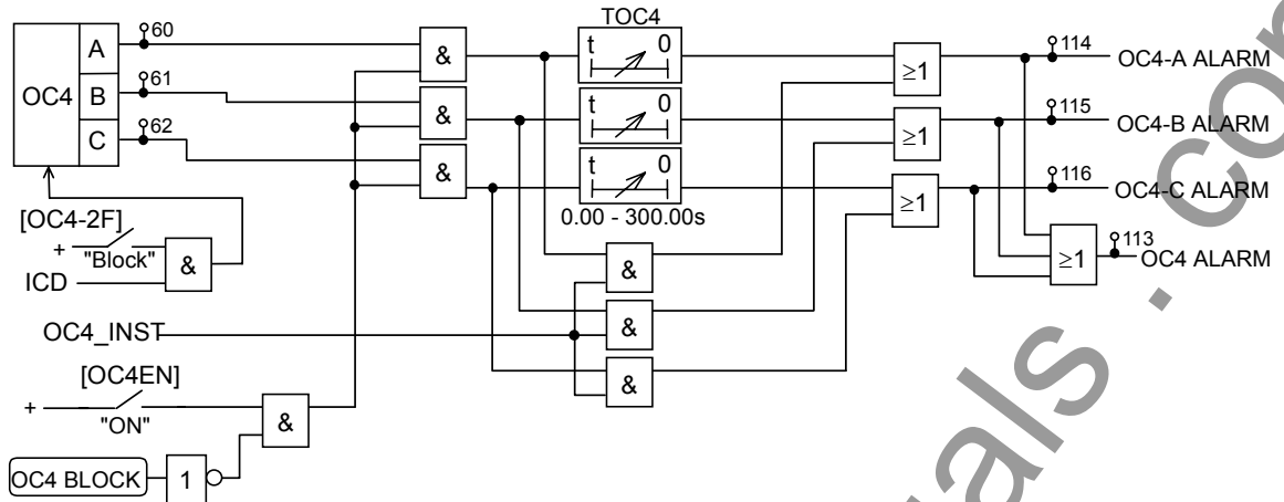
Figure 2.2.6 Phase Overcurrent Protection OC4
