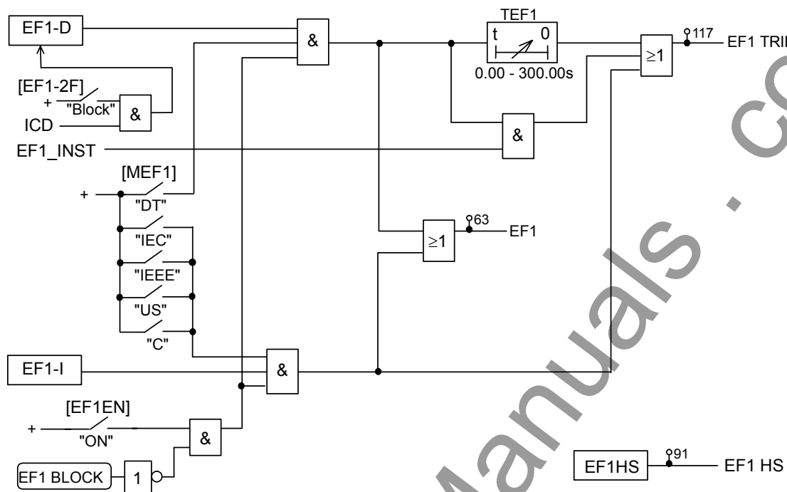
Figure 2.1.6 Earth Fault Overcurrent Protection EF1
