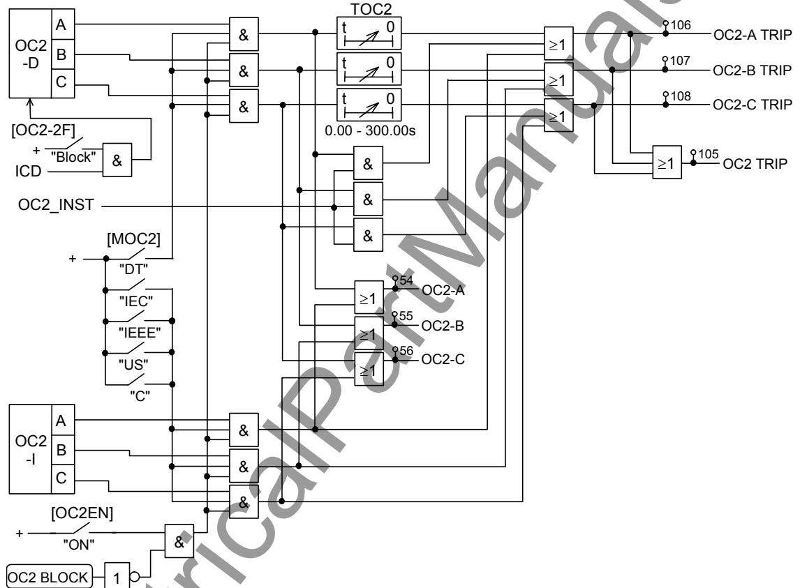
Figure 2.2.4 Phase Overcurrent Protection OC2
