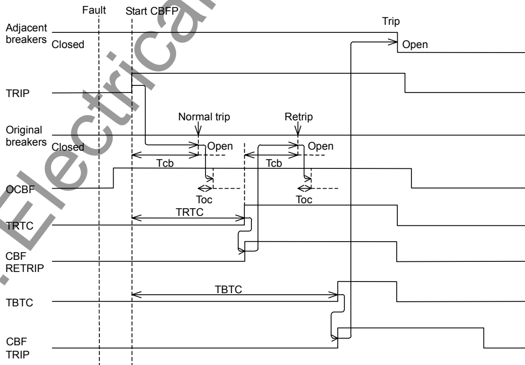
Figure 2.8.2 Sequence Diagram
