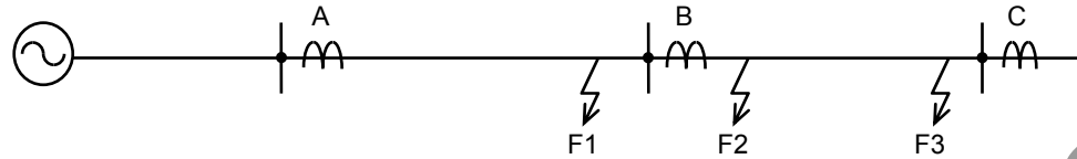
Figure 2.1.7 Current Settings in Radial Feeder
