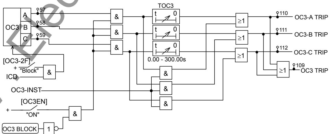
Figure 2.2.5 Phase Overcurrent Protection OC3
