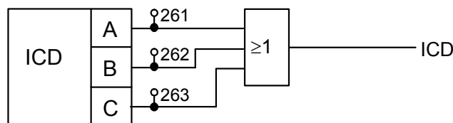
Figure 2.9.2 ICD Block Scheme
