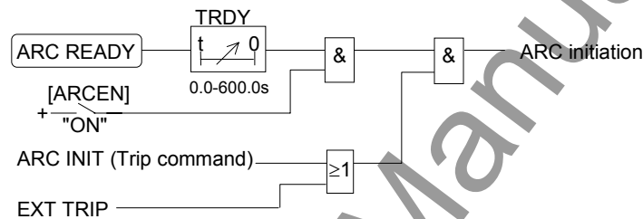
Figure 2.13.2 Autoreclose Initiation
