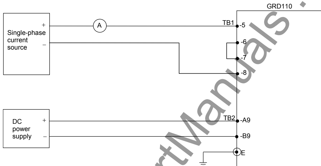
Figure 6.5.3 Test Circuit for EF and SEF Elements
