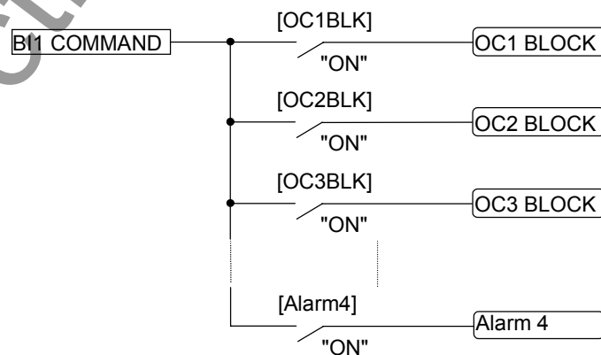
Figure 3.2.2 Function Scheme Logic
