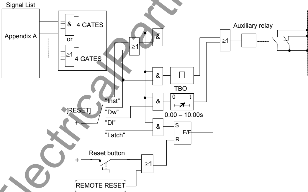
Figure 3.2.3 Configurable Output
