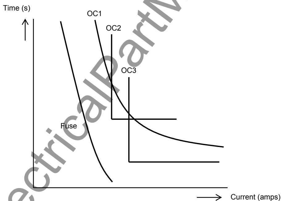
Figure 2.2.3 Staged Definite Time Protection
