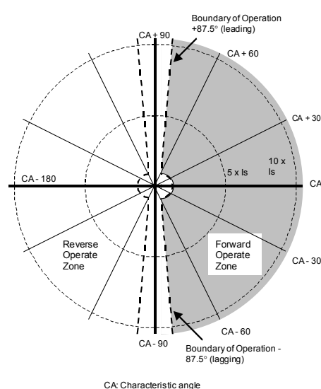
(b) Characteristic for Sensitive Earth Fault
