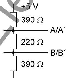
Figure 3-15 Termination of the RS485 Interface (External)
