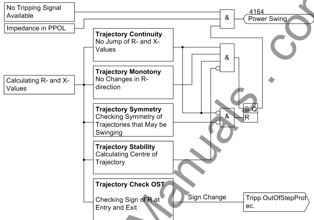
Figure 2-46 Logic diagram of power swing detection
