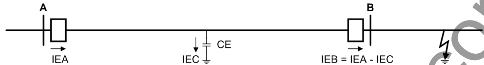
Figure 2-93 Possible current distribution during external earth fault
