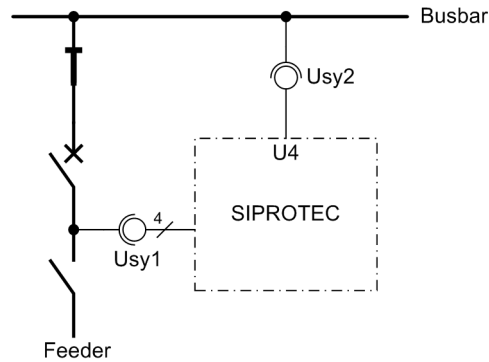
Figure 3-28 Measuring voltages for the synchronism check — Example
