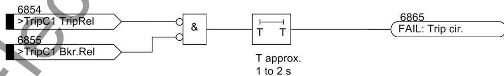
Figure 2-157 Logic diagram of the trip circuit monitoring with two binary inputs
