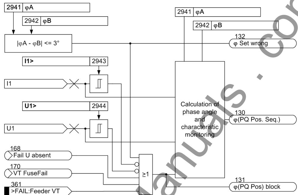
Figure 2-155 Logic of the Positive Sequence System Phase Angle Monitoring
