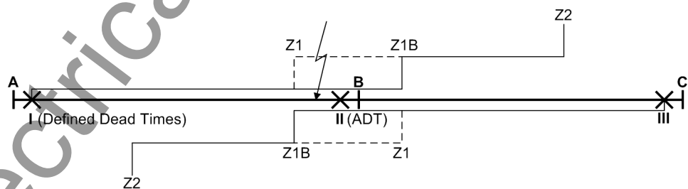
Figure 2-109 Example of adaptive dead time (ADT) A, B, C Busbars I, II, III Relay locations X Tripped circuit breakers
