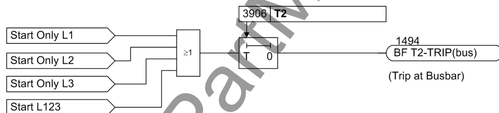
Figure 2-138 Single-stage breaker failure protection with common phase initiation
