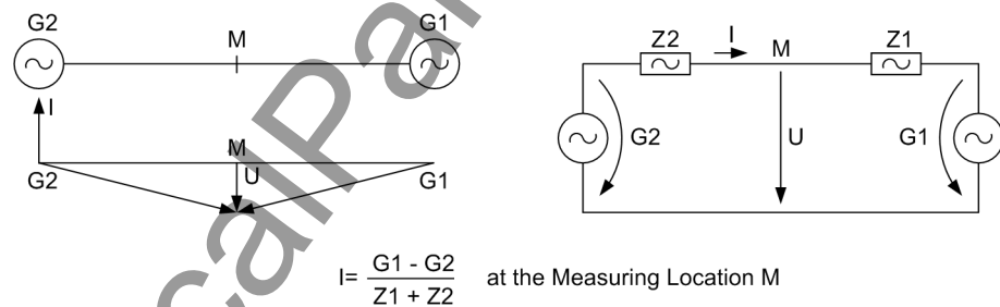
Figure 2-41 Power swing
