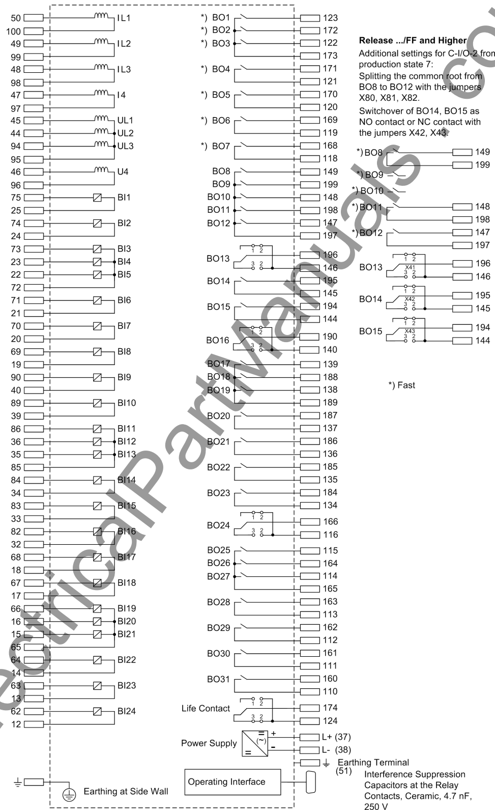
Figure A-13 General diagram 7SA522*-*H (panel surface mounting; size 1/1)
