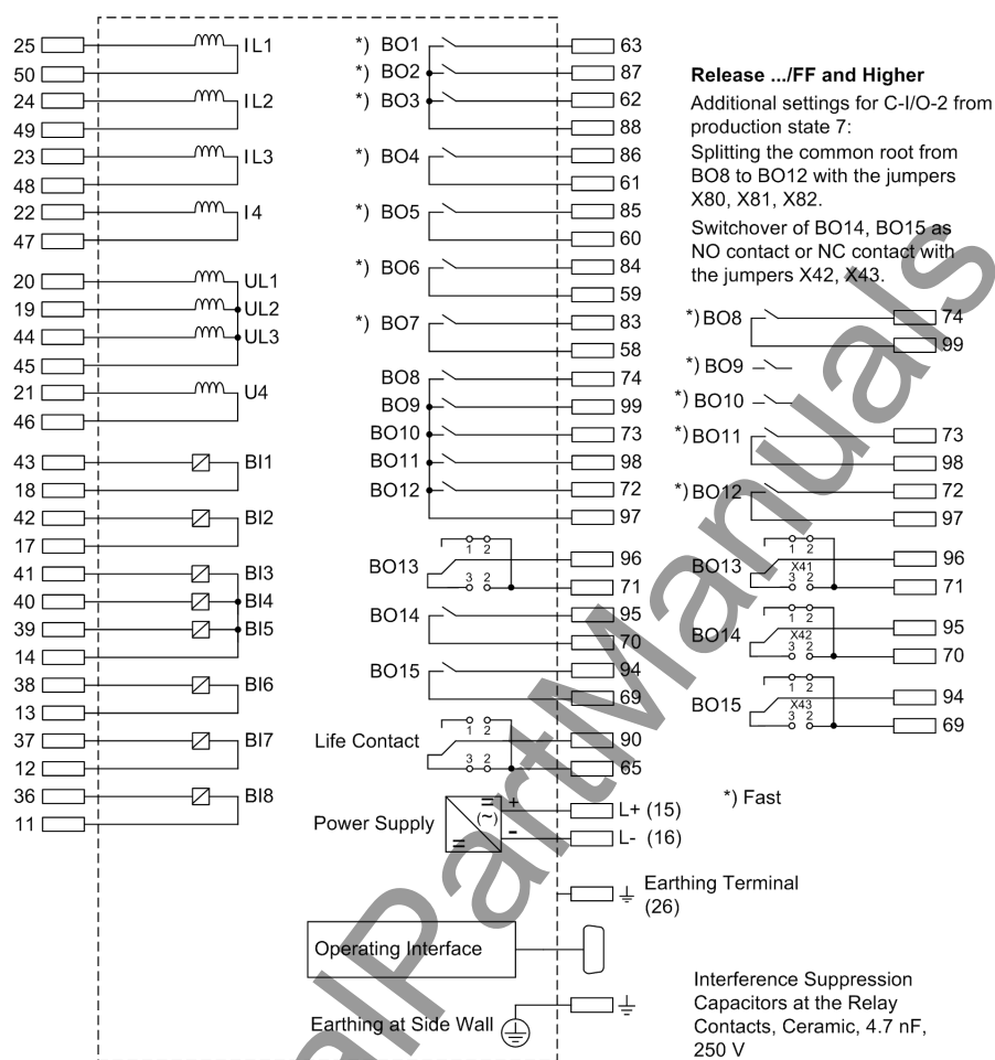
Figure A-8 General diagram 7SA522*-*E (panel surface mounting; size 1/2 )
