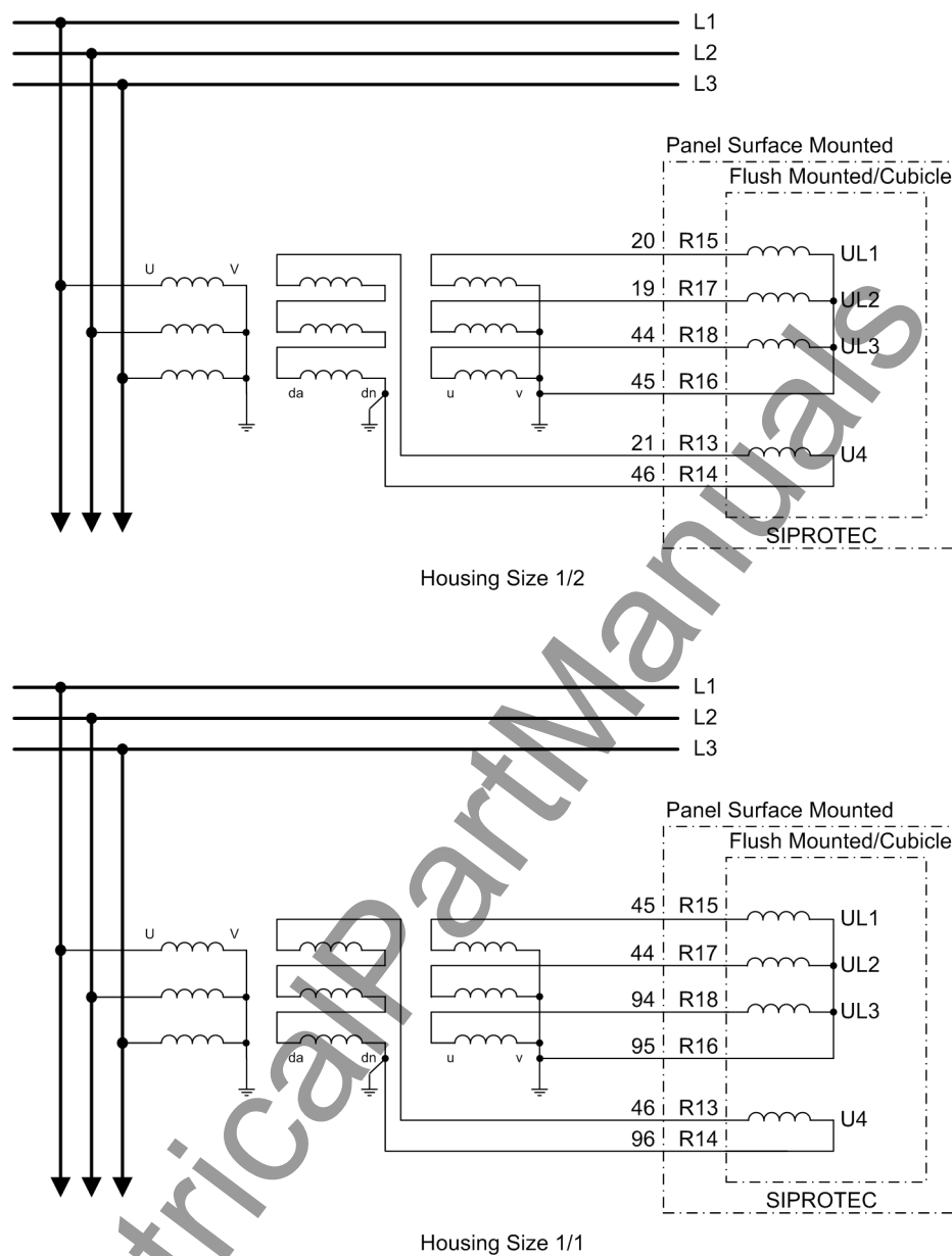
Figure A-22 Voltage connections to three wye-connected voltage transformers with additional open-delta windings (e-n-winding)
