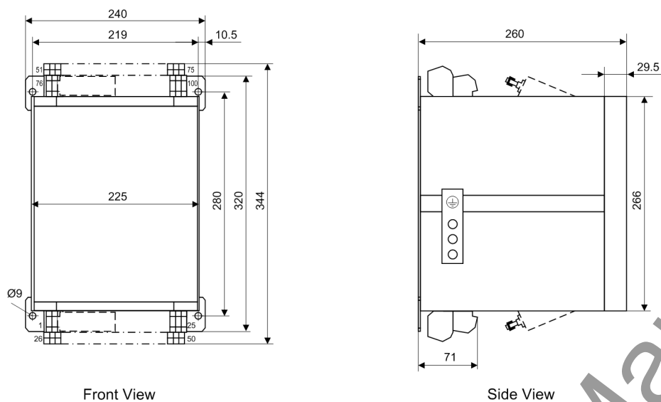
Figure 4-9 Dimensions of a device for panel surface mounting (size 1\frac{1}{2} )
