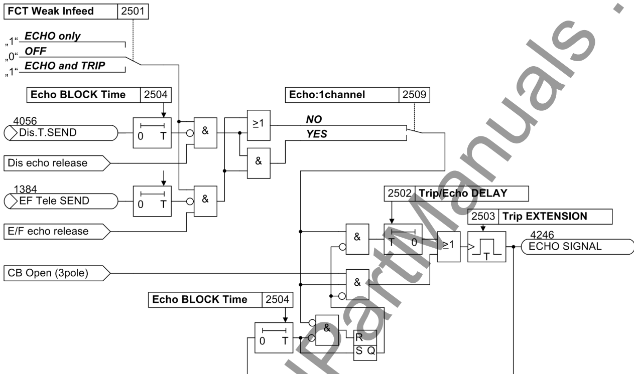
Figure 2-95 Logic diagram of the echo function with teleprotection
