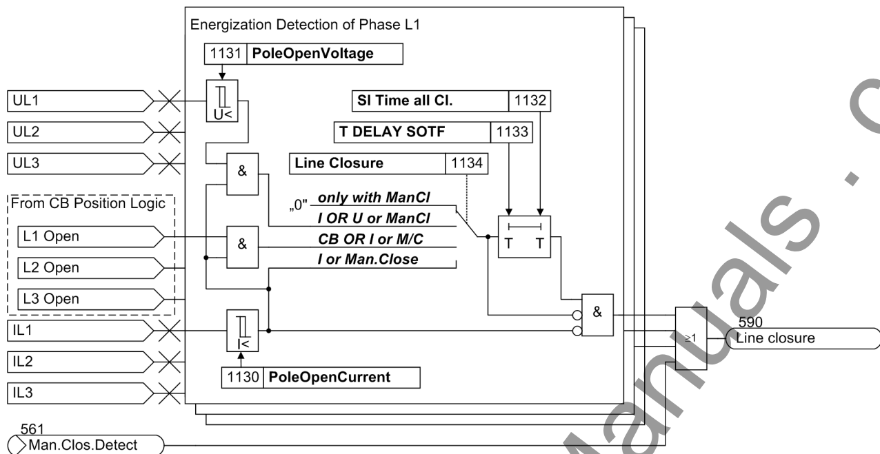
Figure 2-163 Generation of the energization signal
