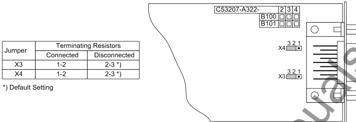
Figure 3-14 Location of the jumpers for configuring the PROFIBUS and DNP 3.0 interface terminating resistors
