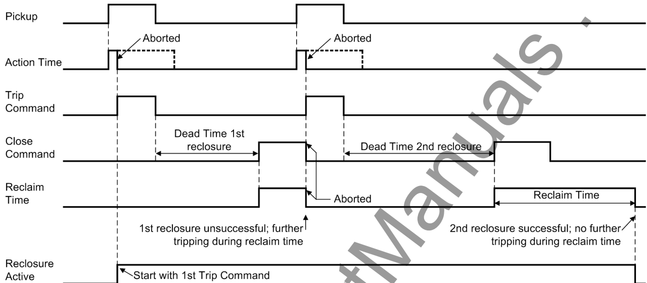
Figure 2-106 Timing diagram of a double-shot reclosure with action time (2nd reclosure successful)
