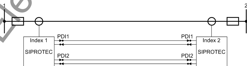
Figure 2-50 Distance protection for two ends with two 7SA522 devices with two protection data interface each (transmitter/ receiver)
