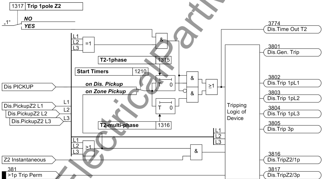
Figure 2-37 Tripping logic for the 2nd zone
