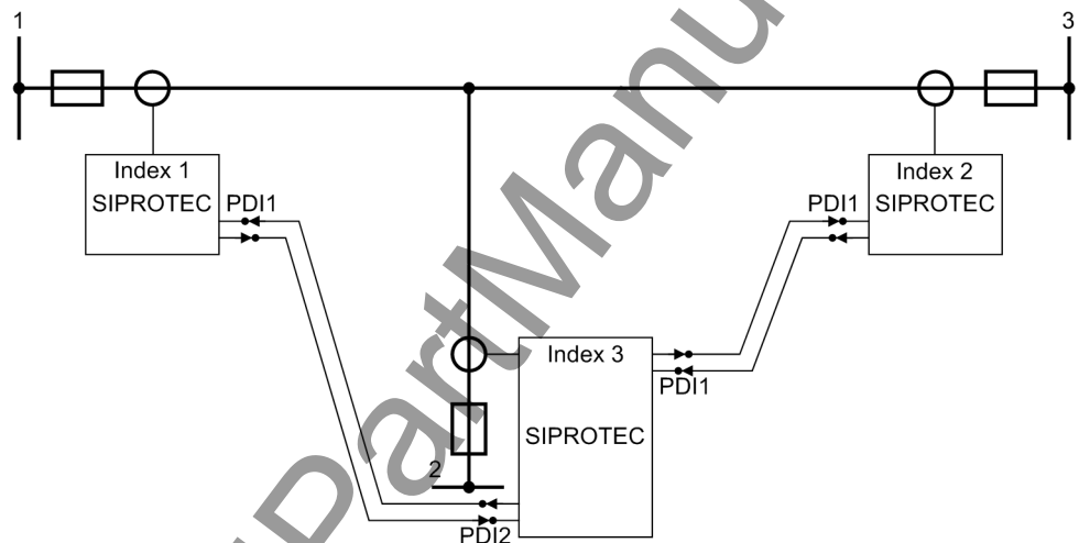
Figure 2-51 Distance protection for three ends with three 7SA522, chain topology
