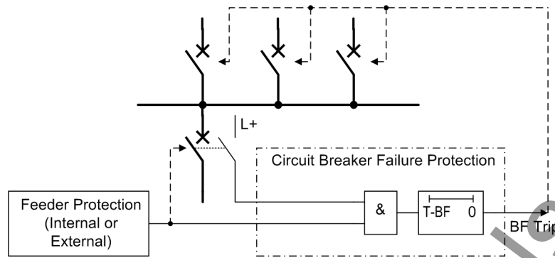
Figure 2-130 Simplified function diagram of circuit breaker failure protection controlled by circuit breaker auxiliary contact
