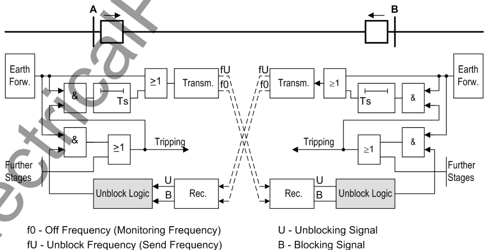
Figure 2-86 Operation scheme of the directional unblocking method
