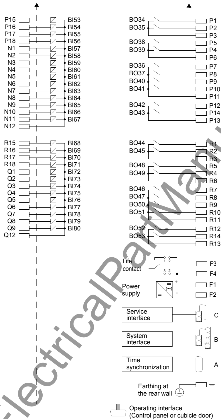
Figure 19 General diagram 6MD613 (panel surface mounting)
