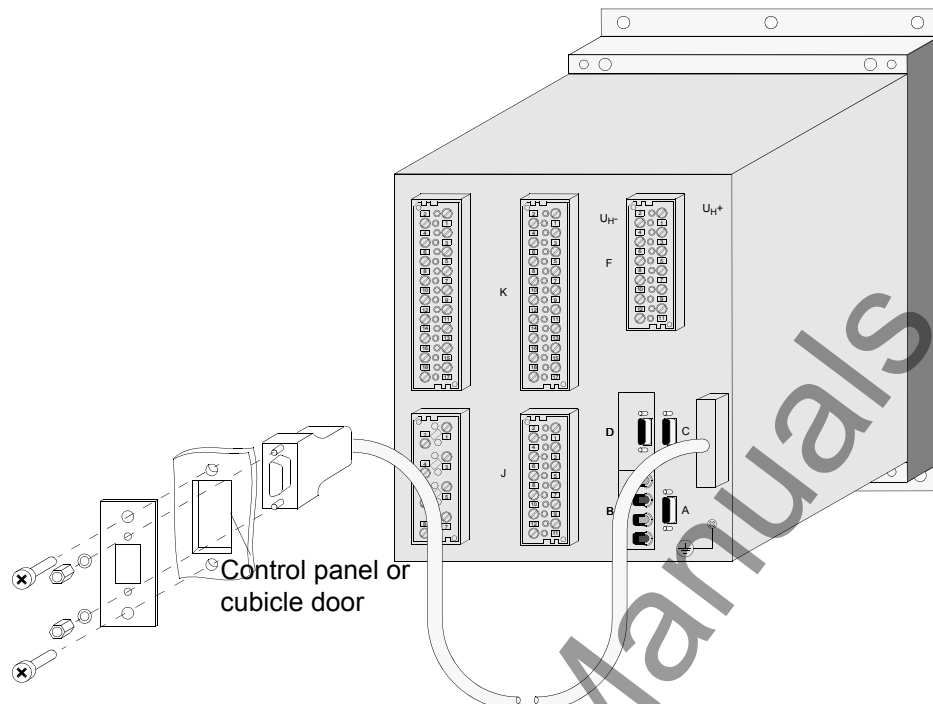
Figure 10 Plugging the D-subminiature connector of the dongle cable into the control panel or cubicle door
