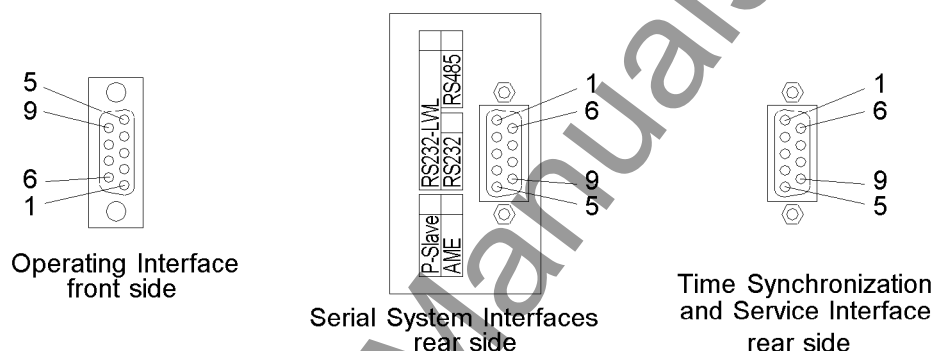
Figure 3-12 9-pin subminiature sockets
