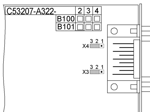
Figure 3-7 Position of the jumpers for configuration of termination resistors of the PROFIBUS FMS and PROFIBUS DP interface
