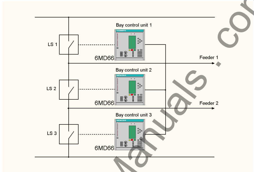
Figure 2-27 1 1/2-Circuit breaker method, disconnector and earth electrode not shown
