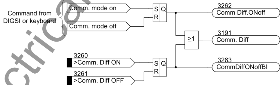
Figure 2-11 Logic diagram of the commissioning mode
