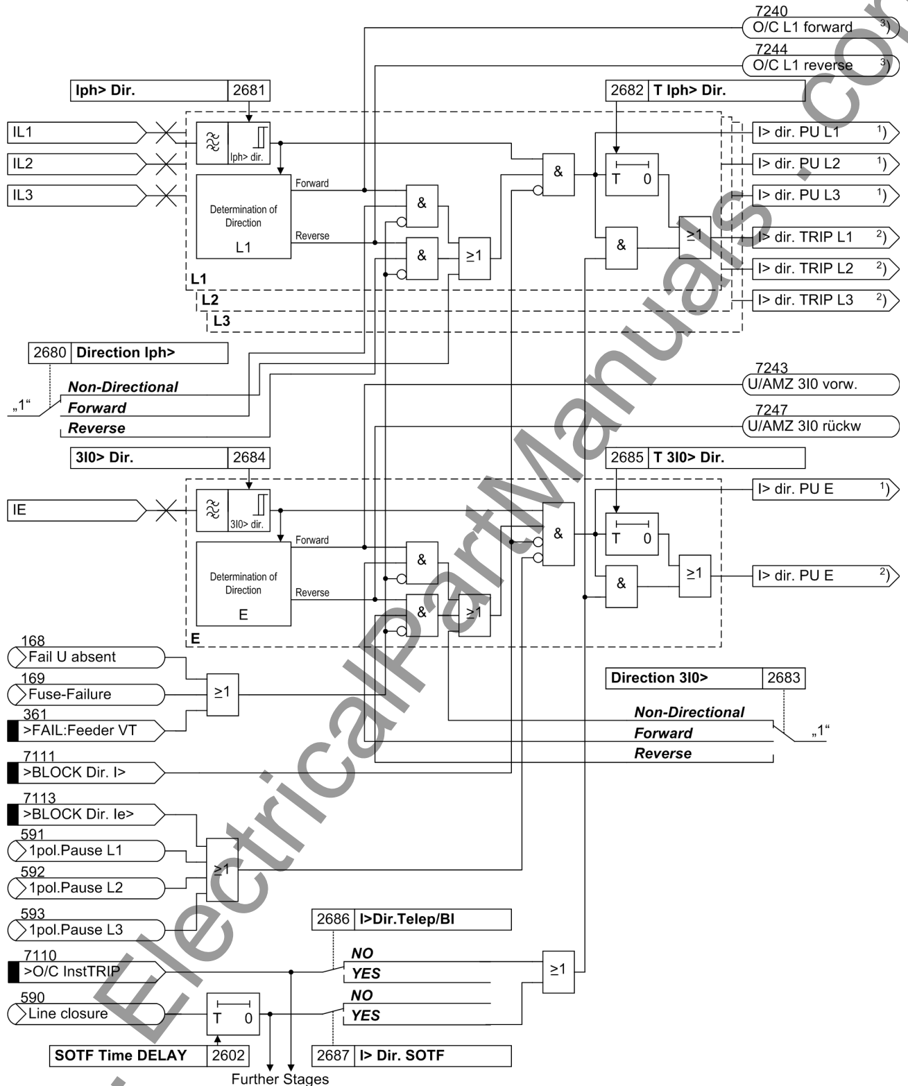
Figure 2-40 Logic diagram of the I> stage
