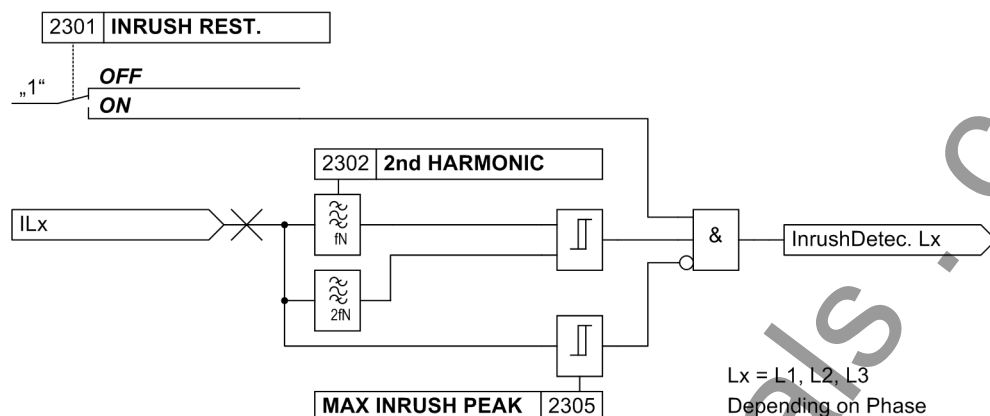
Figure 2-18 Logic diagram of the inrush restraint for one phase
