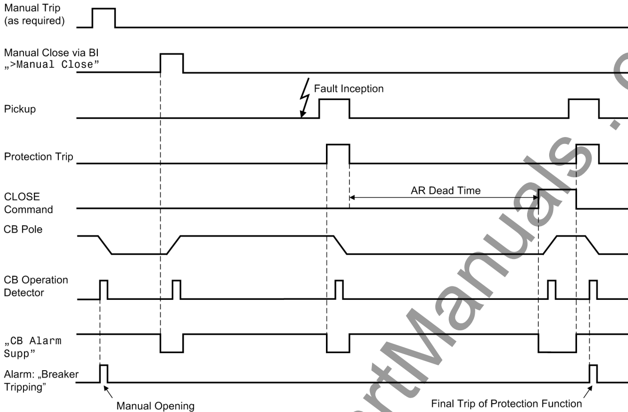
Figure 2-103 Breaker tripping alarm suppression — sequence examples
