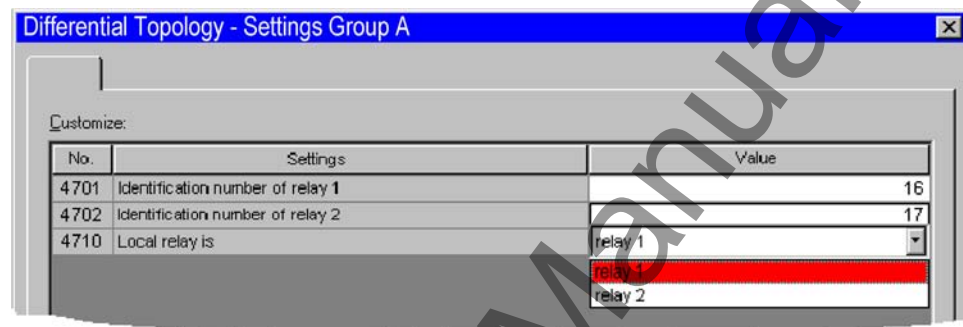
Figure 2-14 Differential protection topology for 2 ends with 2 devices — example
