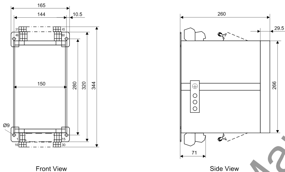
Figure 4-7 Dimensions of a device for panel surface mounting (size \frac{1}{3} )
