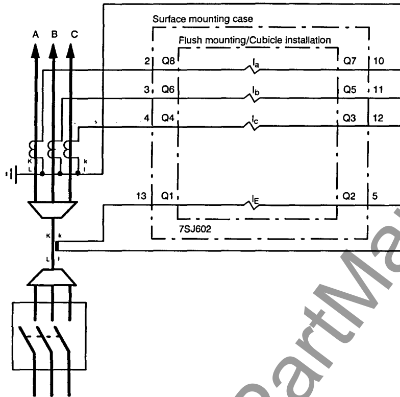
Figure B.3 3 c.t. connection with separate residual c.t. for ground currents
