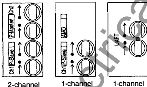
Figure 2.11 Optical interfaces with protective caps
