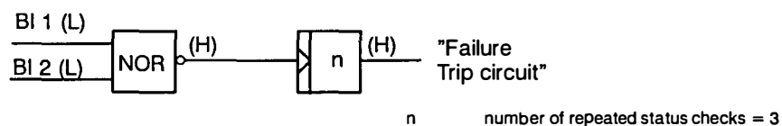
Figure 4.10 Principle of trip circuit supervision with two binary inputs
