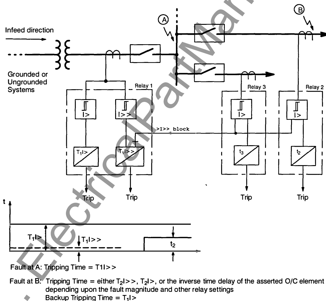
Figure 4.5 Busbar protection using reverse interlocking principle – scheme
