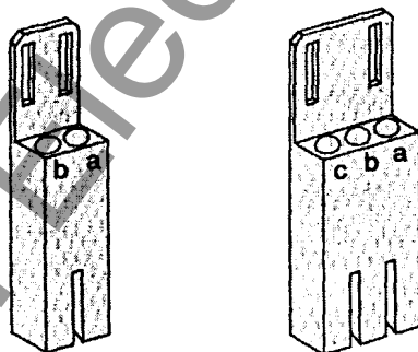
Figure 2.6 2-pin and 3-pin terminal box
