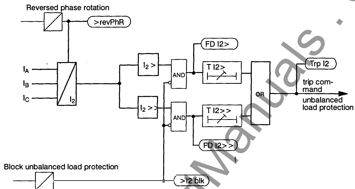
Figure 4.7 Logic diagram of the unbalanced load protection
