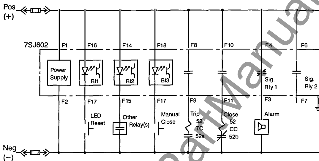
Figure 2.19 Typical DC schematic; 7SJ602 configured with auto-reclosing.
