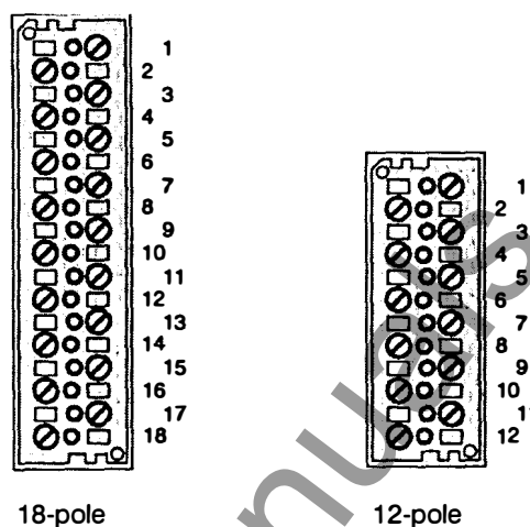
Figure 2.7 Connection modules for screwed terminals (voltage) – rear view
