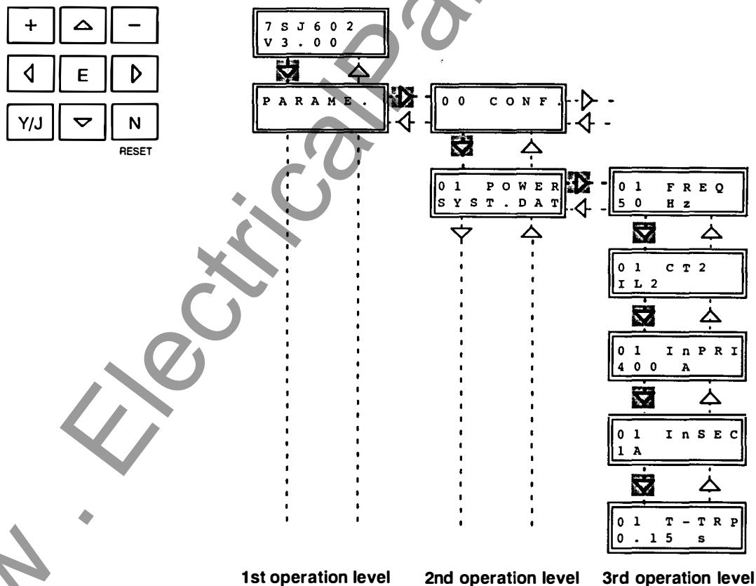
Figure 6.2 Selection of the power system data
