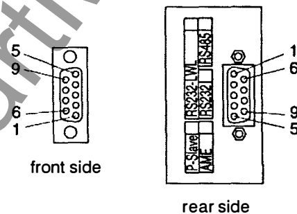
Figure 2.12 9-pin D-subminiature terminal
