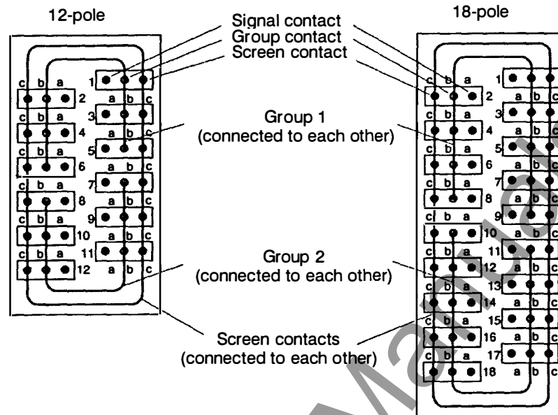
Figure 2.5 Scheme of the contact set
