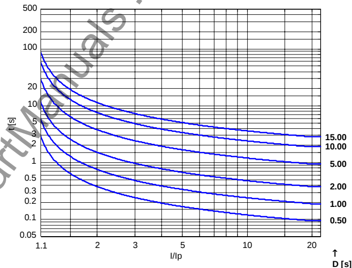
Figure 2-17 Pickup characteristic as per ANSI, moderately inverse (M INV)
