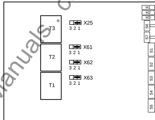
Figure 2-6 Jumper location on the module
