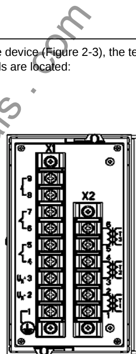
Figure 2-3 Terminal blocks on the rear of the 7SJ46
