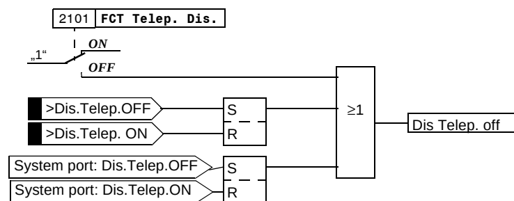
Figure 6-49 Switching on and off of the teleprotection
