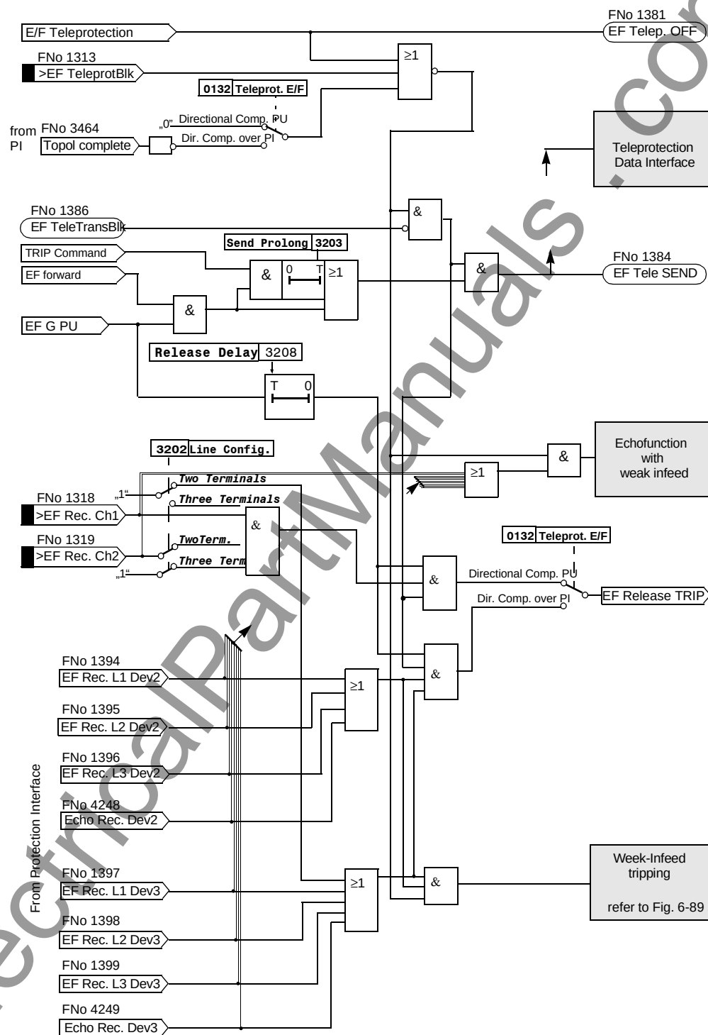
Figure 6-80 Logic diagram of the directional comparison scheme with protection interface (for device 1)
