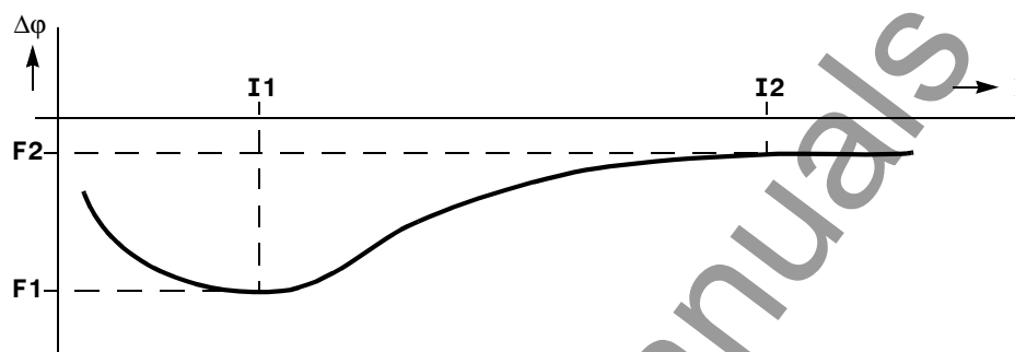
Figure 6-100 Settings for the phase angle correction
