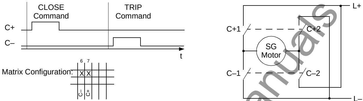
Figure 5-10 Double command motor control (anti-clockwise rotation / clockwise rotation) via two power relays with two contacts each
