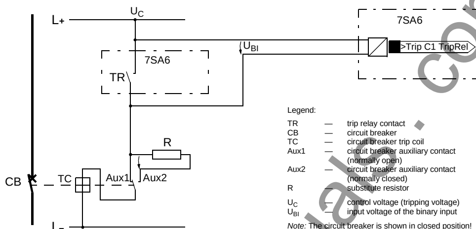
Figure 6-146 Operating principle of the trip circuit supervision with one binary input
