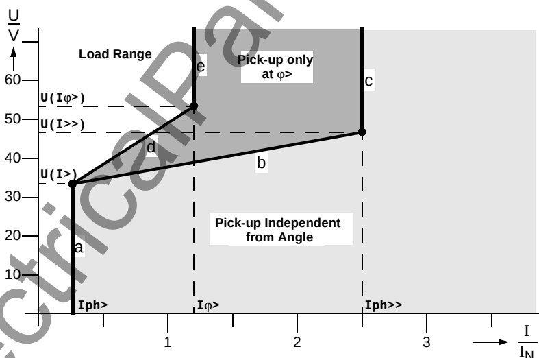
Figure 6-21 Parameters of U/I/ \phi pick-up
