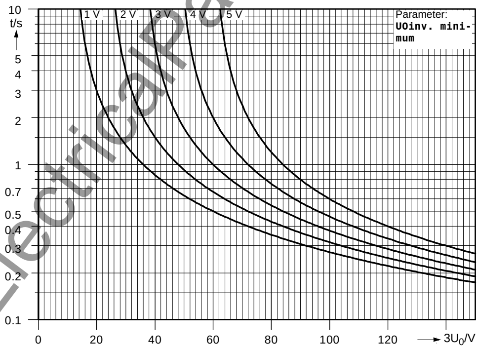
Figure 10-5 Trip time characteristics of the zero sequence voltage protection U_{0inv} .
