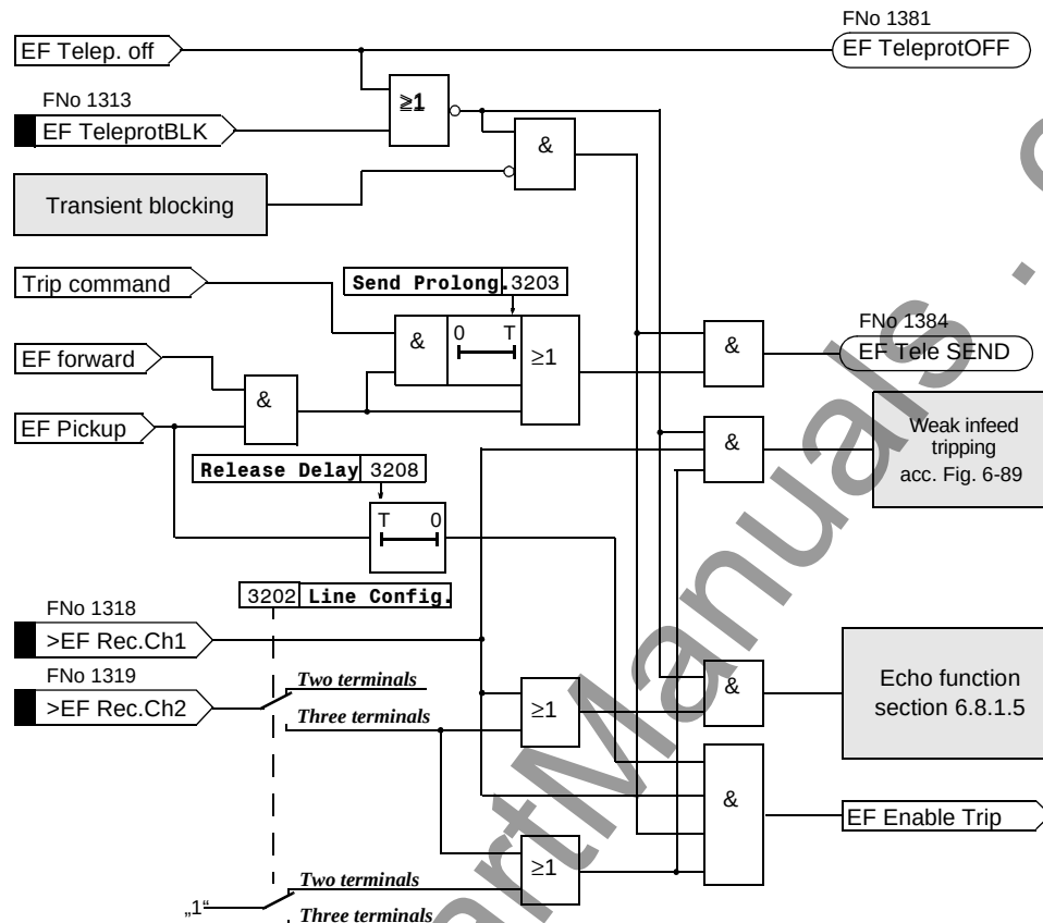
Figure 6-79 Logic diagram of the directional comparison scheme (one line end)
