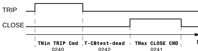
Figure 6-157 Trip/Close test cycle
