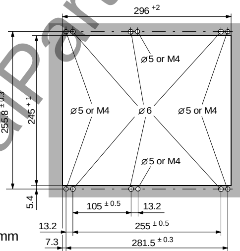
Panel cut-out
