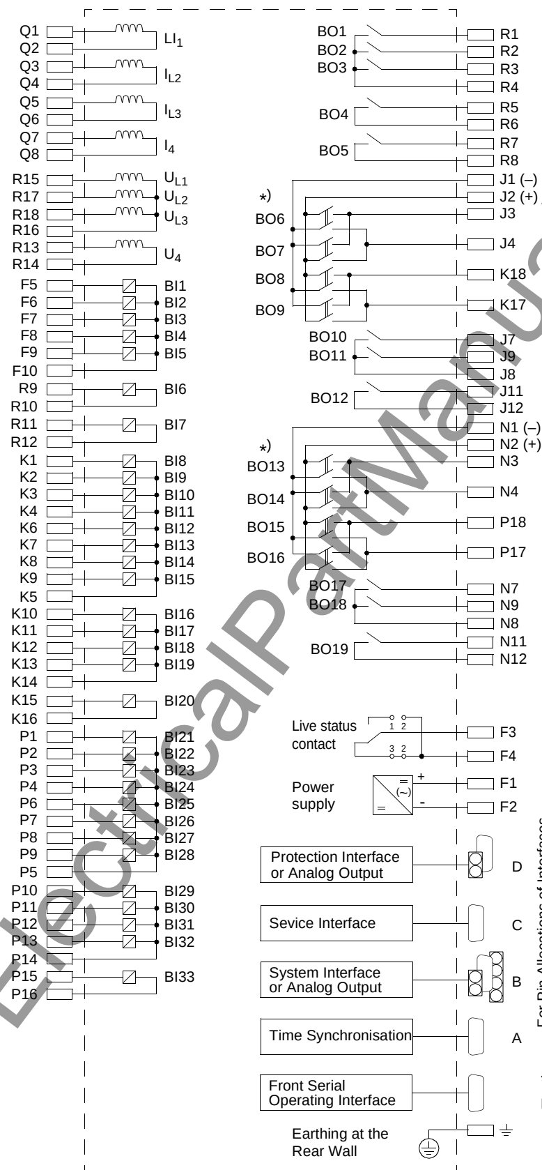
Figure A-10 General Diagram 7SA6*2*-*C/L (panel flush mounted or cubicle mounted)
