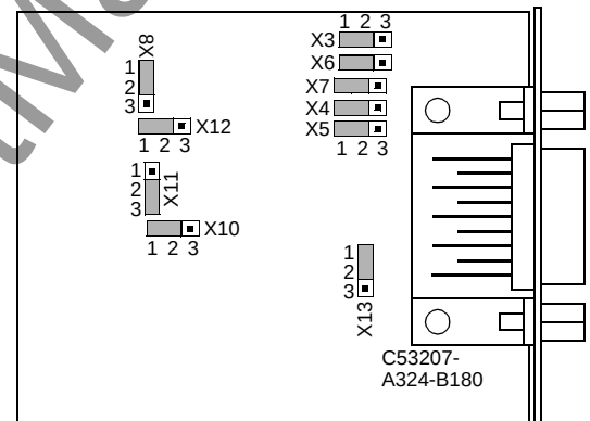
Figure 8-20 Location of the jumpers for configuration of RS232
