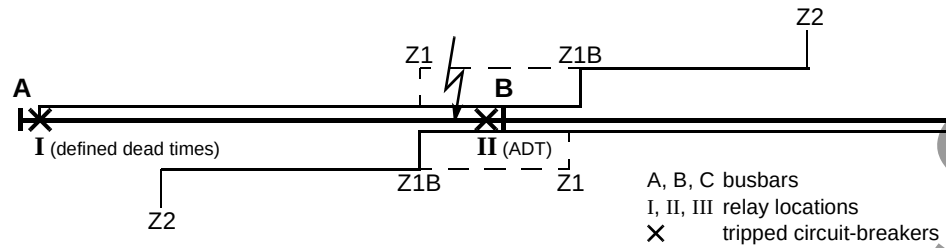
Figure 6-104 Example of adaptive dead time (ADT)
