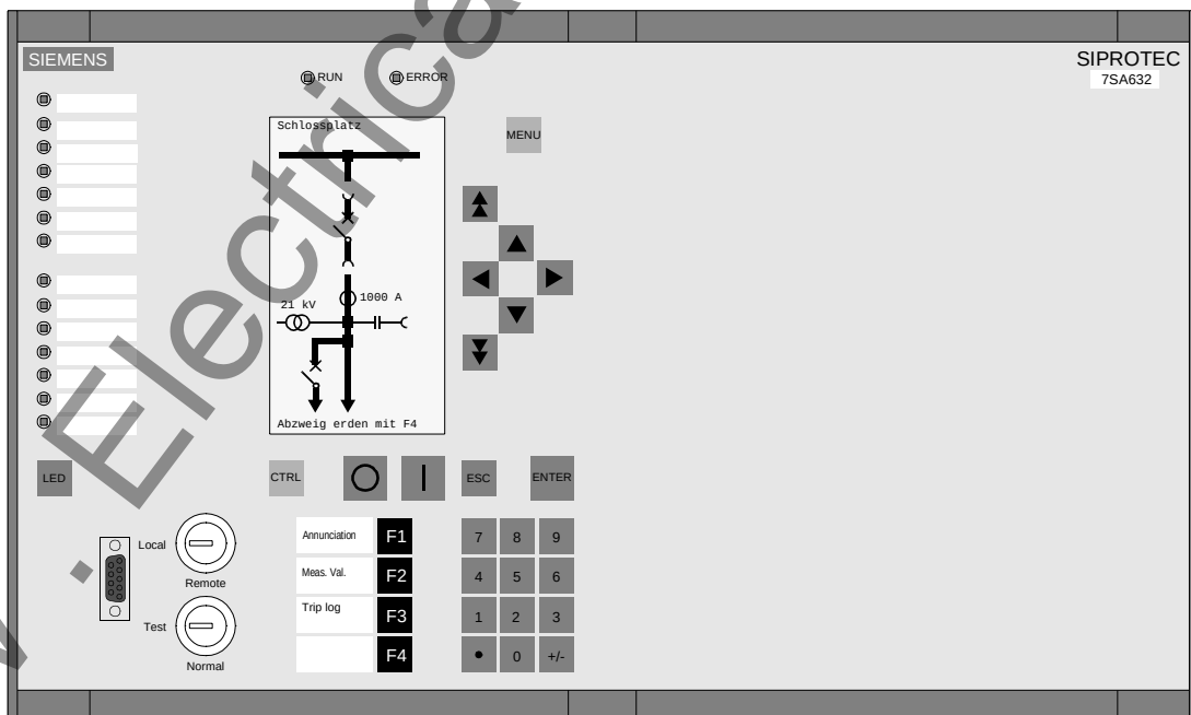
Figure 2-5 Front view of a 7SA63, housing size 1\frac{1}{1} , for panel flush mounting or cubicle mounting
