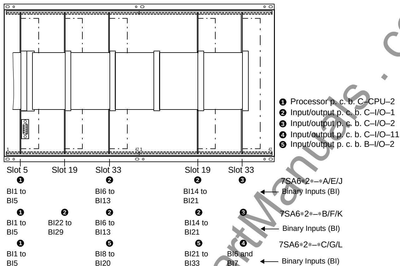
Figure 8-11 Front view of the device with housing size 1\frac{1}{2} after removal of the front cover (simplified and scaled down).
