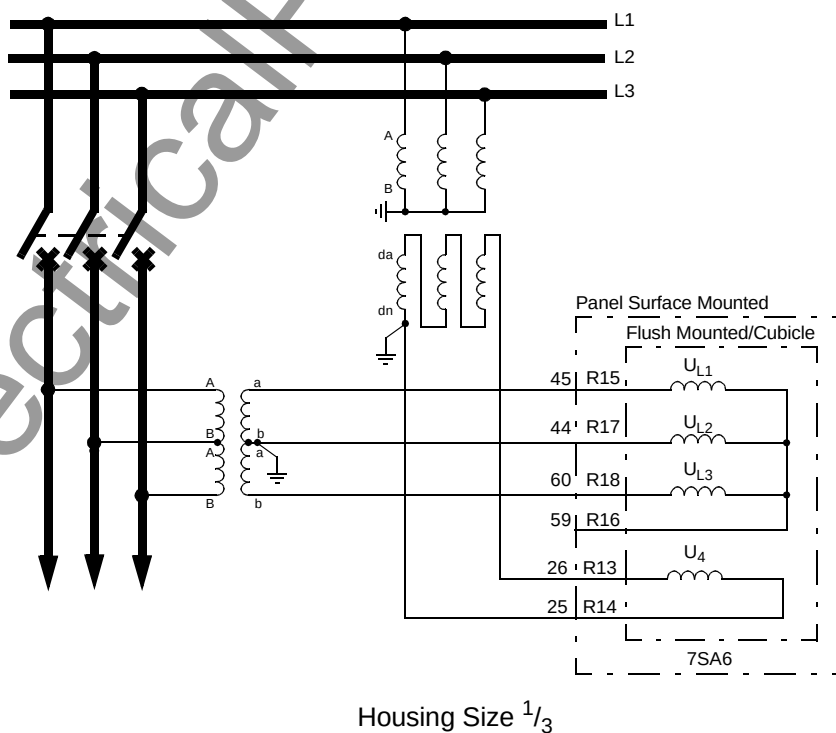
Figure A-44 Voltage connections to two V-connected voltage transformers with additional open-delta windings (da-dn-winding) from the busbar
