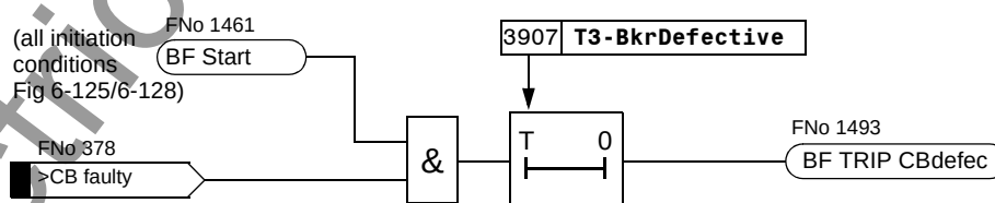
Figure 6-132 Circuit breaker not operational
