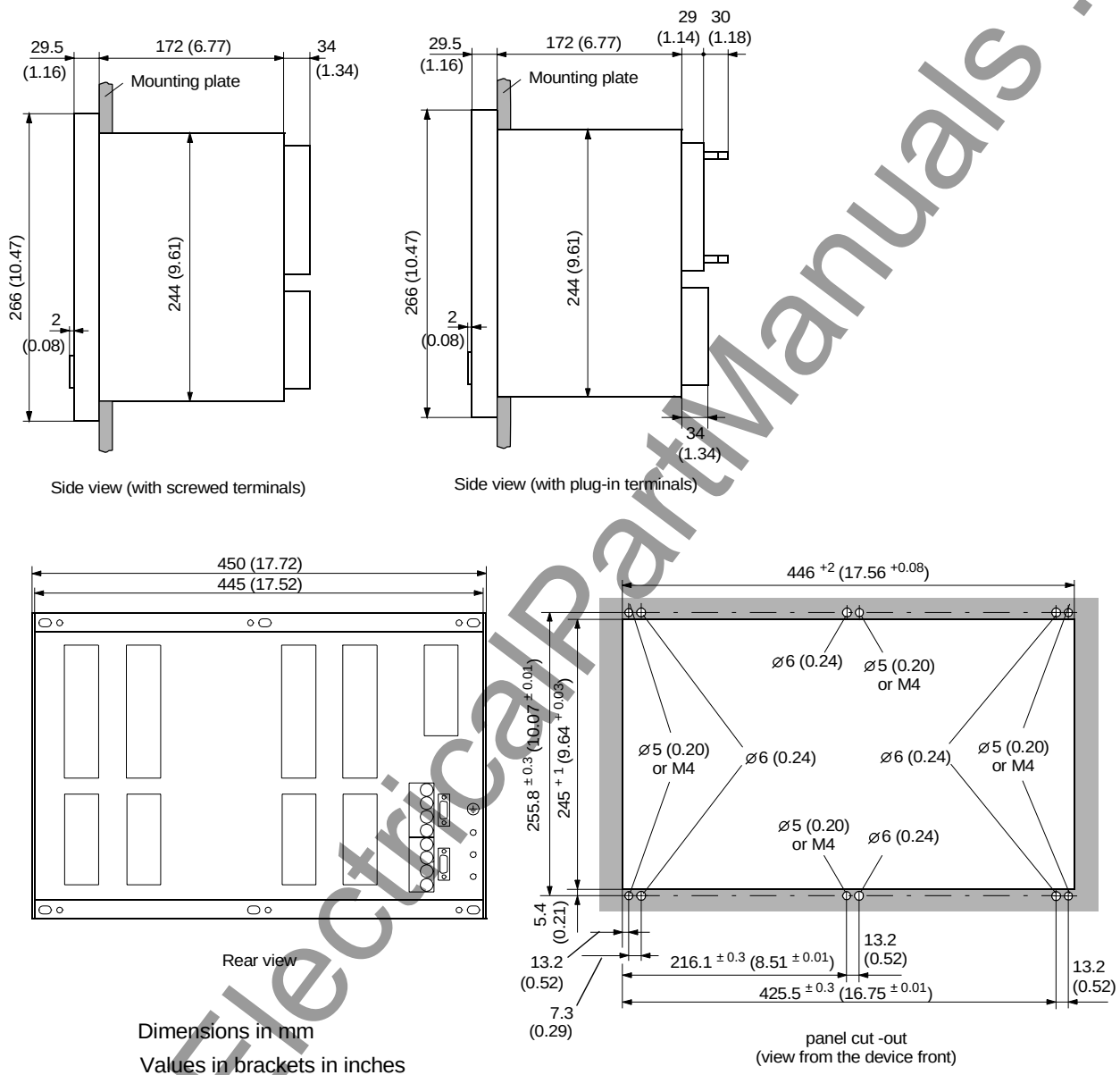
Figure 10-10 Dimensions 7SA6 for panel flush mounting or cubicle installation (size 1\frac{1}{2} x 19")
