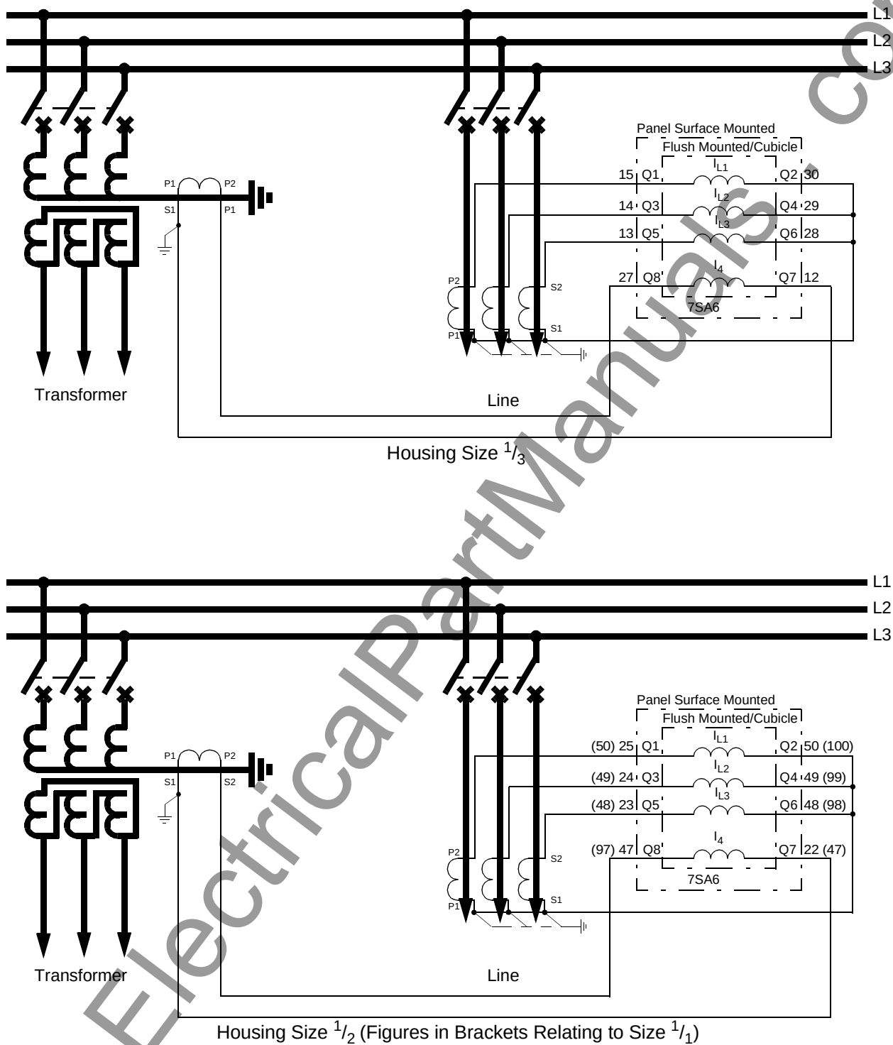
Figure A-38 Current connections to three current transformers and earth current from the star-point connection of an earthed power transformer (for directional-controlled earth fault protection)
