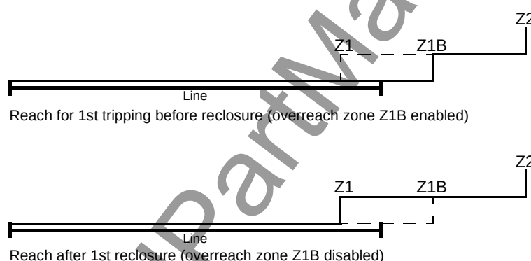
Figure 6-102 Reach control, before the first reclosure, in the distance protection
