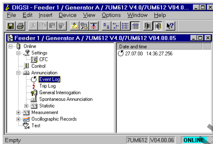
Figure 7-4 Selection of operational messages in DIGSI® 4 — example
