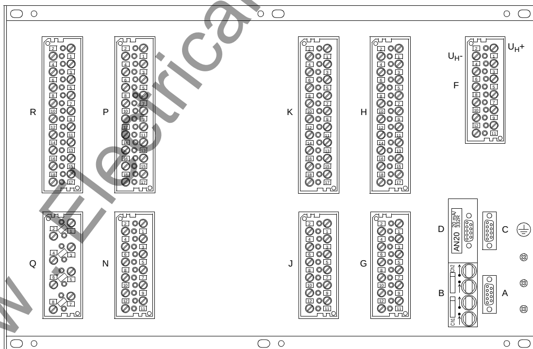
Figure 2-8 Rear view of a 7SA6, housing size 1\frac{1}{1} (terminal arrangement example only)
