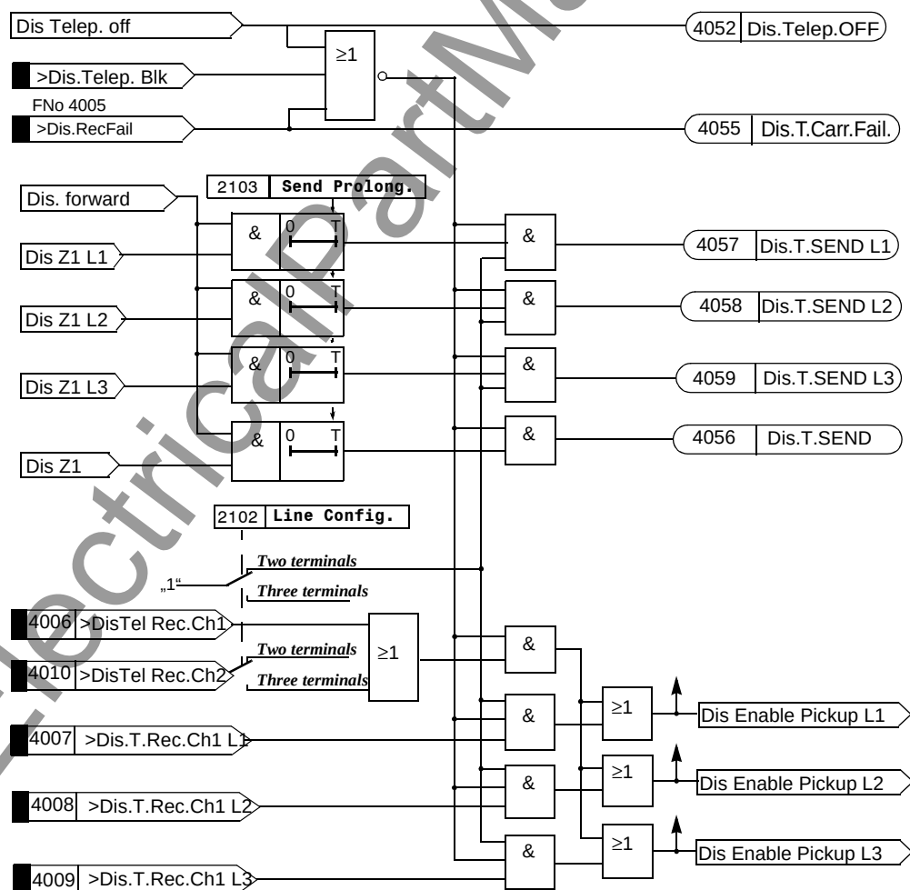
Figure 6-51 Logic diagram of the permissive underreach transfer trip (PUTT) scheme with pick-up (one line end)
