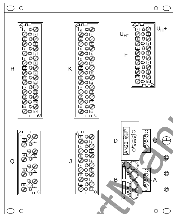
Figure 2-7 Rear view of a 7SA6, housing size 1\frac{1}{2} (terminal arrangement example only)
