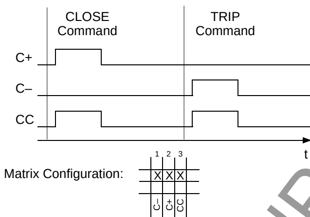
Figure 5-6 Double command with single contacts plus common contact
