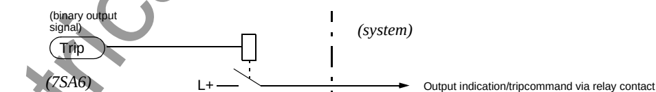
Figure 5-2 Output indication (OUT)
