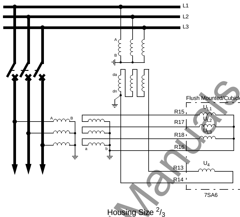
Figure A-43 Voltage connections to three Wye-connected voltage transformers with additional open-delta windings (da-dn-winding) from the busbar
