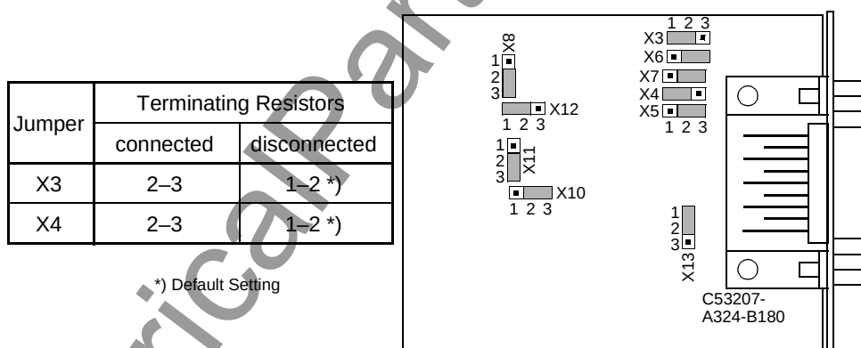
Figure 8-21 Location of jumpers for the configuration of terminating resistors of interface RS485
