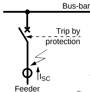
Figure 6-133 End fault between circuit breaker and current transformers
