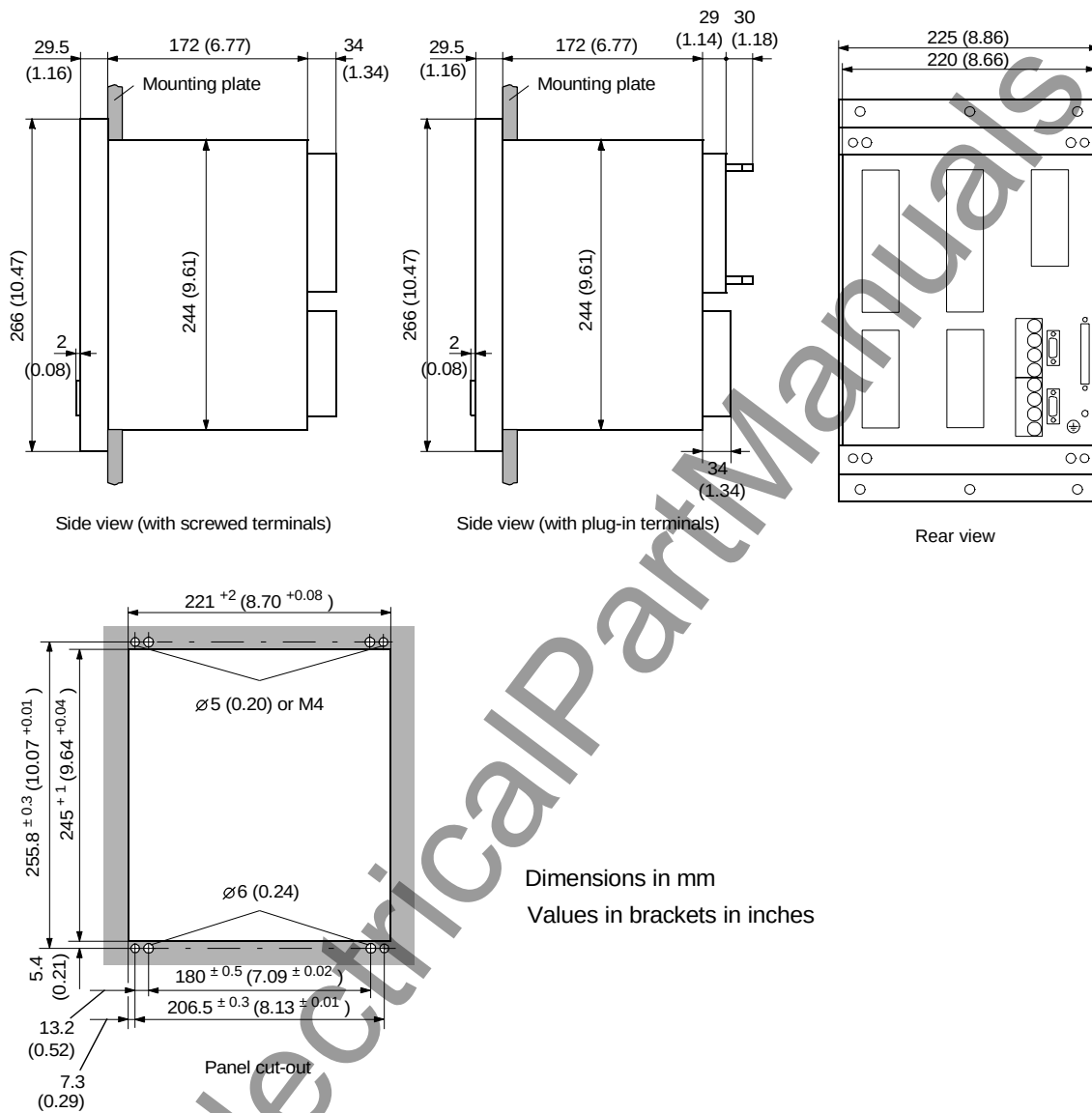
Figure 10-8 Dimensions 7SA6 for panel flush mounting or cubicle installation (size 1\frac{1}{2} x 19")
