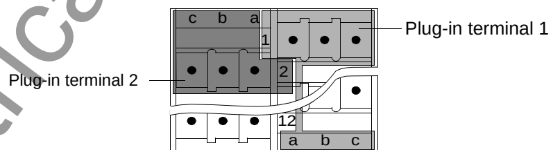
Figure 2-15 Correlation between plug-in terminals and connection numbers/letters
