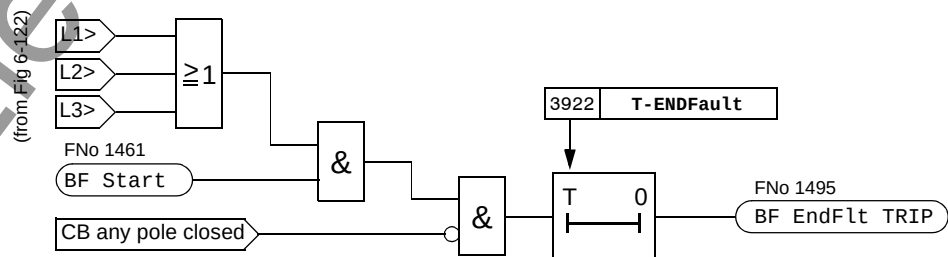
Figure 6-134 Function block diagram of end fault protection
