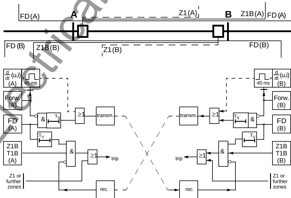
Figure 6-62 Operation scheme of the blocking method
