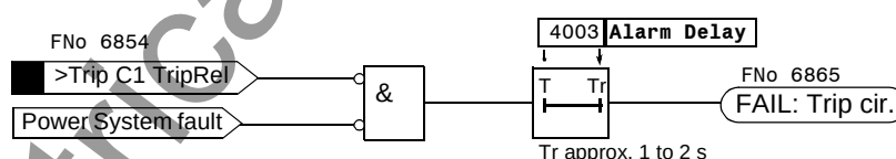
Figure 6-147 Logic diagram of the trip circuit supervision with one binary input
