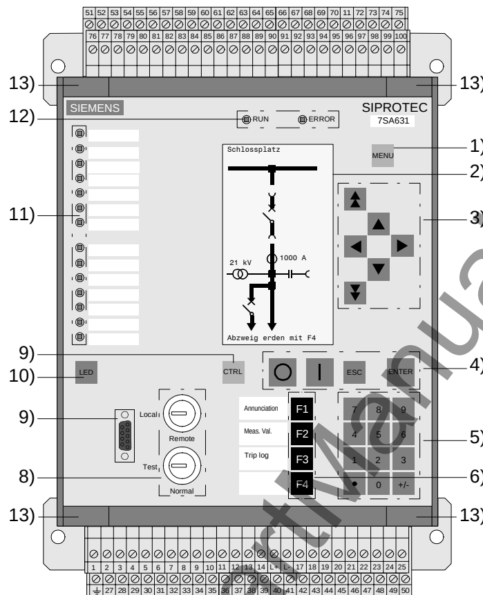
Figure 2-25 Front view of a 7SA63, housing size 1 / 2 , for panel surface mounting without optical communication interfaces
