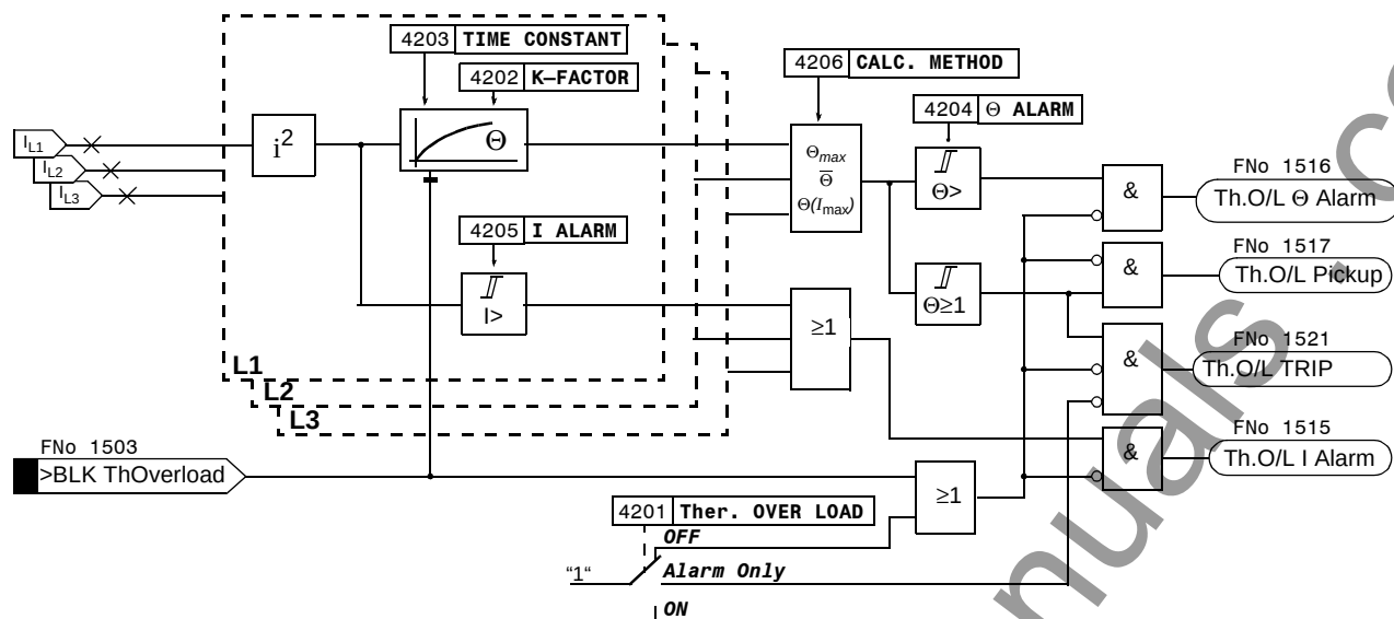
Figure 6-138 Logic diagram of the thermal overload protection
