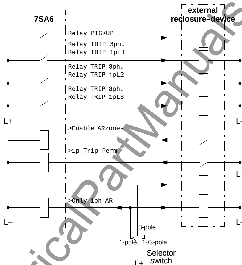
Figure 6-106 Connection example with external reclosure device for 1-/3-pole reclosure with mode selector switch
