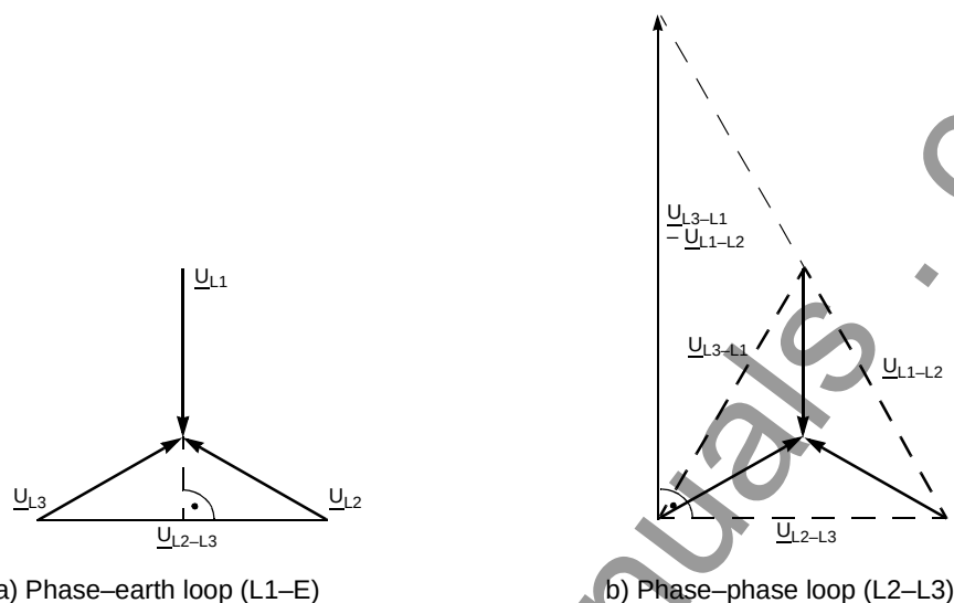
Figure 6-30 Direction determination with quadrature voltages
