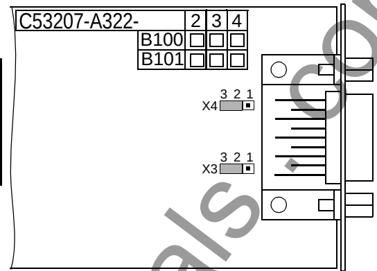
Figure 8-22 Location of jumpers for the configuration of terminating resistors at the interface Profibus
