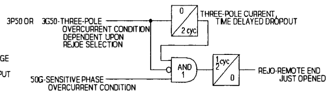
REMOTE-END-JUST-OPENED LOGIC DIAGRAM
