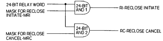
PROGRAMMABLE RECLOSE INITIATE AND CANCEL LOGIC DIAGRAM
