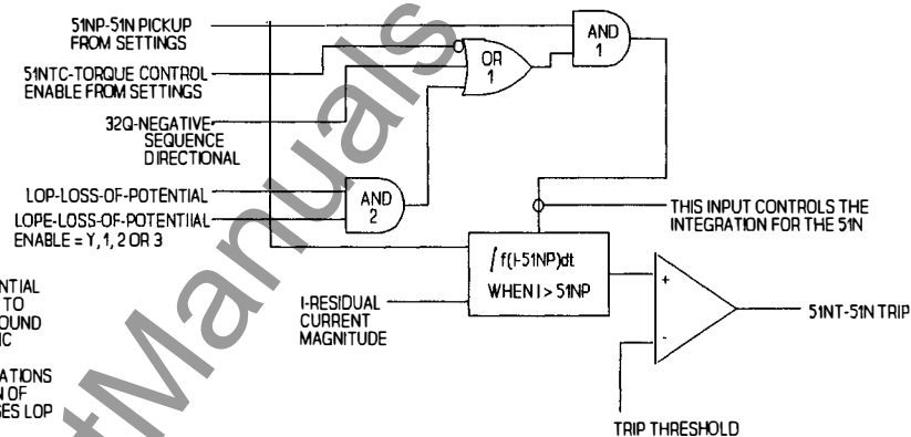
RESIDUAL TIME-OVERCURRENT (51N) LOGIC DIAGRAM
