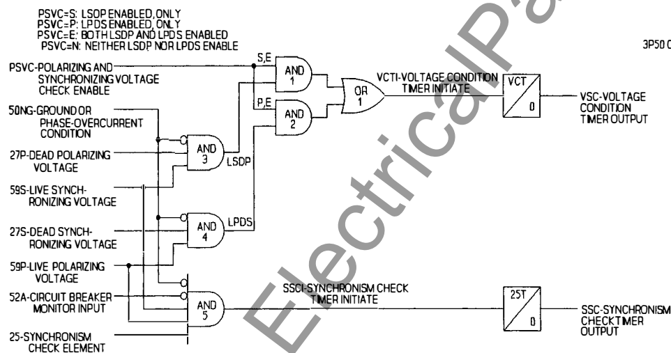
SYNCHRONISM AND VOLTAGE CHECKING LOGIC DIAGRAM
