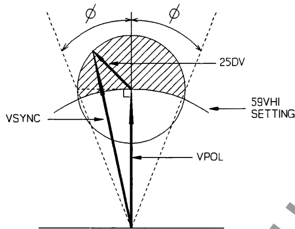
Figure 5.2: Sync-Check Window
