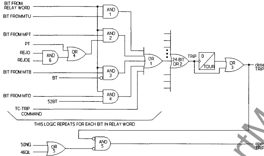
PROGRAMMABLE TRIP LOGIC DIAGRAM
