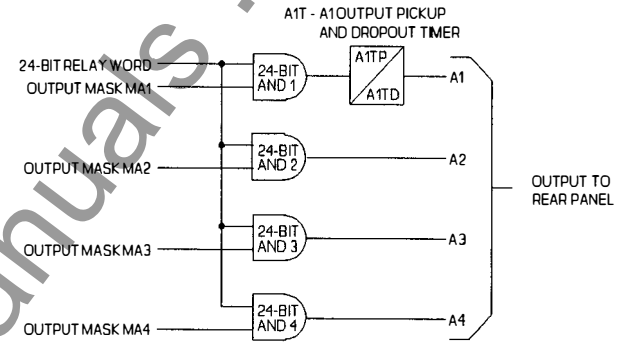
PROGRAMMABLE OUTPUT LOGIC DIAGRAM
