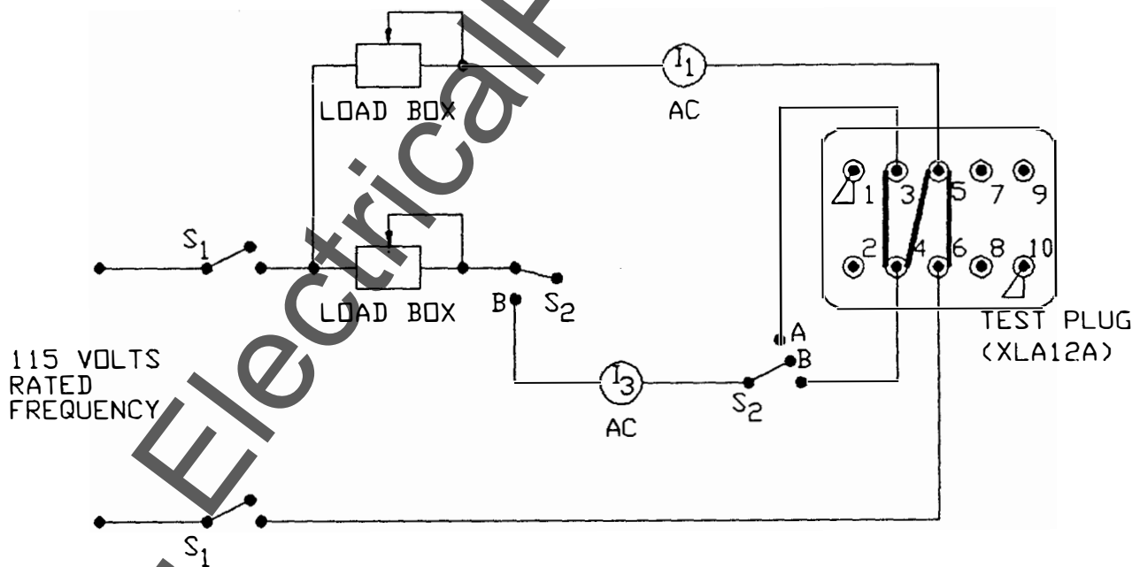
* Figure 10 (0286A3545 [1]) Test Circuit for NBD Relays
