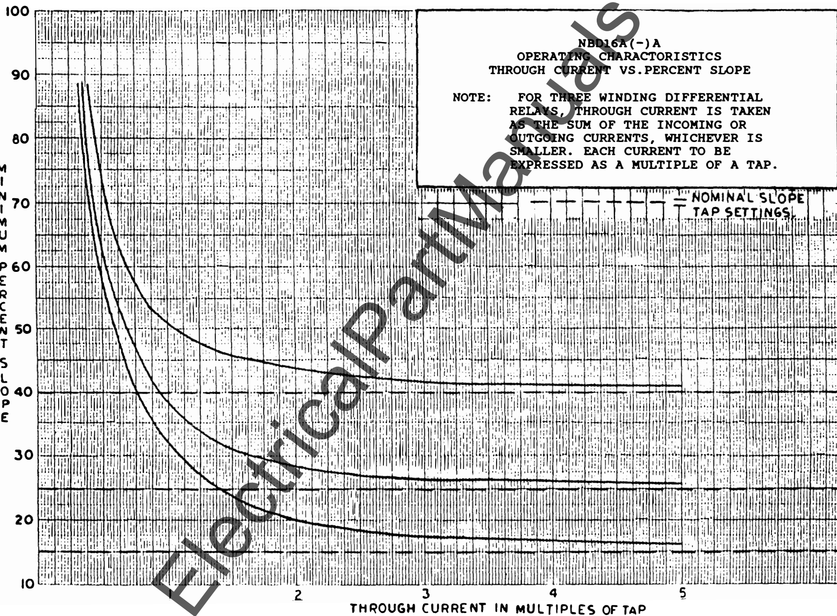
Figure 4 (0285A5495) Operating Characteristics Expanded Curve of Figure 3
