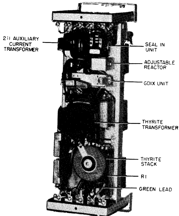
Figure 1B (8029724) CLPG12C Relay Rear View
