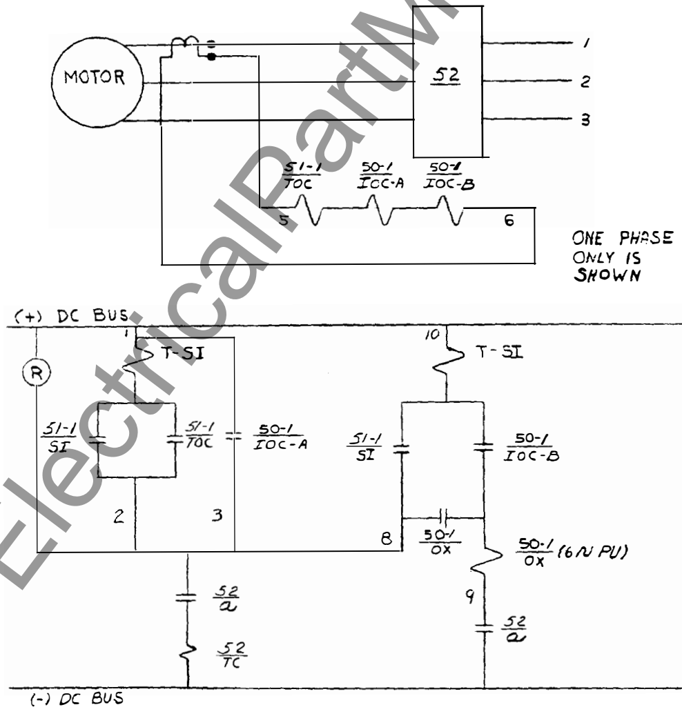
Figure 5 (0207A7826-0) External Connections Diagram for IAC66M Relay
