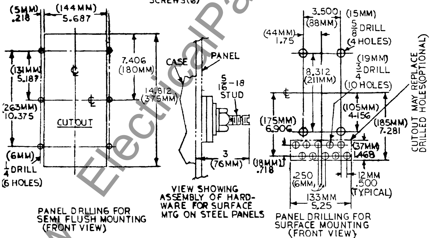
Figure 3 (6209273-3) Outline and Panel Drilling Dimensions for the IAC66M Relay
