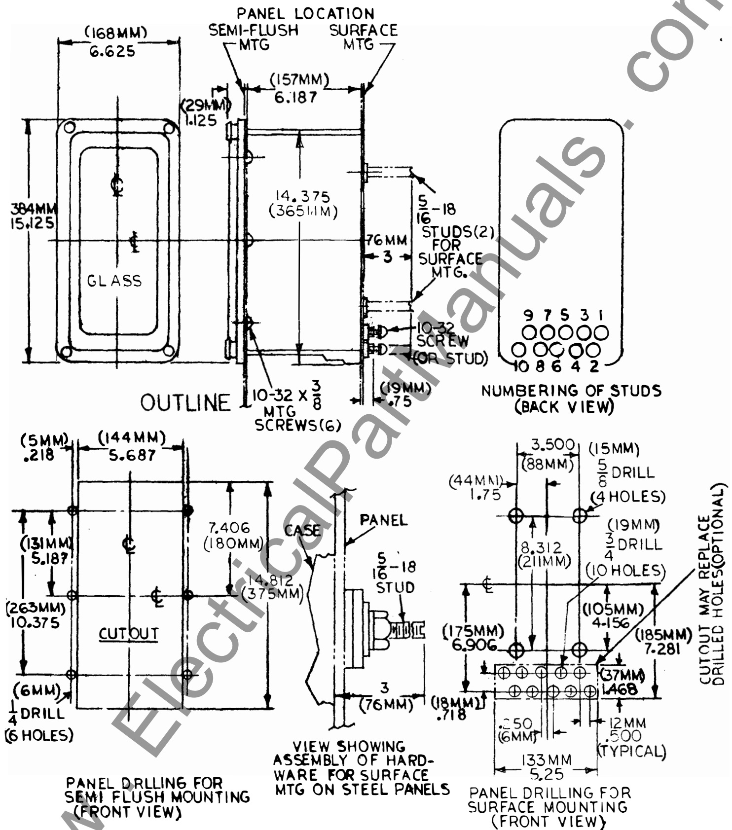
Fig. 22 (K-6209273-3) Outline and Panel Drilling Dimensions for IBC Relays
